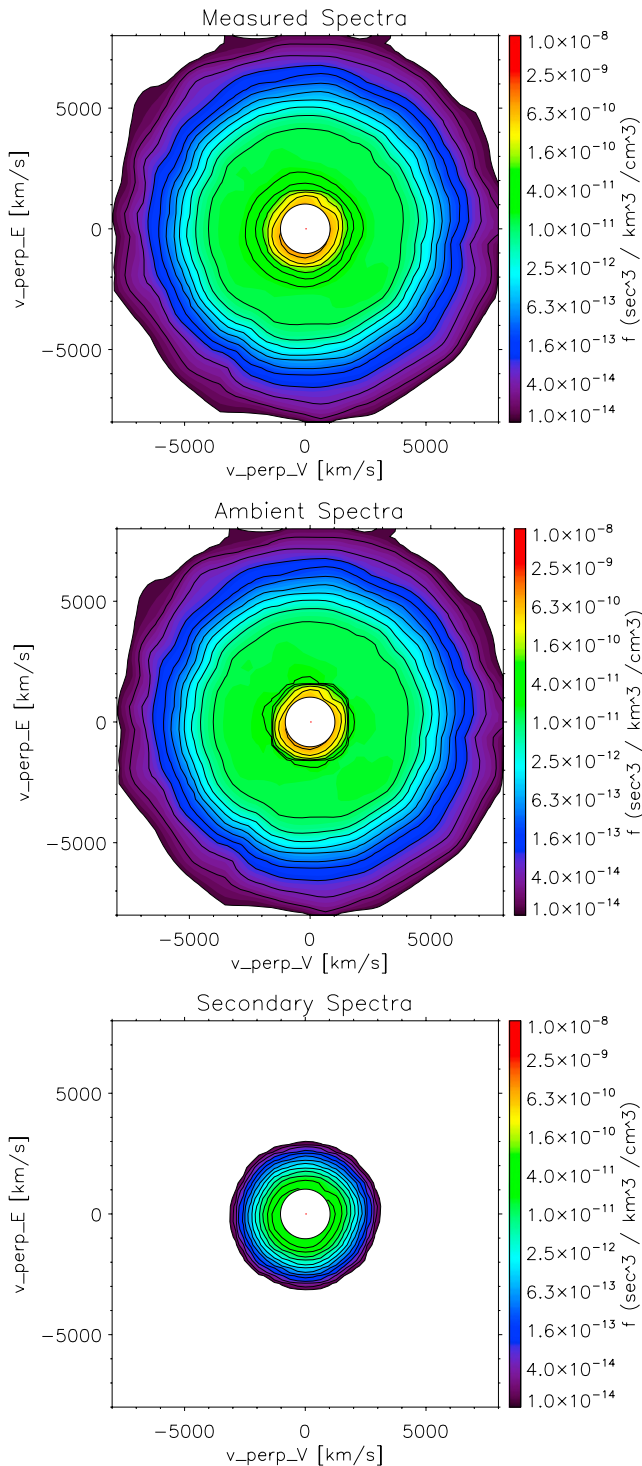
Figure 5. 3-Dimensional spectra decomposed into measured, ambient, and secondary spectra. The axis is oriented so the magnetic field points out of the page. The corrected (ambient) spectra are gyrotropic around the magnetic field, as is expected due to the highly magnetized nature of the electron distribution.
