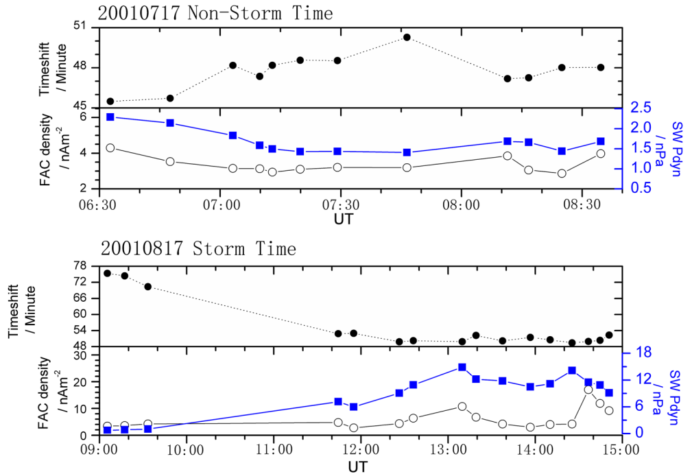
Figure 1. Two examples of the field-aligned current (FAC) cases with their corresponding solar wind dynamic pressure ( SW P_{dyn} ) when the Cluster spacecraft were crossing the PSBL in the magnetotail in non-storm time (the top panel) and storm time (the bottom panel), respectively. The black dotted line denotes the time shift that the interplanetary magnetic field (IMF) from ACE observation influence on the magnetotail, the blue line denotes the solar wind dynamic pressure and the black line denotes the density of FACs.
