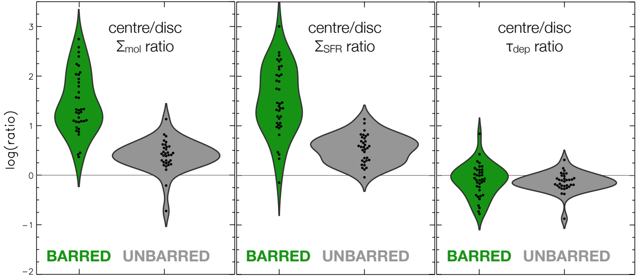
Fig. 9. Violin plots showing the contrast in molecular gas and star formation rate surface density, as well as depletion time, between centres and discs. The sample is split into barred (green) and unbarred galaxies (grey).
