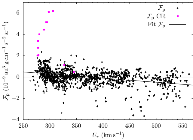
Fig. 4. Dependence of the proton contribution \mathcal{F}_p to the angular-momentum flux on the radial proton bulk speed U_r . We show the measurements of \mathcal{F}_p as points and overplot the linear fit to Eq. (5) as a black line. All measurement points have horizontal and vertical error bars, which are small due to the time-averaging. The fit parameters are given in Table 2. The magenta squares represent the measurements of \mathcal{F}_p during the time of the compression region (CR) on 2020-09-06.
