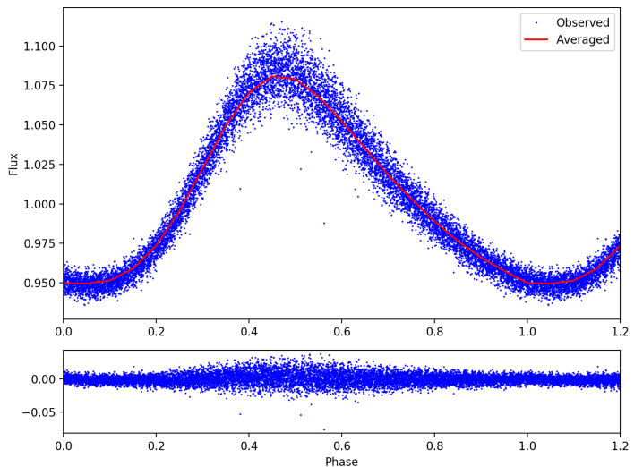
Fig. 1. Phase diagram of TIC 308396022 from TESS data, folded by the frequency, f_1 = 13.20362567\text{d}^{-1} . The obvious light variation of rapid climb and slow descent is typical for a HADS star.
