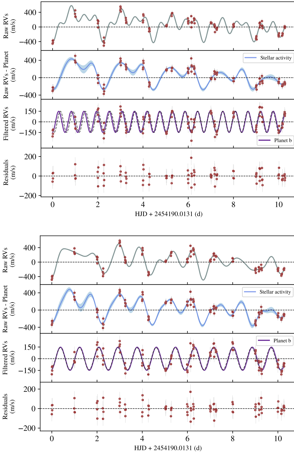
Figure B5. Resulting fits for the GP analysis of data sets #32 (top) and #36 (bottom). Top panel is the total model (grey line) and the observed raw RVs (red points). The second panel is the GP fit with the uncertainty shown by the shadowed area (analytically computed predictive standard deviation of the GP); red points are (raw RVs) – (recovered planet). The third panel is the recovered planet (purple line) on top of the true injected planet (dashed curve). Red points are (raw RVs) – (GP fit). The bottom panel is the residuals, i.e. (raw RVs) – (GP model) – (recovered planet).
