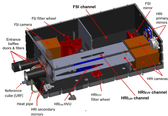
Fig. 21. Schematic of the EUI Optical Bench System showing its three telescopes: the Full Sun Imager (FSI), the High Resolution Imager in Lyman- \alpha (HRI LYA ), and the High Resolution Imager at 17.4 nm (HRI EUV ) (from Rochus et al. 2020).
