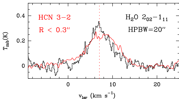
Figure 3. Spectra of the \text{H}_2\text{O } 2_{02} \rightarrow 1_{11} line obtained with the HIFI instrument on board the Herschel Space Observatory towards GV Tau N. For comparison, we have plotted the averaged ALMA spectrum of HCN 3 \rightarrow 2 in a circle of R < 0.3 arcsec around GV Tau N scaled to match the intensity of the \text{H}_2\text{O } 2_{02} \rightarrow 1_{11} line. The systemic velocity, v_{\text{lsr}} = 6.3 \text{ km s}^{-1} , is indicated with the red-dashed line.
