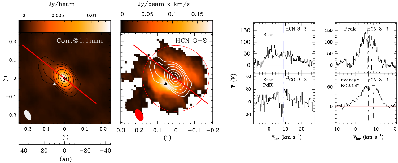
Figure 1. Left: Continuum image at 1.1 mm as observed with ALMA. Levels are 5\sigma , 10\sigma , 20\sigma – 100\sigma by 20\sigma , where \sigma = 0.13 mJy beam -1 . Centre: Zero moment map of the HCN 3→2 line in units of Jy beam -1 × km s -1 . Contour levels are 0.01, 0.025, 0.05, 0.1, 0.15, and 0.175 Jy beam -1 × km/s. The red line indicates the jet direction derived from the 1.1 mm continuum observations ( Jet 1 ), and the circle marks the radius of the gaseous disc, R = 0.18 arcsec. In white, the contours of the 1.1 mm continuum emission. Right: Interferometric spectra of the HCN 3→2 and 13 CO 3→2 lines towards the star position (the black and white crosses in left-hand and centre panels, respectively) as observed with ALMA and PdBI. The HCN 3→2 spectrum at the emission peak in the gaseous disc (the white and black triangles in the left-hand and centre panels) and the averaged HCN 3→2 spectrum in the region R < 0.18 arcsec are shown in the right-hand panel. The intensity scale in the spectra is main beam brightness temperature. Vertical lines mark v_{\text{lsr}} = 6.3 km s -1 and 8.7 km s -1 .
