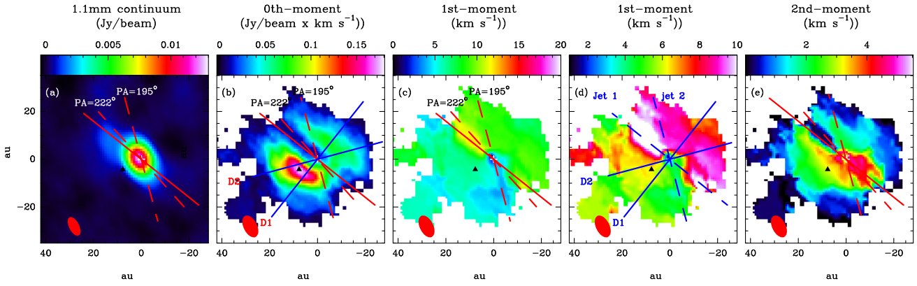
Figure 4. (a) to (d) Continuum image at 1.1 mm and moment maps of the HCN 3→2 emission as observed with ALMA. The dashed lines indicate the direction of the giant Herbig–Haro flow at PA = 222° (Devine et al. 1999) and of the optical jet detected at PA = 195° (Movsessian & Magakian 1999). We also indicate the directions perpendicular to Jet 1 , named D1 , and to Jet 2 , named D2 . Panels (c) and (d) show the same map with different colour scales to highlight the bipolar outflow(s) (c) or the rotation motion (d). The directions Jet 1 , Jet 2 , D1 , and D2 are selected to perform the position–velocity diagrams.
