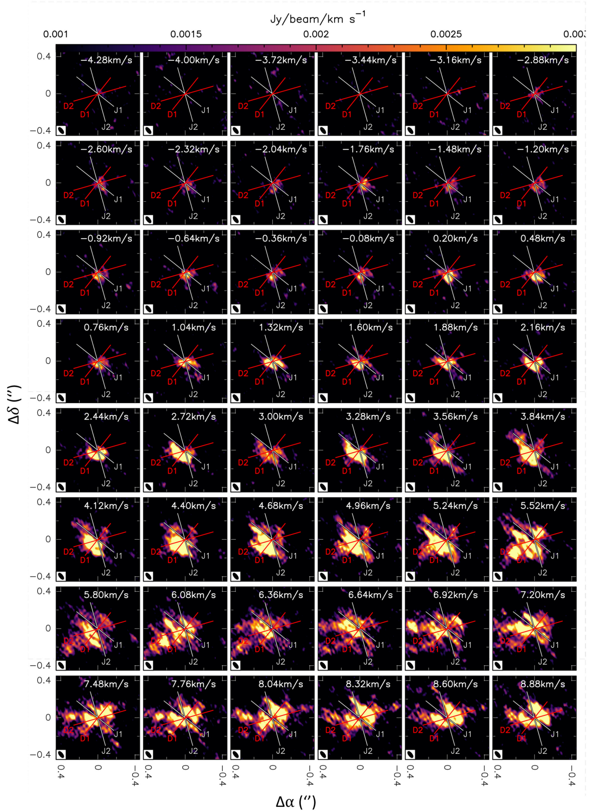
Figure A1. Channel maps of the HCN 3→2 line as observed with ALMA. The solid lines indicate the directions of Jet 1 , Jet 2 , D1 , and D2 .
