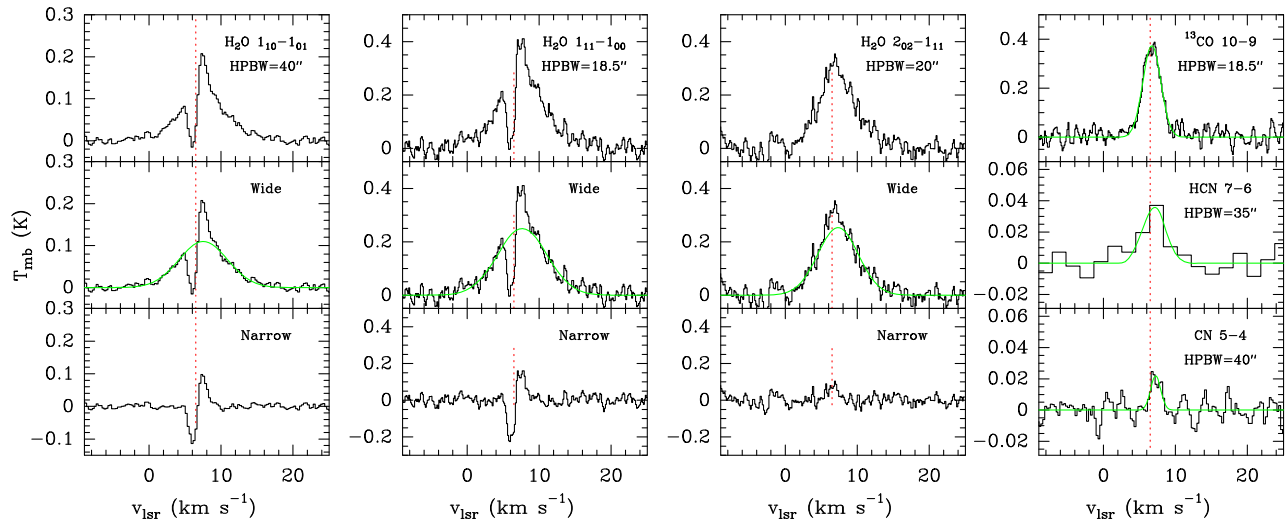
Figure 2. Spectra of the ^{13}\text{CO } 10 \rightarrow 9 , \text{H}_2\text{O } 1_{11} \rightarrow 0_{00} , 1_{10} \rightarrow 1_{01} , and 2_{02} \rightarrow 1_{11} lines obtained with the HIFI instrument on board the Herschel Space Observatory towards GV Tau N. The systemic velocity, v_{\text{lsr}} = 6.3 \text{ km s}^{-1} , is indicated with the red-dashed line.
