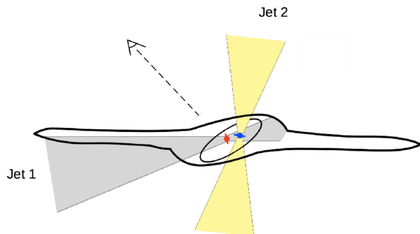
Figure 6. Sketch of the geometry proposed for GV Tau N to explain ALMA spectroscopic observations.
