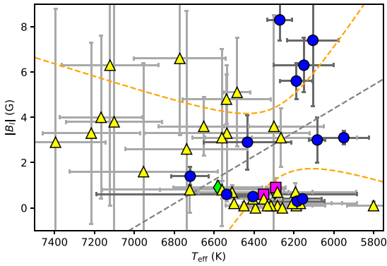
Figure 2. |B_l| versus T_{\text{eff}} for 50 of our stars (excluding \beta CrB with a fossil field, and excluding 4 non-detections, \alpha Hyl, \alpha Crv, \eta Lep, and \gamma Cet, with large B_l and large uncertainties). The blue circles indicate definite magnetic detection on an F-star, yellow triangle indicates no detection, a magenta square is a marginal detection, while a green diamond is a definite detection but uncertain if detection is from the F-star or a companion. The dashed grey trend line and orange 95 per cent confidence intervals are shown for our 14 stars with magnetic detection, excluding \beta CrB. No significant trend observed between T_{\text{eff}} versus |B_l| .
