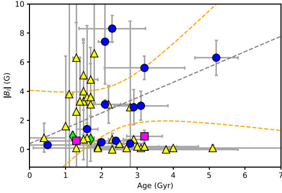
Figure 6. |B_l| versus stellar age for 50 of our stars, excluding \beta CrB (fossil field) and excluding 4 stars ( \alpha Hyi, \beta TrA, \theta UMa, and \gamma Cet) with no detection and large B_l with large uncertainties. The dashed grey trend line and orange 95 per cent confidence intervals shown for our 14 stars with a magnetic detection excluding \beta CrB. No significant trend observed. The symbols are the same as Fig. 2.
