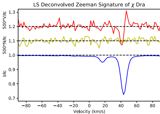
Figure B12. LSD profile (single spectra) for \chi Dra (F7V+K1V) on 2015 April 24. The plot is described in Fig. B1.
