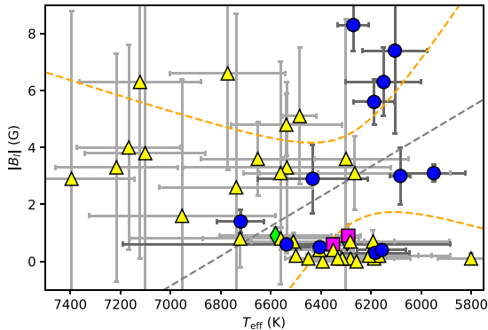
Figure 2. |B_l| versus T_{\text{eff}} for 50 of our stars (excluding \beta CrB with a fossil field, and excluding 4 non-detections, \alpha Hyl, \alpha Crv, \eta Lep, and \gamma Cet, with large B_l and large uncertainties). The blue circles indicate definite magnetic detection on an F-star, yellow triangle indicates no detection, a magenta square is a marginal detection, while a green diamond is a definite detection but uncertain if detection is from the F-star or a companion. The dashed grey trend line and orange 95 per cent confidence intervals are shown for our 14 stars with magnetic detection, excluding \beta CrB. No significant trend observed between T_{\text{eff}} versus |B_l| .
