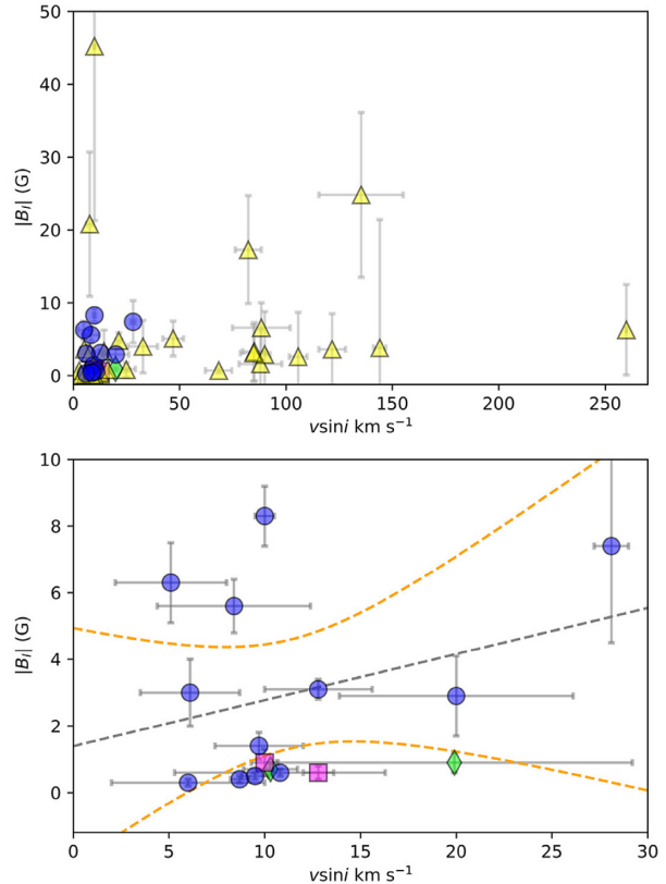
Figure 5. Top Figure. |B_l| versus v \sin i for 54 of our stars (excluding \beta CrB with a fossil field). Bottom figure. v \sin i versus |B_l| for 14 of our stars with a magnetic detection except \beta CrB. The dashed grey trend line and orange 95 per cent confidence intervals shown. No significant trend observed. The symbols are the same as Fig. 2.
