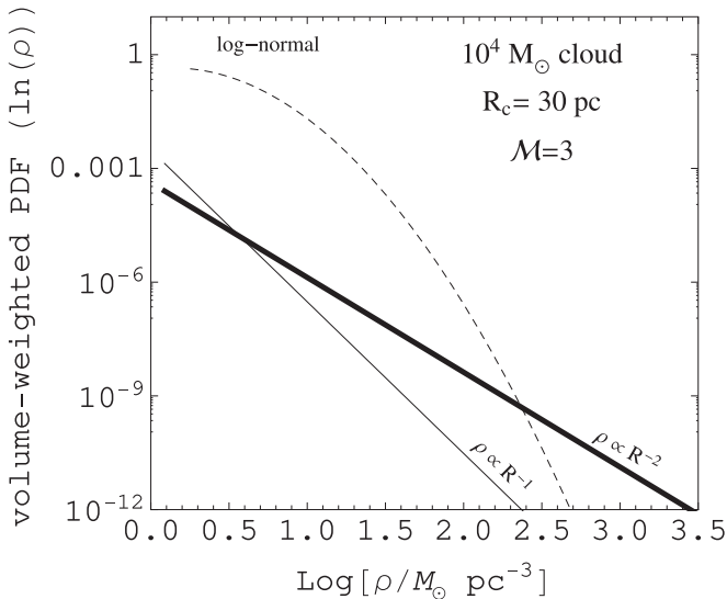
Figure 3. Example volume-weighted log-density PDFs for a 10^4 M_{\odot} cloud with radius R_c = 30 pc. The thick solid line shows the PDF for our nominal case of a PL density distribution \rho \propto R^{-2} . The thin solid line assumes a shallower density profile \rho \propto R^{-1} associated with lower density gas fractions. The dashed line represents a lognormal PDF with density variance set by the characteristics of driven turbulence, assuming solenoidal driving (Federrath et al. 2010) and a conservative Mach number \mathcal{M} = 3 .
