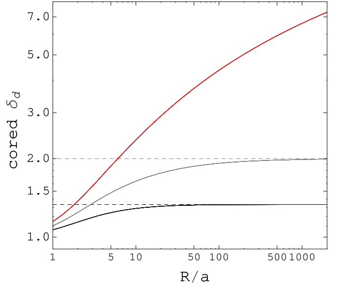
Figure 10. Behavior of the factor \delta_d for the cored PL density profiles in Equation (29) with index k = 1 (black), k = 1.5 (gray), and k = 2 (red) as a function of the ratio of the cloud size R_c to the core radius a . Dashed black and gray horizontal lines show the value of \delta_{d,\text{PL}} for a pure PL (which is finite only for k < 2 ).
