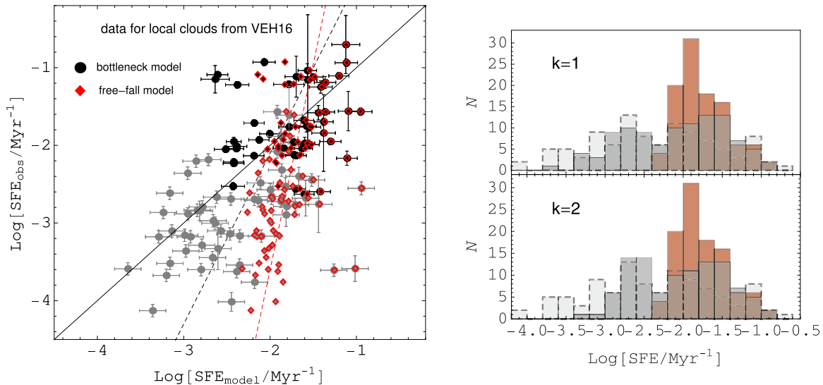
Figure 7. (Left) Comparison between the observed SFE_{\text{obs}} and the SFE_{\text{model}} predicted by either the bottleneck model (black and gray circles) or the free-fall model (red-outlined diamonds). Measurements from two density regimes within the clouds are shown (low: gray and high: black). Error bars are shown only on the bottleneck model predictions and reflect propagated uncertainties on either the measured mass and SFR (vertical) or the cloud mass and size (horizontal). The black line indicates equality. The gray (red) dashed line shows the best-fit relation to all points predicted by the bottleneck (free-fall) model. (Right) Histograms of observed and predicted SFE in local clouds. In both panels, observed SFEs are shown in light gray with a black dashed boundary, and the predictions of the free-fall model are shown in red. Two predictions of the bottleneck collapse model are highlighted (dark gray) assuming two different PL indices: k = 1 (top) and k = 2 (bottom).
