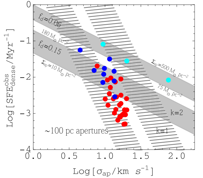
Figure 9. Observed variation in the dense gas SFE, \text{SFE}_{\text{dense}} , with gas velocity dispersion \sigma_{\text{ap}} measured in \sim 100 pc apertures throughout NGC 3627 (cyan; probing out to R_{\text{gal}} \sim 3 kpc), M31 (blue; out to R_{\text{gal}} \sim 15 kpc), and M51 (red; out to R_{\text{gal}} \sim 3 kpc; Querejeta et al. 2019, and references therein). Gas kinematics on this scale provide a measure of motions in the galactic potential. Four bands show the decrease in SFE with \sigma_{\text{ap}} predicted by Equation (38) assuming either k = 2 (solid gray) or k = 1 (hashed gray), at two different (fixed) levels of the dense gas fraction f_d and a range in gas surface density on 100 pc scales, \Sigma_{\text{H}_2, \text{ap}} = 10 - 180 M_\odot \text{pc}^{-2} (bottom, left) and \Sigma_{\text{H}_2, \text{ap}} = 75 - 500 M_\odot \text{pc}^{-2} (top, right). The lower/left trend for each k is intended to span the observed ranges in M33 and M51 (Querejeta et al. 2019) while the upper/right trend is meant to match observations of the dense gas in NGC 3627 (Murphy et al. 2015) and assumes the relevant aperture size of 300 pc.
