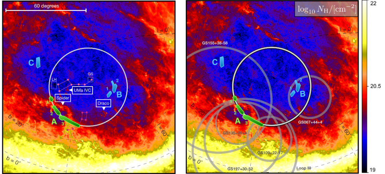
Fig. 2. Stereographic projection of the total gas column density, N_H , derived from Planck observations of dust thermal emission (color scale). The locations of feature A, which defines the UMa arc, and features B and C are denoted. The UMa circle is shown in light gray. Left panel: positions of the UMa IVC, Draco, and Spider clouds, along with the Ursa Major and Minor constellations (in pink). Two of the lowest column density windows in the Galaxy (Lockman Hole (LH) and Groth strip (GS)) are shown. Right panel: positions of known arches and loops, in dark gray. The transition between blue and red on the false-color intensity scale corresponds to N_H = 10^{20} \text{ cm}^{-2} .
