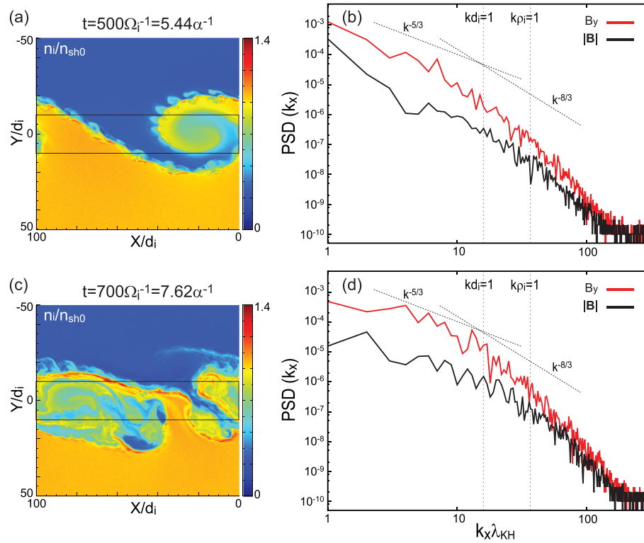
Figure 4. (a, c) Density profiles in the XY plane at t = 500\Omega_i^{-1} and t = 700\Omega_i^{-1} from a 3-D kinetic simulation of the KHI (Nakamura, 2020, where \Omega_i = eB_0/m_i and \alpha = V_0/\lambda_{KHI} , the total velocity jump across the initial shear layer divided by the most unstable KHI wavelength. The X axis is roughly antiparallel to the initial magnetosheath flow, and the Y axis is normal to the initial velocity shear and current layers. The average wave number spectra of the magnetic energy density in normalized unit (b, d) are computed by use of the simulation data in the domain enclosed by the black boxes.
