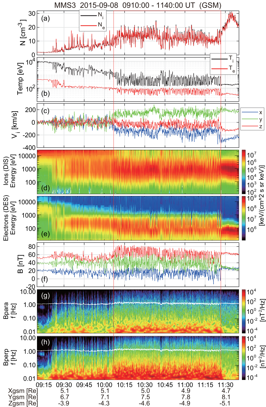
Figure 1. MMS3 fast survey-mode observations of Kelvin-Helmholtz (KH) waves at the postnoon magnetopause on 8 September 2015 for the interval 0910–1140 UT. (a) Ion and electron densities, (b) ion and electron temperatures assuming isotropic velocity distributions, (c) three GSM components of the ion velocity, (d, e) energy versus time spectrograms of omnidirectional ions and electrons from the dual ion spectrometer (DIS) and dual electron spectrometer (DES) parts, respectively, of the Fast Plasma Investigation (FPI) instrument suite, (f) GSM components of the magnetic field, and (g, h) wavelet power spectra of the magnetic field fluctuations parallel and perpendicular to the mean field, with the proton cyclotron frequency marked by the white curve. The KH-active interval 1007–1127 UT between the two vertical red lines is used to derive turbulent spectra in Figure 2.
