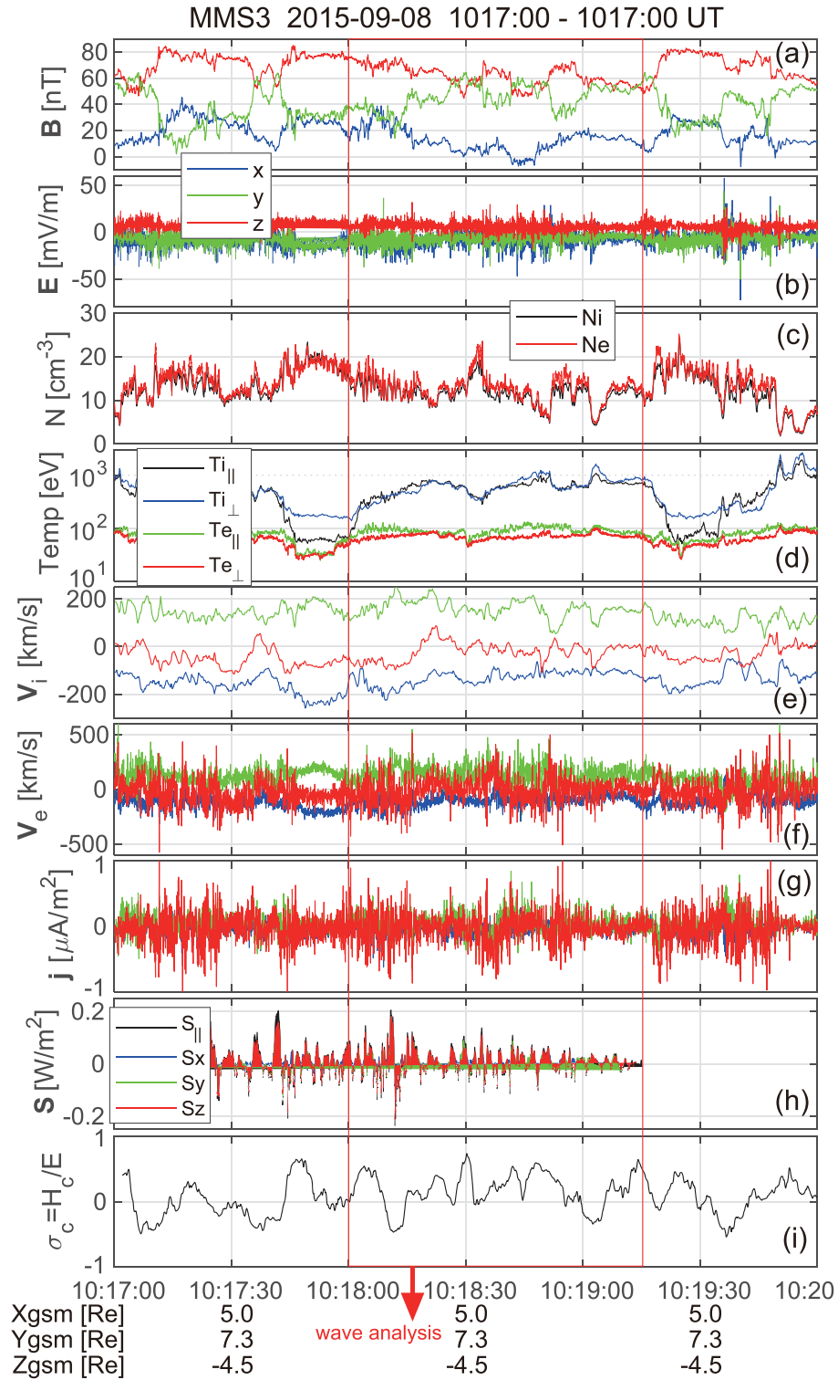
Figure 5. An example of the KH-active boundary layer intervals on 8 September 2015 used for the k -vector analysis. (a, b) GSM components of the magnetic and electric fields, (c) ion and electron densities, (d) ion and electron temperatures in both the parallel and perpendicular directions, (e, f) ion and electron velocities, and (g) current density based on the FPI measurements, (h) parallel and GSM components of Poynting flux, \mathbf{S} = \delta \mathbf{E} \times \delta \mathbf{B} / \mu_0 , and (i) normalized ion cross helicities, \sigma_c = H_c / E , the ratio between the cross helicity and average energy (see text for details), all from the MMS3 spacecraft. The magnetosphere-side interval enclosed by the red box is used in the k -vector analysis.
