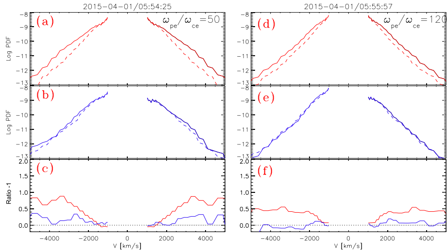
Figure 4. Electron distribution function transverse (red lines) and parallel (blue lines) to the background local magnetic field direction, at times corresponding to maxima (solid lines) and minima (dashed lines) in the magnetic field magnitude. Panels (c) and (f) present the ratio of maximum to minimum (solid divided by dashed) distribution function values for the transverse (red) and parallel (blue) cases, minus 1. The left column presents the data when f_{pe}/f_{ce} \sim 50 ; the right column when f_{pe}/f_{ce} \sim 120 .
