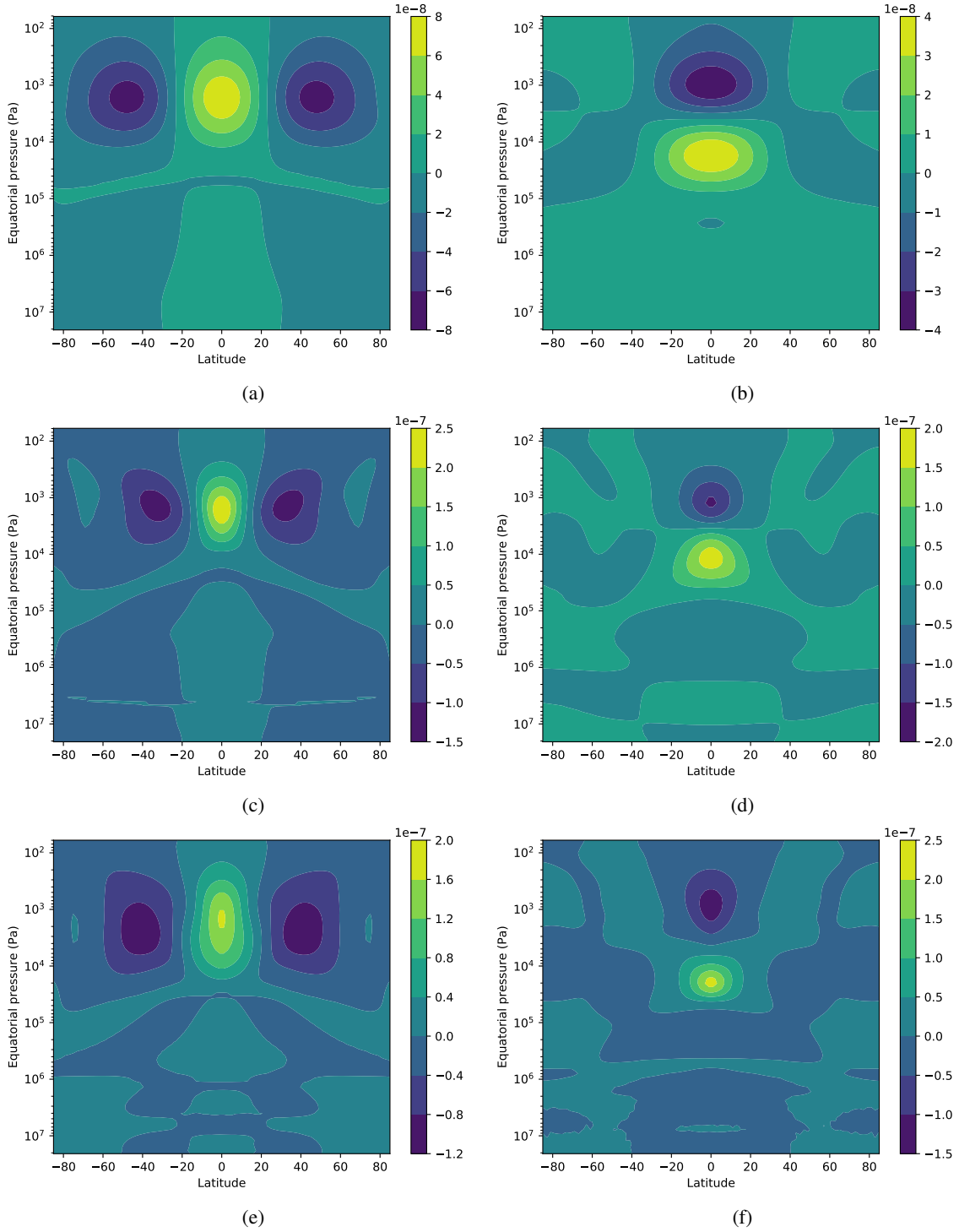
Fig. 8. Left column: meridional eddy accelerations as a function of pressure and latitude in the \Delta T_{\text{eq,top}} = 100 K case after 1 (top), 5 (middle) and 20 (bottom) days. Right column: same for vertical eddy acceleration. Units in \text{kg m}^{-2} \text{s}^{-2} .
