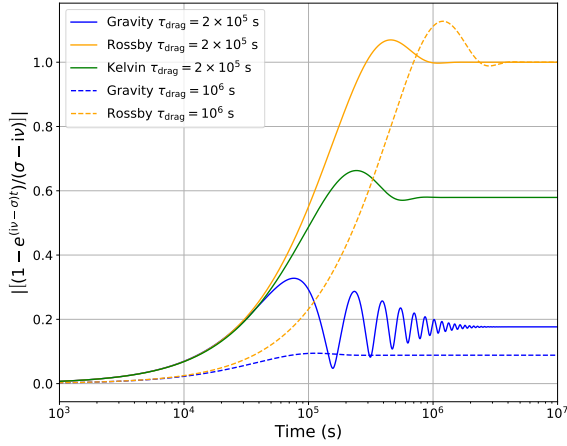
Fig. 5. Modulus of (1 - e^{i(v-\sigma)t})/(\sigma - i\nu) normalized by the final value for the Rossby wave as a function of time for gravity, Rossby and Kelvin waves with the numerical frequencies and decay rates obtained with ECLIPS3D. \tau_{\text{rad}} follows the prescription of Iro et al. (2005) whereas \tau_{\text{drag}} is set constant either to 2 \times 10^5 s (plain lines) or 10^6 s (dashed lines).
