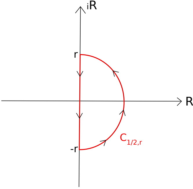
Fig. B.1. Graphical representation of the C_{1/2,r} contour, encompassing the complex numbers with positive real part when r \rightarrow \infty .
