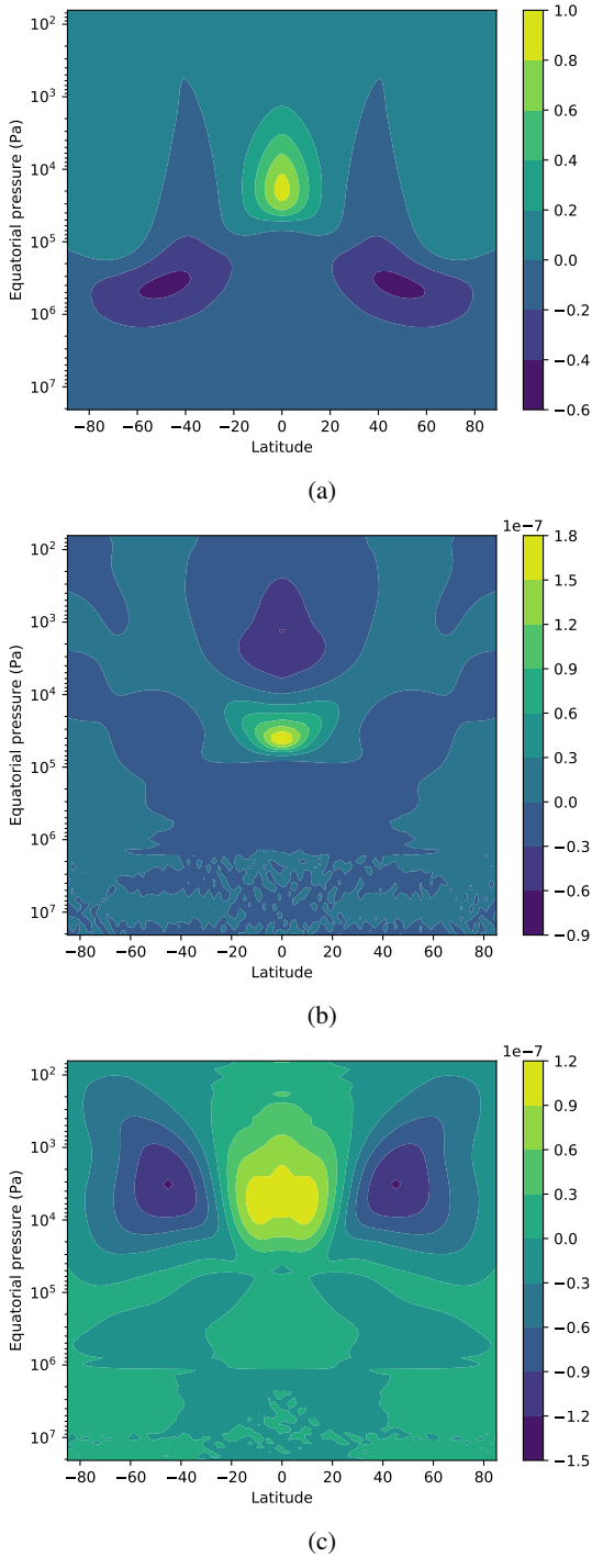
Fig. 7. (a) (\bar{\rho} \bar{u}) ( \text{kg m}^{-2} \text{s}^{-1} ) as a function of pressure and latitude after 50 days of simulation with \Delta T_{\text{eq,top}} = 100 \text{ K} . (b) Vertical eddy acceleration ( \text{kg m}^{-2} \text{s}^{-2} ) for the same simulation. (c) Meridional eddy acceleration ( \text{kg m}^{-2} \text{s}^{-2} ) for the same simulation.
