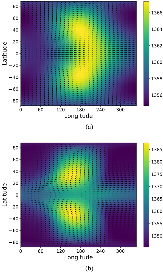
Fig. 1. Temperature (color scale in K) and horizontal wind (arrows) as a function of longitude ( x axis) and latitude ( y axis) at the 40 mbar pressure level of the linear steady state (denominated MG circulation) obtained using ECLIPS3D (Debras et al. 2019) with heating function, drag and radiative timescales following the definitions of Komacek & Showman (2016): (a) \Delta T_{\text{eq,top}} = 100 K, \tau_{\text{drag,top}} = 10^5 s and \tau_{\text{rad,top}} = 10^5 s. The maximum speed at this pressure range is 10 m s ^{-1} . (b) \Delta T_{\text{eq,top}} = 100 K, \tau_{\text{drag,top}} = 10^6 s and \tau_{\text{rad,top}} = 10^4 s. The maximum speed at this pressure range is 100 m s ^{-1} . Note that the maximum speed has been multiplied by ten as the drag timescale has been multiplied by ten.
