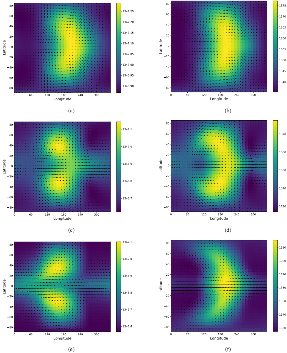
Fig. D.1. Temperature (colors) and winds at a height corresponding to 80 mbar pressure at t = 0 . \tau_{\text{drag}} = 10^6 s and \tau_{\text{rad}} follow the prescription of Iro et al. (2005) for all simulations. The left column has \Delta T_{\text{eq,top}} = 1 K, while the right column has \Delta T_{\text{eq,top}} = 100 K. Finally, the top panel shows the atmosphere after one day of evolution, middle panel after three days, and bottom panel after 50 days. Maximum speeds are (a) 1 \text{ m s}^{-1} ; (b) 100 \text{ m s}^{-1} ; (c) 2 \text{ m s}^{-1} ; (d) 300 \text{ m s}^{-1} ; (e) 5 \text{ m s}^{-1} and (f) 1000 \text{ m s}^{-1} .
