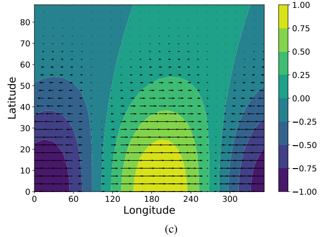
Fig. C.2. Temperature (colors) and winds (arrows), both in arbitrary unit, as a function of longitude and latitude for the shallow water solutions of Eqs. (40) and (A.7) considering \tau_{\text{rad}} = 2.8 and \tau_{\text{drag}} = 28 . Presenting (a) westward propagating gravity wave; (b) Rossby wave; and (c) Kelvin wave.
