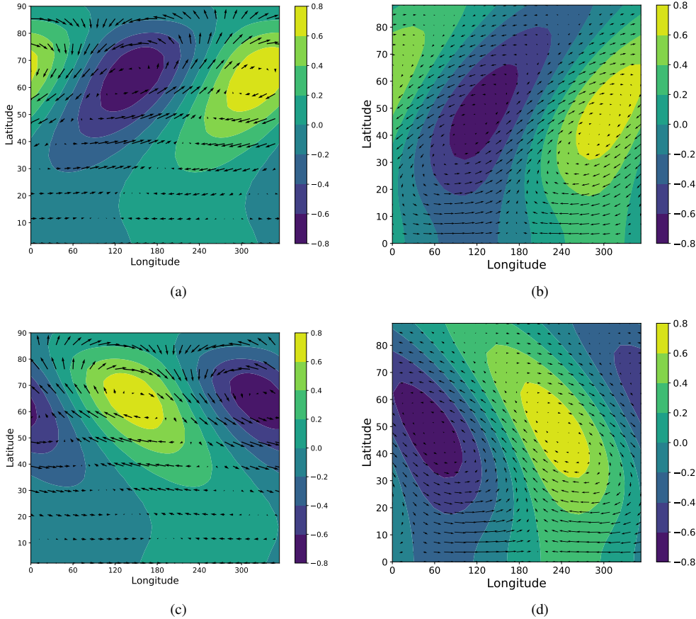
Fig. 4. Pressure perturbations (color scale) and winds (arrows) as a function of longitude and latitude for four Rossby waves for an axisymmetric hot Jupiter atmosphere at rest. Units are arbitrary. The values of the drag and radiative timescales are described in Sect. 4.2. Left column: results from ECLIPS3D 3D spherical coordinate calculations and right column: for the analytical results to the equation developed in Appendix A. For the top row , the drag is dominant, and the bottom row radiation is dominant. We note that as the initial state is at rest and axisymmetric, there is an uncontrolled phase in longitude, meaning the longitudinal location is arbitrary.
