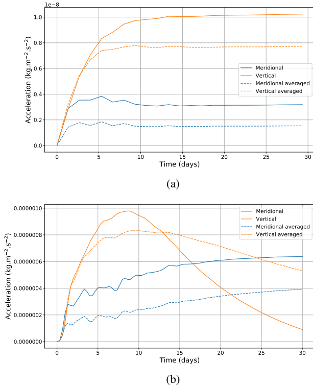
Fig. 9. Eddy accelerations at the equator at the 80 mbar pressure level (plain lines) or averaged from 40 mbar to 0.4 bar (dashed lines) as a function of time for (a): \Delta T_{\text{eq,top}} = 1 \text{ K} , (b): \Delta T_{\text{eq,top}} = 100 \text{ K} .
