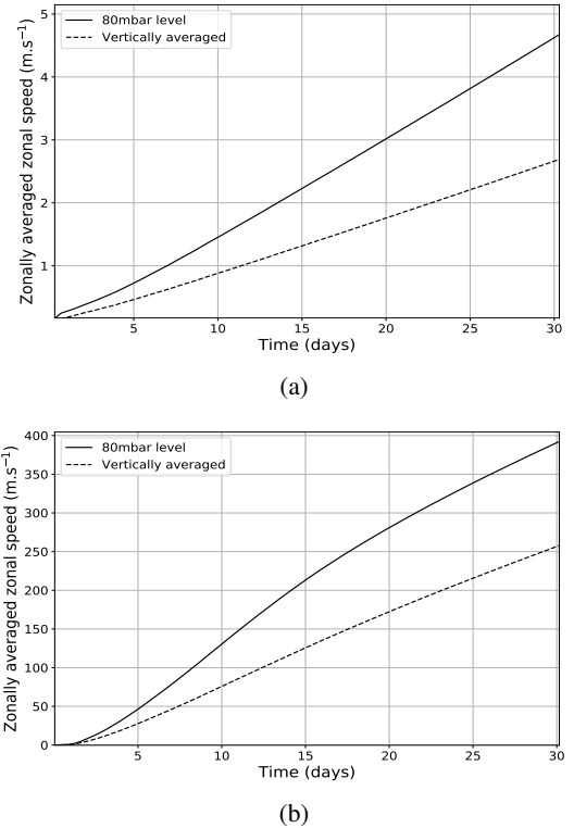
Fig. 10. Zonally-averaged zonal speed at the 80 mbar pressure level (plain lines) or averaged from 40 mbar to 0.4 bar (dashed lines) as a function of time for (a): \Delta T_{\text{eq,top}} = 1 \text{ K} , (b): \Delta T_{\text{eq,top}} = 100 \text{ K} .
