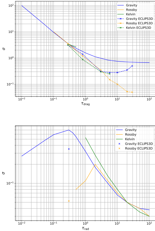
Fig. 3. Typical decay rate \sigma for gravity and Rossby and Kelvin waves as a function of (top) \tau_{\text{drag}} for \tau_{\text{rad}} = 0.3 and (bottom) \tau_{\text{rad}} for \tau_{\text{drag}} = 20 . The lines are values obtained using Eqs. (40), (50) while crosses are results from seven ECLIPS3D calculations. As \tau_{\text{rad}} is not constant with depth in the ECLIPS3D results, we have chosen to use an arbitrary value of \tau_{\text{rad}} = 0.3 for comparison. However, when \tau_{\text{drag}} increases the location where the wave exhibits its maximum perturbation, it moves to higher pressures which should correspond to an increase in the equivalent \tau_{\text{rad}} . For the Rossby waves, the low \tau_{\text{drag}} limit has not been studied numerically as it is irrelevant for superrotation. Kelvin waves of comparable height with Rossby and gravity waves are only clearly identified in four ECLIPS3D calculations.
