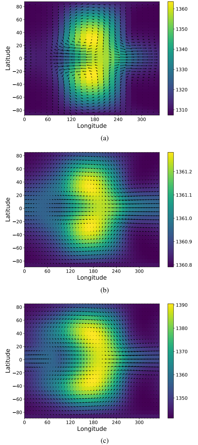
Fig. 6. Temperature (color) and winds (arrows) as a function of longitude and latitude for (a) linear steady state calculated with ECLIPS3D with \Delta T_{\text{eq,top}} = 100 K, \tau_{\text{drag}} = 2 \times 10^5 s and \tau_{\text{rad}} following Iro et al. (2005) . Maximum speed is 400 m s ^{-1} (b): 3D GCM result at the 80 mbar level after 10 days of simulation, with \Delta T_{\text{eq,top}} = 1 K and the radiative timescale of Iro et al. (2005) . The maximum speed is 2.5 m s ^{-1} ; (c): 3D GCM result at the 80 mbar level after 10 days of simulation, with \Delta T_{\text{eq,top}} = 100 K and the radiative timescale of Iro et al. (2005) . The maximum speed is 350 m s ^{-1}
