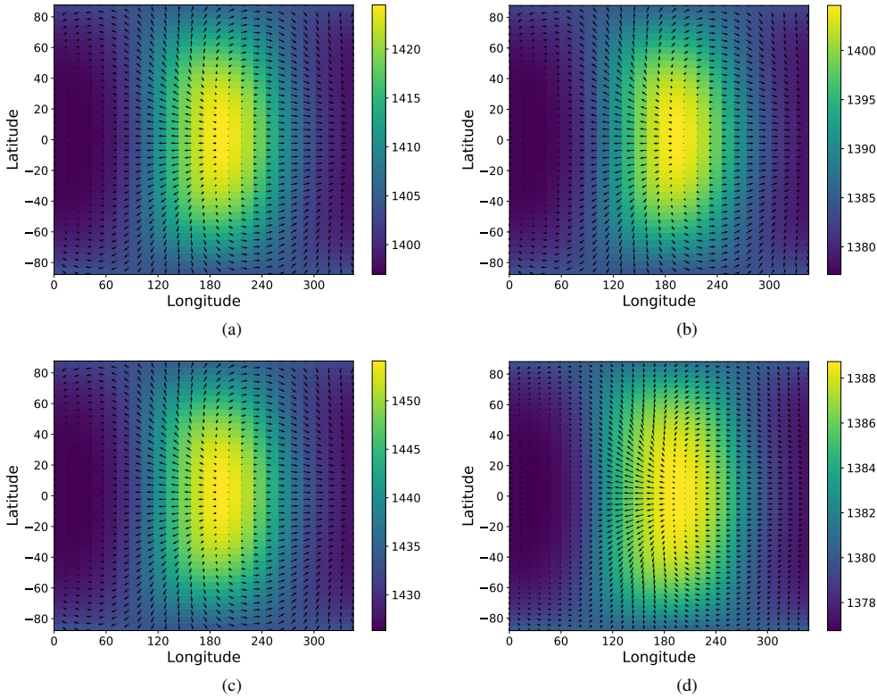
Fig. 2. Temperature (color scale in K) and winds (arrows) as a function of longitude and latitude with different heating functions, with drag and radiative timescales defined as in Komacek & Showman (2016) with non-dimensional values of 1 (almost half an Earth day). (a–c): the initial pressure at this height is 50 mbar which corresponds to an initial temperature of 1326 K and the forcing is \Delta T_{\text{eq,top}} = 50 K. (d): the initial pressure is 40 mbar and initial temperature 1322 K. (a): heating as in Komacek & Showman (2016) (b): same as in Komacek & Showman (2016) but with a cooling at the night side three times more efficient than the heating on the day side. (c): same as in Komacek & Showman (2016) with no cooling at the night side. (d): heating rate extracted from the full radiative transfer calculations of the GCM (divided by ten to obtain comparable values).
