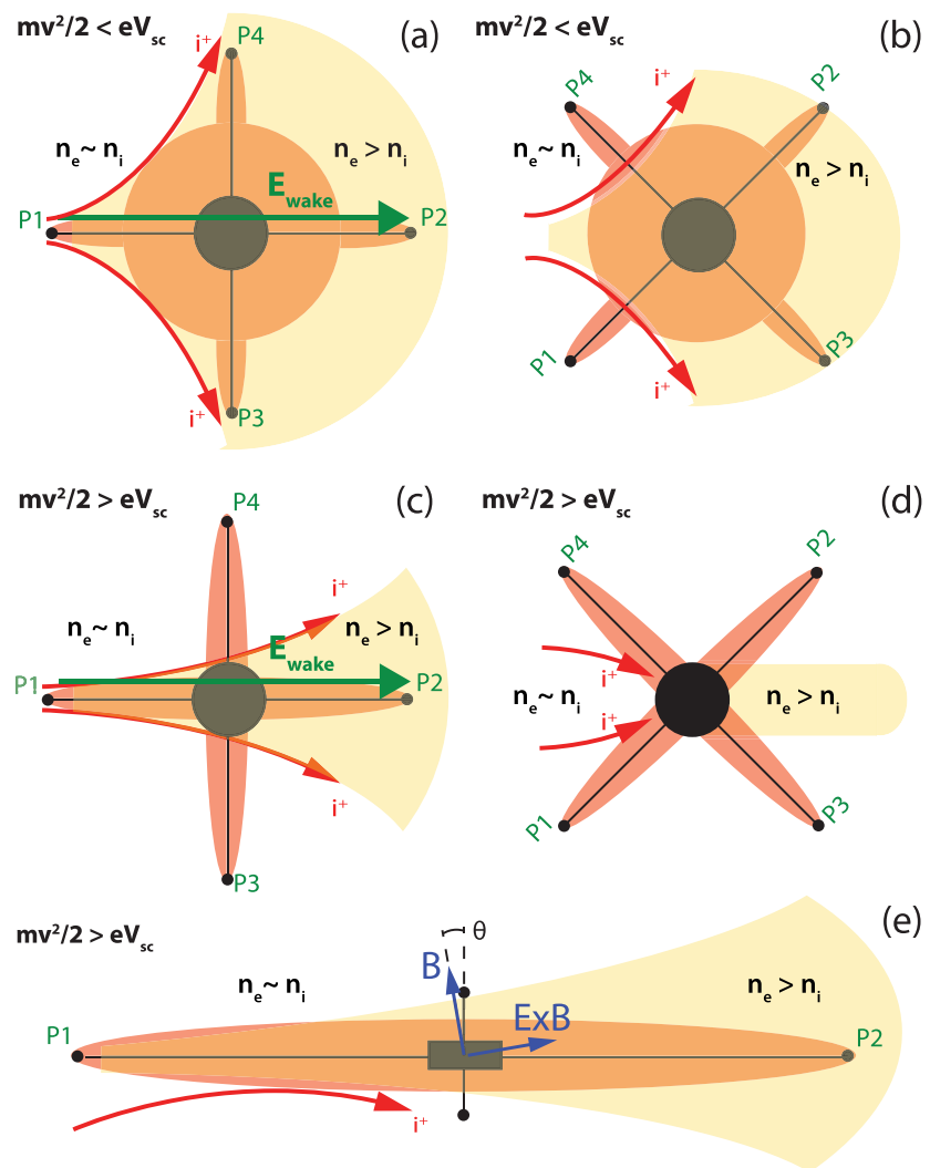
Figure 6. Sketches of the potential structure and ion wake formed around Magnetospheric MultiScale spacecraft. Spacecraft body and wake size are not to scale. (a) Cold ion deflection by the spacecraft body and spin-plane booms potential structure (red-shadowed region), case mv_{ic}^2/2 < q_{ic}V_{sc} . An enhanced ion wake is formed (yellow-shadowed region). (b) Same as (a) without alignment between the ion beam and electric field booms, a smaller ion wake (yellow-shadowed region) is formed than for case (a), owing to the spacecraft body potential structure. (c) Cold ion deflection by the spacecraft potential structure (red-shadowed region), case mv_{ic}^2/2 > q_{ic}V_{sc} . A narrow, boom-induced ion wake is formed behind the spacecraft (yellow-shadowed region). (d) Same as (c) without alignment between the ion beam and electric field booms. The cold ions are focused toward the spacecraft by the effect of the spin-plane booms. A narrow wake is formed behind the spacecraft, mainly the region blocked by the spacecraft body (yellow-shadowed region, note that the spacecraft body and therefore the wake behind it are not to scale in this plot, but magnified for better visualization). (e) View from the side of the narrow, boom-induced ion wake.
