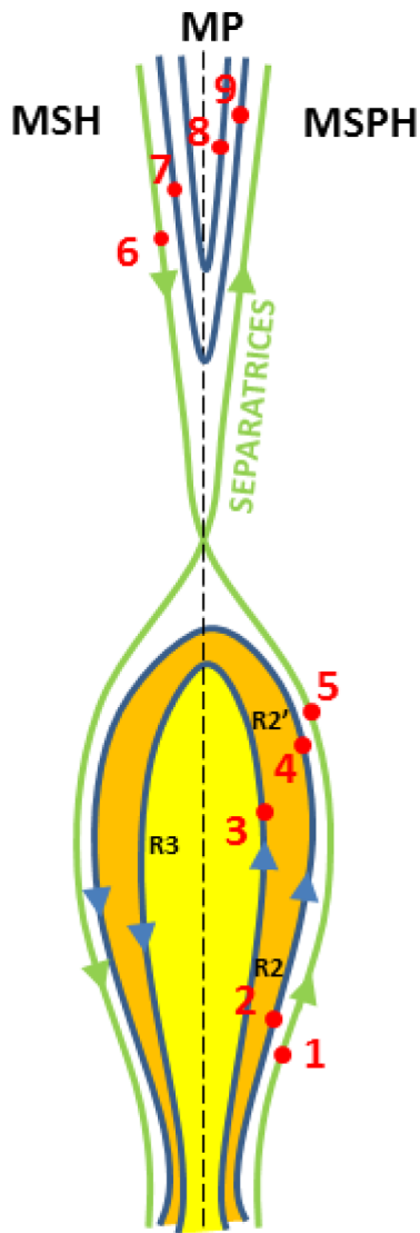
Figure 5. A schematic of the flux transfer event which includes the structure of the reconnection layer as inferred from our observations.
