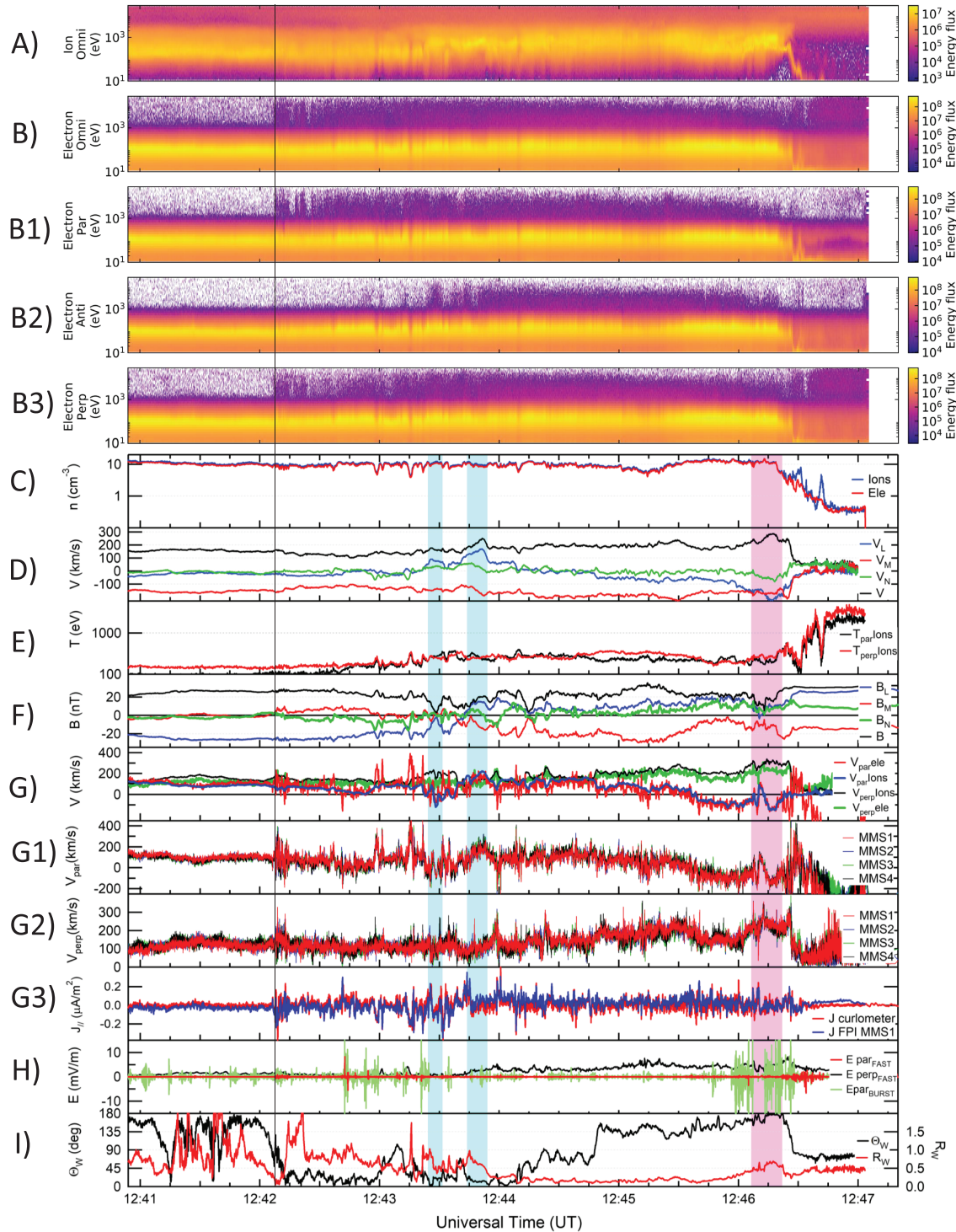
Figure 4. An enlargement about the reconnection jets observed in the last part of the event, with the same format as Figure 3. The cyan and pink shadings highlight the northward and southward reconnection jets, selected by means the Walén relation. The black line indicates the magnetic separatrix.
