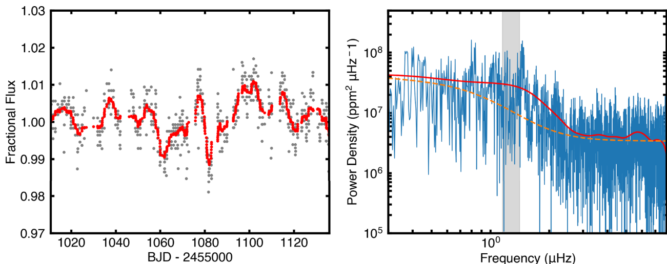
Figure 3. Left: Subset of the OGLE-IV baseline flux spanning 125 d. The red line shows a boxcar smoothing with a width of 0.5 d. The quasi-periodic variability with a timescale of 9 d is due to convection-driven oscillations. Right: power spectrum of the full light curve after removing the microlensing event. The orange dashed line shows the background model, and the red line is a heavily smoothed version of the power spectrum used to measure the frequency of maximum power. \nu_{\max} = 1.28 \pm 0.13 \mu\text{Hz} is the peak of the smoothed curve after subtracting the background model (the shaded grey area shows the 1\sigma region of \nu_{\max} ).
