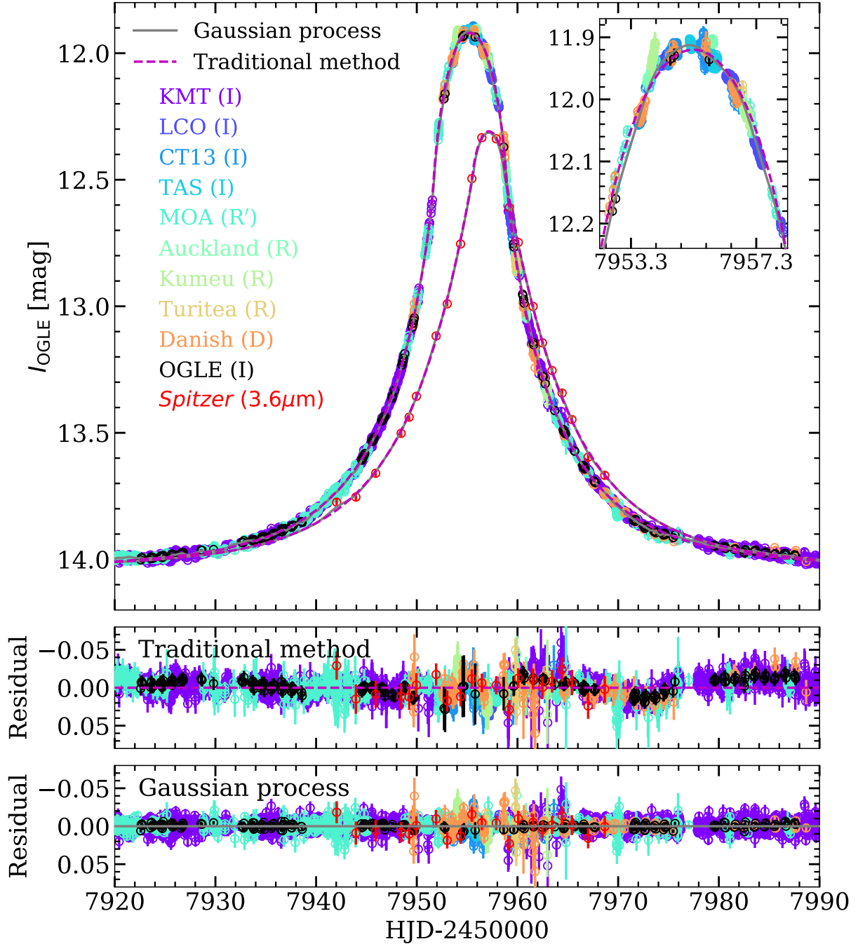
Figure 1. Top panel: the light curve of OGLE-2017-BLG-1186 with the best-fitting models for OGLE (or I -band) data, i.e. the (+, -) case, from both the traditional method (magenta dashed line) and the GP method (grey solid line). The inset shows the peak in greater detail. Lower panels: residuals for each method.
