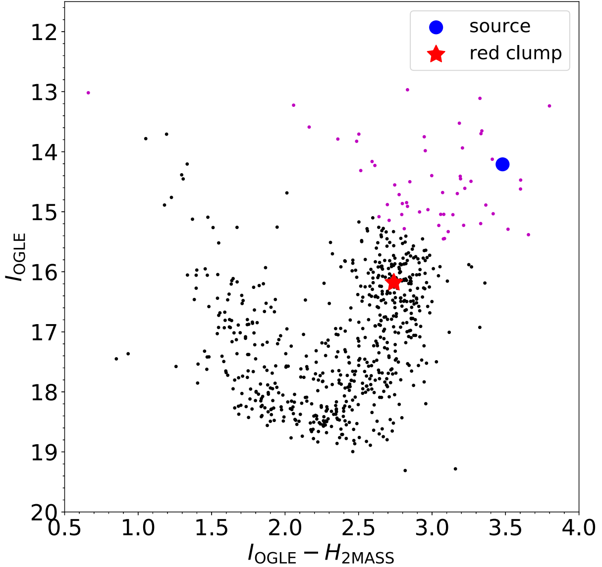
Figure 4. CMDs of a 2 arcmin \times 2 arcmin square centred around OGLE-2017-BLG-1186. Because the saturation limit of VAV catalogue is H \sim 12.0 , we use H -band photometry from the VAV catalogue (black dots) for H > 12.5 and H -band photometry from the 2MASS catalogue (magenta dots) for H < 12.5 . The VAV catalogue has been calibrated to the 2MASS photometric system. The red asterisk shows the centroid of the red clump, and the blue dot indicates the position of the source star.
