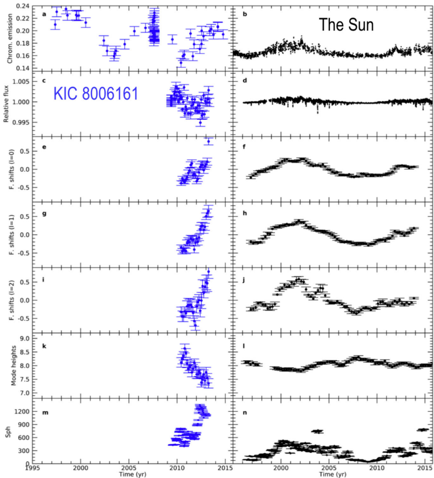
Fig. 4.3 Activity proxies as a function of time for KIC 8006161 (left panels) and the Sun (right panels). The panels show from top to bottom: the chromospheric emission, the relative flux, radial frequency shifts, frequency shifts of dipolar modes, frequency shifts of quadrupolar modes, logarithmic mode heights of the modes and S_{\text{ph}} . Image reproduced with permission from Karoff et al. (2018), copyright by ESO
