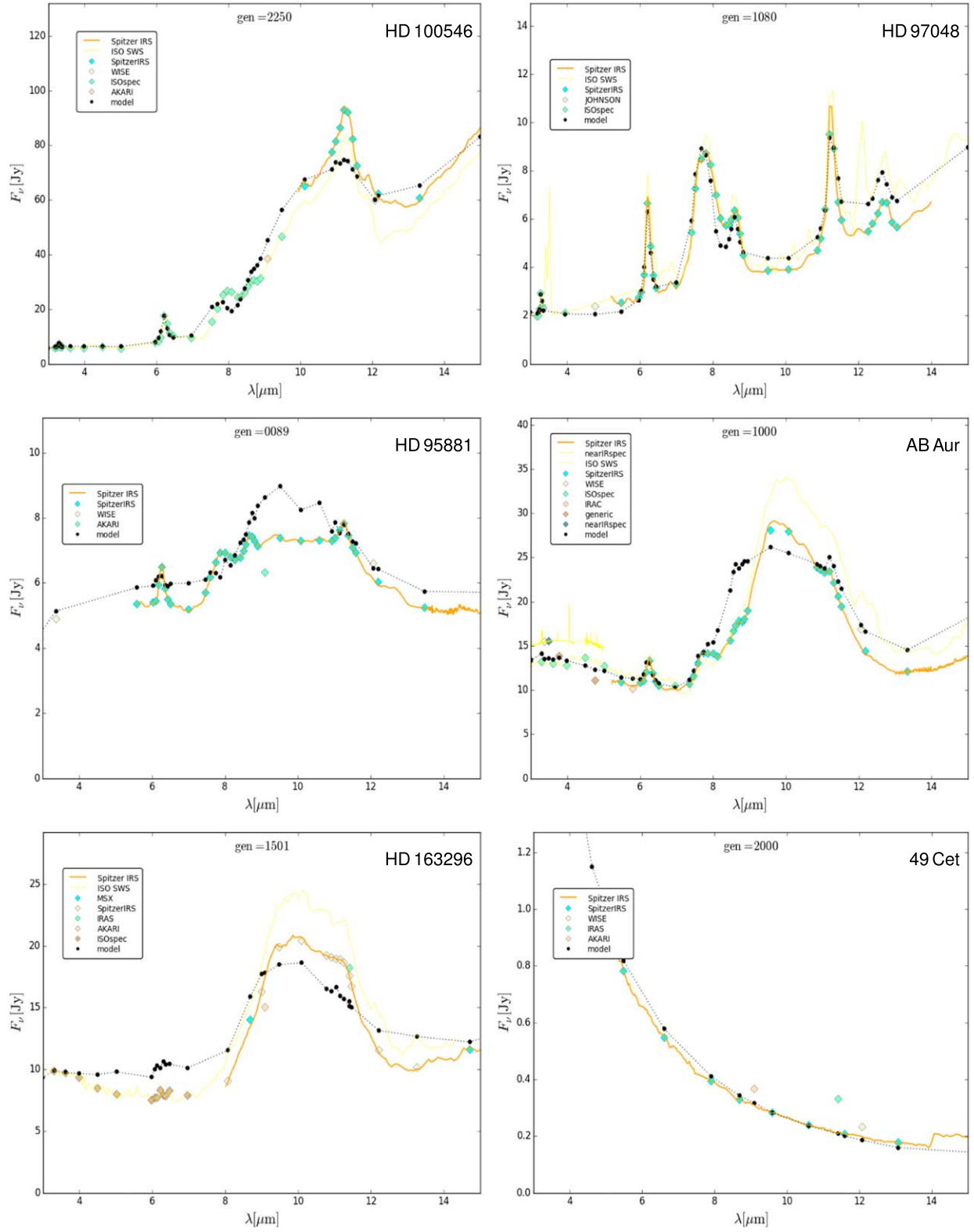
Figure 35. Enlargements of the SED-fits in the mid-IR region on linear scales, centered around the broad silicate emission feature at 10 \mu m and the PAH emission features at 3.3, 6.25, 7.85, 8.7, 11.3, and 12.7 \mu m. All results have been obtained with the DIANA standard dust opacities, see text, where only the powerlaw parameters of the dust size-distribution and the volume fraction of amorphous carbon was varied for the fit. Therefore, detailed fits of the spectral shapes of the features are not expected. Concerning the PAHs, only the abundance of the PAHs and the fraction of charged PAHs was varied for fitting.
