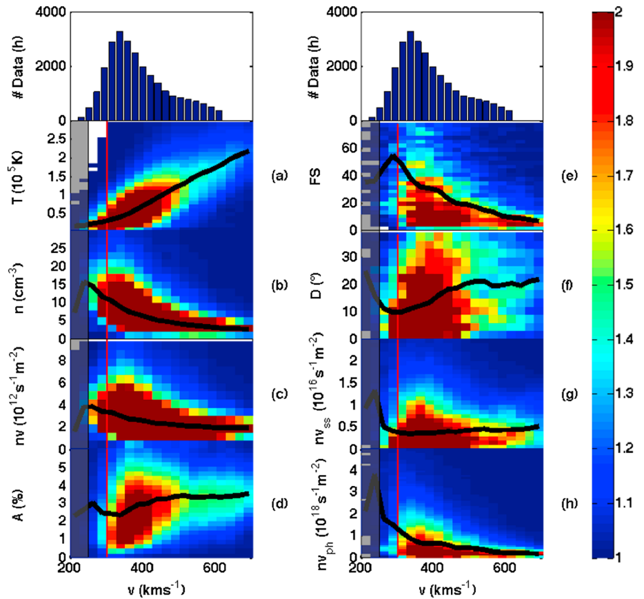
Figure 4. For each panel, using the entire Helios 1 and 2 data sets, excluding ICMEs, we display the percentage of samples for a given pair of values ( V , Y ) where V is the solar wind speed and Y the property on the Y axis. The black line shows the median of that quantity for each velocity interval. (a–d) The quantities directly measured in situ and (e–h) the properties at the Sun resulting from tracing the in situ measurements back to the Sun. The corresponding quantities are the following: (Figures 4a–4d, measured in situ) proton temperature, proton density, proton flux, He abundance, (Figures 4e–4h, back traced) field line expansion factor, distance to the photospheric neutral line and proton flux at the source surface, and above the photosphere. The red vertical line is at 300 km/s to separate the slow solar wind from the VSSW. On top of each column a histogram shows the distribution of all Helios samples (in units of time). The properties below 250 km/s lack sufficient statistics (less than 200 h of measurement) and are thus shaded in grey to highlight the necessary caution with this interval. Bins have a size of 25 km/s and cover a speed range from 200 km/s to 700 km/s. In Figures 4a–4d, the proton density and proton flux are scaled to 1 AU with a R^{-2} dependence and the temperature with R^{-0.7} [Ebert et al. , 2009]. Only data inside 0.7 AU are included.
