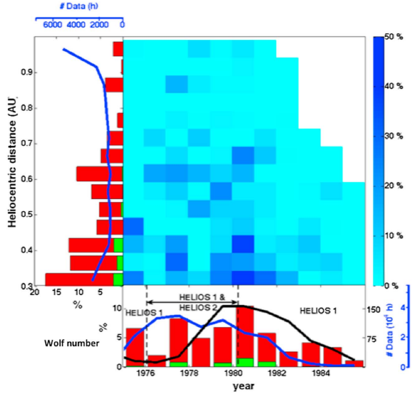
Figure 2. (middle) Space-time distribution of the VSSW from all Helios data from 1975 to 1985. For a given year and radial helio-spheric distance, the percentage of VSSW ( V < 300 km/s) is given as the percentage of total wind measured in that time and distance bin, and according to the right-hand side color palette. (left) Time integral of the central plot, showing the percentage of solar wind samples slower than 300 km/s (red) and slower than 250 km/s (green) as a function of heliocentric distance. The blue line represents the amount of data samples, in hours. (bottom) Spatial integral of the central plot, showing the percentage of solar wind samples slower than 300 km/s (red) and slower than 250 km/s (green) as a function of year from 1975 to 1985. The black line represents the yearly averaged Wolf sunspot number, and the blue line shows the amount of data, in hours. Vertical dashed lines show the launch and decommissioning of Helios 2, whose science operations were shorter than Helios 1.
