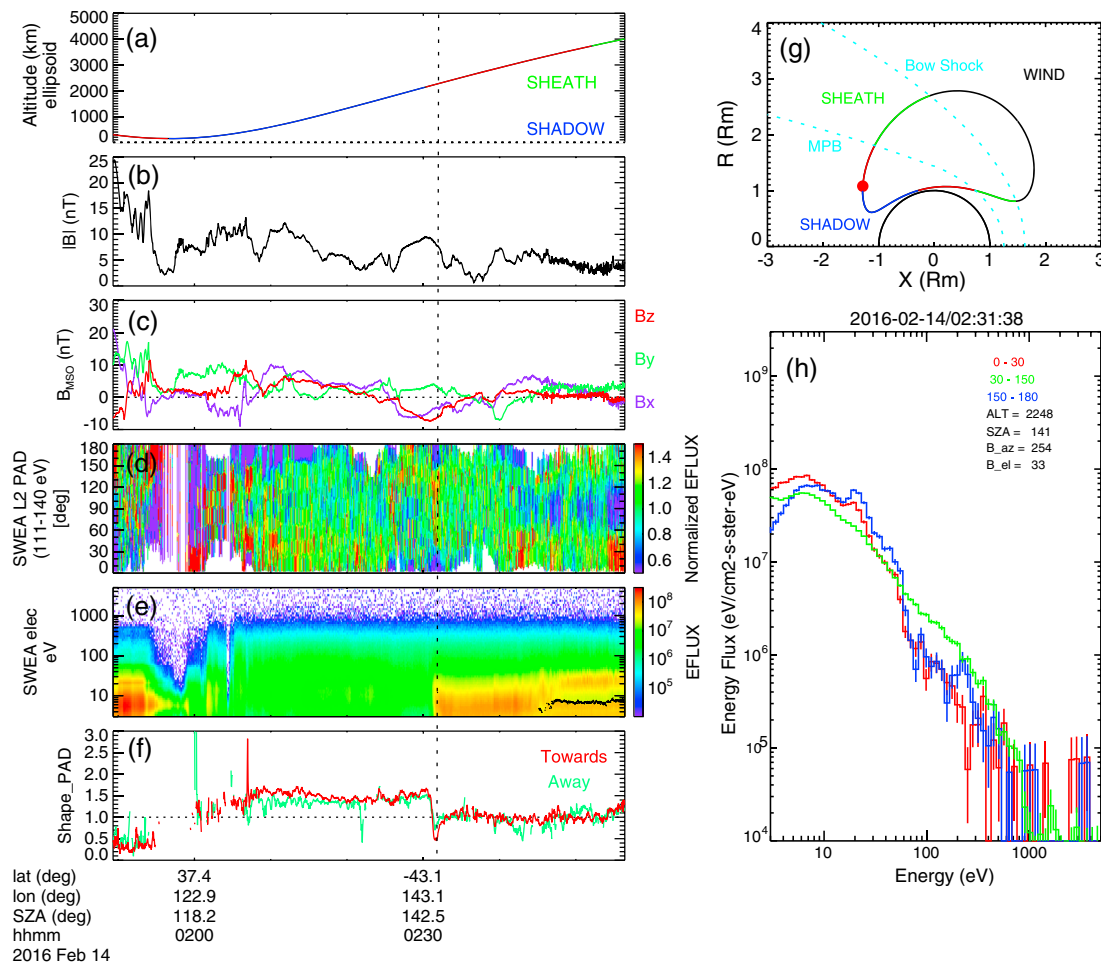
Figure 1. Time series of (a) spacecraft altitude, (b) magnetic field magnitude and (c) components in MSO coordinates measured by MAG, pitch angle distribution (PAD) of (d) 111–140 eV electrons, (e) energy spectra measured by SWEA, and (f) pitch angle-resolved shape parameters on 14 February 2016. The black dots in Figure 1e indicate the spacecraft potential estimated by SWEA measurements. In Figure 1f, “away” and “toward” indicate electron movement relative to the planet, determined from pitch angles and magnetic elevation angles. (g) The orbit geometry in MSO cylindrical frame, with X pointing at the Sun and R being the distance from the X axis. (h) The electron energy spectra for pitch angle (PA) 0^\circ - 30^\circ (red), 30^\circ - 150^\circ (green), and 150^\circ - 180^\circ (blue), extracted at time indicated by the vertical dashed line in the left panels and the spacecraft location indicated by the red dot in Figure 1g. In Figures 1a and 1g, altitudes and orbit trajectories are colored according to nominal locations of the plasma regions, with fitted parameters from Trotignon et al. (2006). MPB refers to the magnetic pileup boundary.
