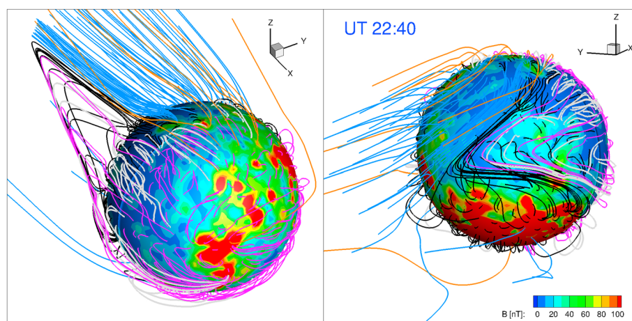
Figure 3. An example of magnetic field lines derived from a time-dependent MHD simulation by Ma et al. (2014) and Fang et al. (2015). The snapshot corresponds to a time point in the simulation when the strongest crustal field region is located on the nightside. The field lines have foot points at 150 km altitude on 10 \times 10^\circ longitude-latitude grids. The color on the spherical surface is the magnetic magnitude at 105 km. As no draped solar wind-entrained field lines can penetrate down to such a low altitude, only closed and open field lines are shown, magenta for both foot points on the dayside, black for both foot points on the nightside, gray/white for cross terminator closed loops, orange for open field lines with one foot point on the dayside, and blue for open field lines with one foot point on the nightside.
