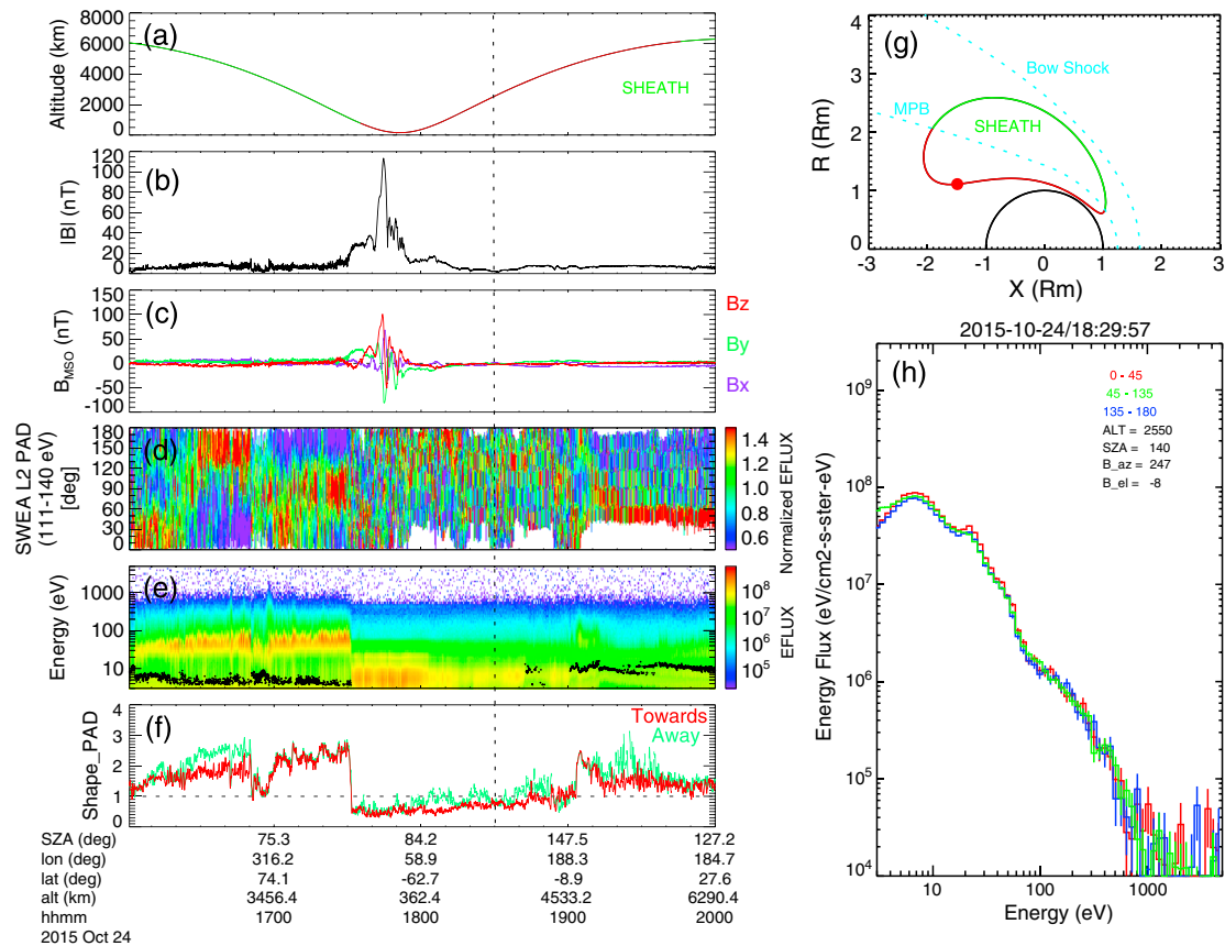
Figure 2. The ephemeris, magnetic field, and electron information of an orbit on 24 October 2015, the same format as Figure 1.
