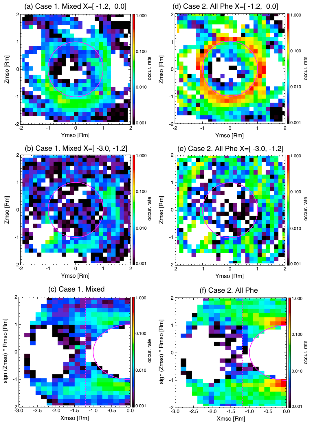
Figure 4. The occurrence rate of the high-altitude closed loops in three projections, the left column for case 1 and the right column for case 2. The top two rows are in the Y_{MSO} - Z_{MSO} plane for two X_{MSO} ranges: (a–d) X_{MSO} = [-1.2, 0] and (b and e) X_{MSO} = [-3, -1.2] , respectively, and (c and f) the MSO cylindrical coordinates with radial distance signed by \pm Z_{MSO} .
