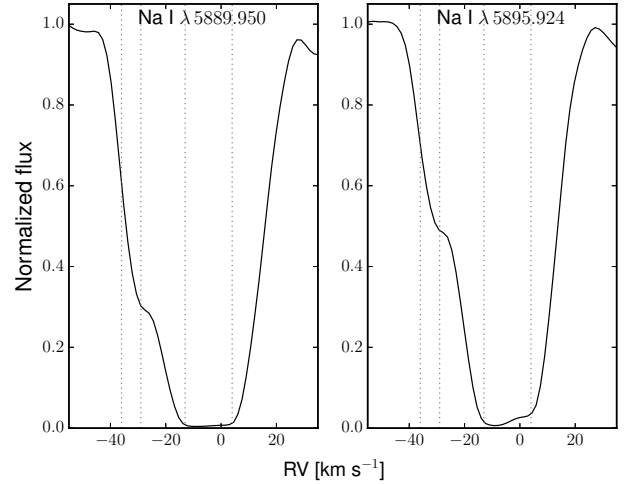
Fig. 10. Section of the FEROS spectrum of HD 166734 showing the Na I interstellar lines, covering a velocity range of -55 to +35 km s -1 . The dotted lines indicate, from left to right, RVs of -36 , -29 , -13 , +4 km s -1 for both panels.
