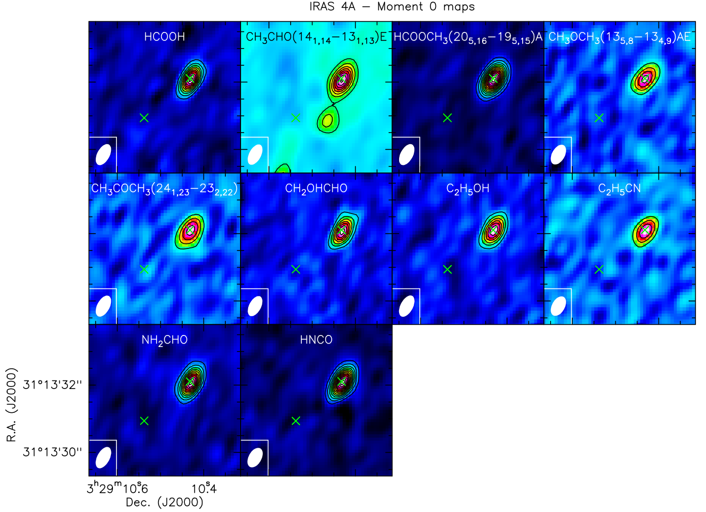
Fig. 4. Moment 0 maps of representative molecular lines observed with ALMA. The transition is specified if more than one line from the same species was detected. The continuum peak position of the two protostellar cores A1 and A2 are indicated with green crosses. Contours start at 5\sigma and increase by steps of 5\sigma in all the maps. The values of \sigma for each map are summarised in Table 3. The synthesised beam is depicted in white in the lower left corner.
