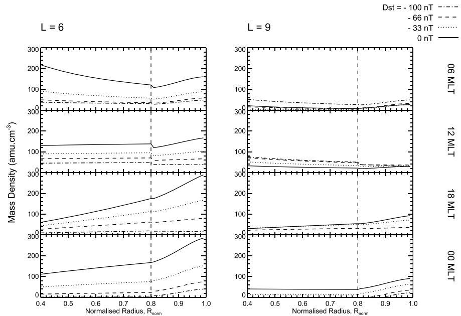
Figure 6. Panels showing the mass density ( \text{amu cm}^{-3} ) as a function of the normalized radius, R_{\text{norm}} . The mass density values are calculated by combining the electron density (equation (2)) and average ion mass (equation (3)) field-aligned models using equation (1). Each panel shows the field line distribution at a different value of the D_{st} index (nT), as indicated by the linestyle. Profiles for (left) L = 5 and (right) L = 9 ; the vertical panels show profiles for multiple MLT values. The vertical dashed lines on each panel indicate the boundary separating the power law and Gaussian form field-aligned dependence for the electron density model.
