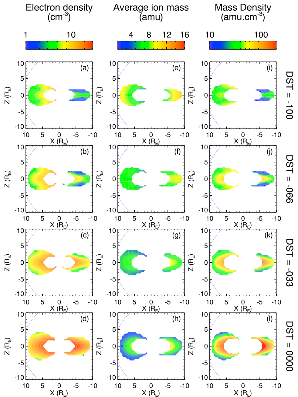
Figure 2. Spatial distribution in the X - Z SM plane using the field-aligned models for (a–d) electron density and (e–h) average ion mass, defined by equations (2) and (3), respectively. (i–l) The models are combined to infer the corresponding total mass density distributions. Each vertical panel shows the distribution for a different value of the D_{st} index (nT). The T96 magnetic field model used corresponds to spring equinox, with a solar wind dynamic pressure of 2 nPa. The expected locations of the magnetopause under these conditions are included as the blue solid lines for reference.
