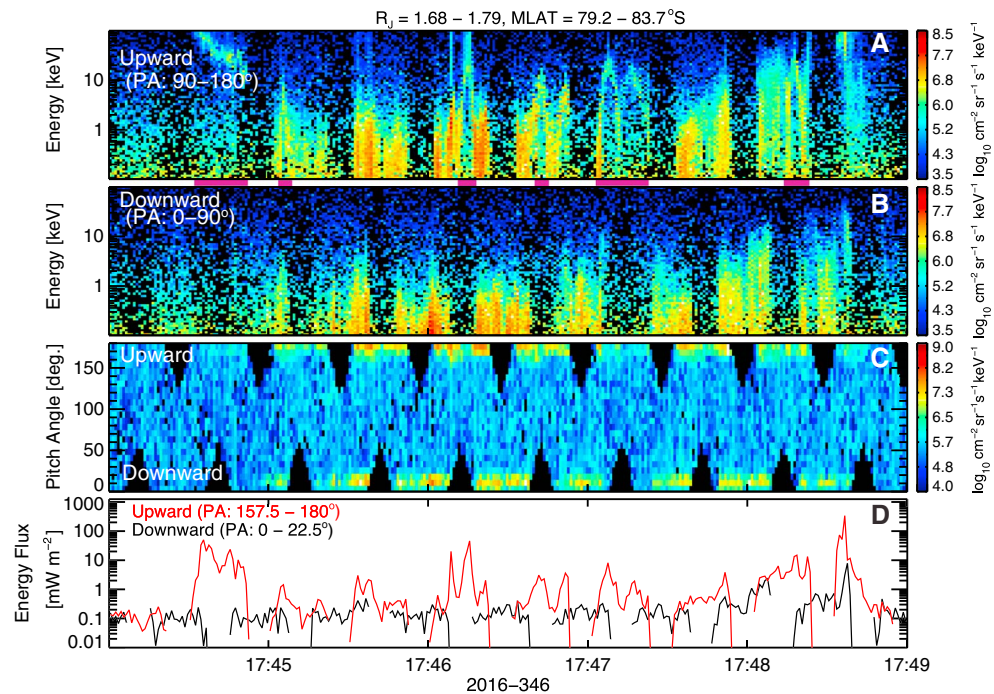
Figure 3. The 0.1–100 keV electron observations over Jupiter’s southern pole during PJ3 when Juno ranged between 1.68 and 1.79 R_J in jovian distance and 79.2–83.7°S in magnetic latitude. (a and b) Energy-time pitch angle averaged differential intensity spectrograms for electrons with pitch angles between 90° and 180° (upward, Figure 3a) and 0° and 90° (downward, Figure 3b), respectively. Purple horizontal bars identify possible inverted-V structures. Figure 3c displays pitch angle-time spectrograms of electron intensity (summed over energies from ~0.1 to 100 keV). Black triangular regions in the spectrograms reflect pitch angles that were not sampled due to E300 being off. The time series of estimated upward and downward electron energy fluxes within 22.5° of the magnetic field are shown in Figure 3d.
