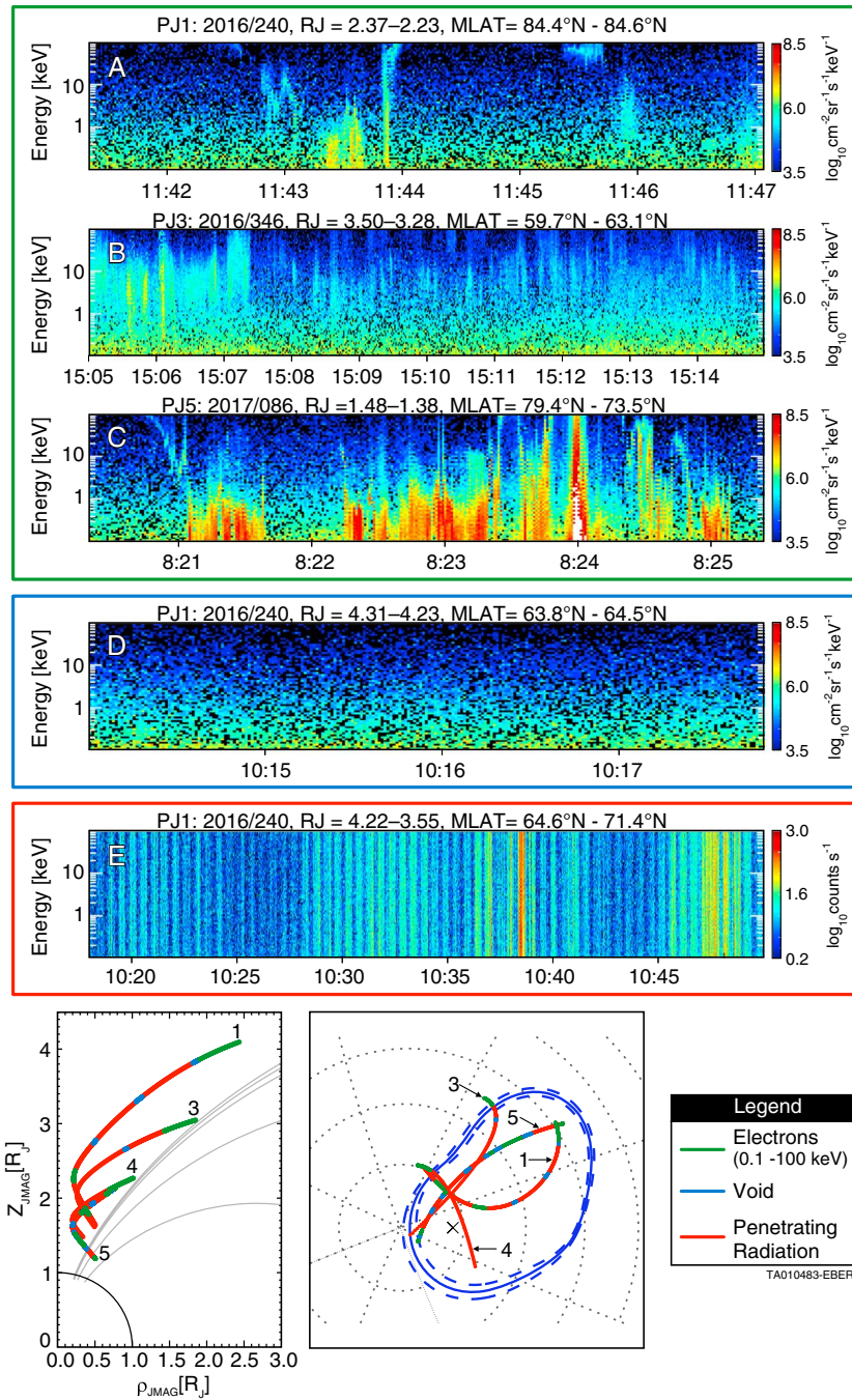
Figure 1. Displayed are representative intervals of (a–c) regions with 0.1–100 keV electrons (green box), (d) regions void of these electrons (blue box), and (e) regions dominated by penetrating radiation (red box) in Jupiter’s northern polar auroral region prior to Juno perijoves 1, 3, and 5. (f) Juno’s trajectory over Jupiter’s northern polar region in a magnetic coordinate system based on the VIP4 + CAN magnetic field model (e.g., Connerney et al., 1981, 1998). Green, blue, and red lines denote periods when JADE-E observed 0.1–100 keV electrons, regions void of these electrons, and penetrating radiation, respectively. Each trajectory is labeled by its associated perijove number. (g) Magnetic projection of Juno’s trajectory onto Jupiter’s atmosphere and relative to the statistical average position of Jupiter’s main aurora as derived from Hubble Space Telescope UV observations (Bonfond et al., 2012). Black dashed circles and lines denote contours of constant jovicentric latitude and system III longitude, respectively. Color-coded JADE-E region identification is the same as Figure 1f.
