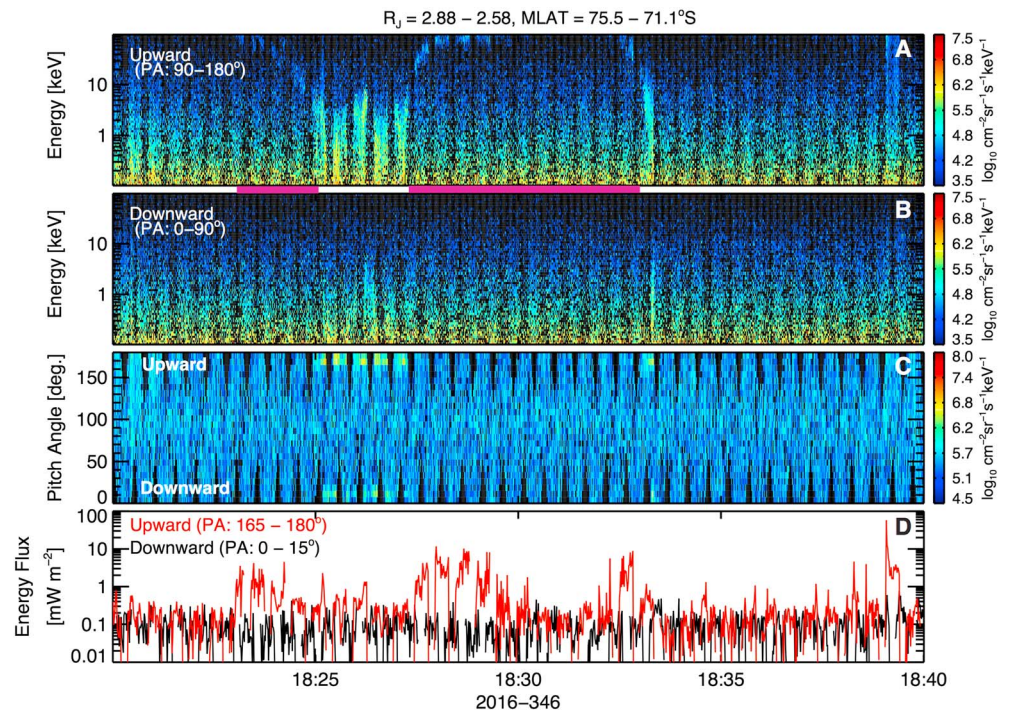
Figure 4. Similar format as Figure 3 but for a period over Jupiter’s southern pole during PJ3 when Juno ranged between 2.88 and 2.58 R_J in joviocentric distance and 75.5–71.1°S in magnetic latitude.
