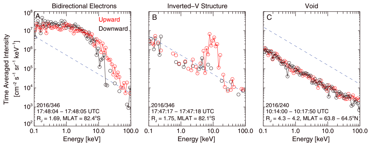
Figure 5. Energy spectra for periods when JADE-E observed (a) bidirectional electrons, upward electrons with an (b) inverted-V energy distribution, and (c) a void. The intensities have been averaged over the number of pitch angle bins used in the calculation and the number of 1 s measurements in the stated time interval. Blue dashed lines denote the JADE-E intensity assuming 1 count per energy step for a 1 s accumulation period divided by the number of pitch angle bins used in each energy spectra calculation.
