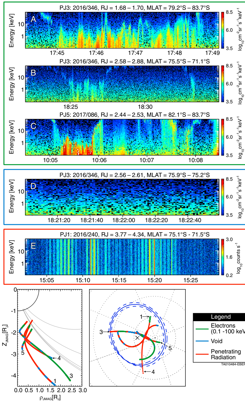
Figure 2. Same format as Figure 1 but for 0.1–100 keV electron observations in Jupiter’s southern polar region during the polar passes immediately after Juno perijoves 1 and 3–5.
