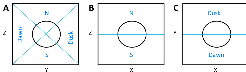
Figure 4. Cartoon diagram of the binning method used to produce statistical maps in this study. (a) The Y-Z plane cut into four regions—north (N), south (S), dawn, and dusk. (b and c) Data from these regions are used to produce the maps, looking at different planes. This system is used for both the MSO and MSE frames at Mars. Only data between -1 R_M < 1.5 R_N are used when creating the statistical map shown in Figure 4a.
