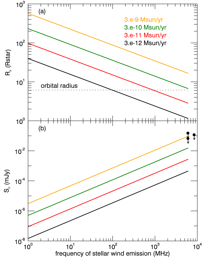
Fig. 4. a) Size of the stellar wind radio-emitting region as a function of frequency for a range of stellar mass-loss rates: 3 \times 10^{-12} M_\odot \text{ yr}^{-1} to 3 \times 10^{-9} M_\odot \text{ yr}^{-1} from bottom to top solid lines. The dotted line indicates the orbital radius of V830 Tau b. b) The same as in a) , but for the flux density of the emitting wind, S_\nu . Circles are the upper limits for the radio emission of V830 Tau b as presented by Bower et al. (2016).
