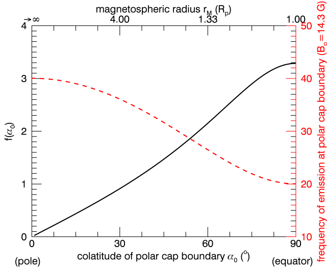
Fig. A.1. Black solid curve: variation of f (Eq. (A.12)) as a function of the planetary co-latitude of the polar-cap boundary \alpha_0 . The top axis indicates the (non-linear) conversion from \alpha_0 to a normalised magnetospheric size following Eq. (A.1). Red dashed curve: the emission frequency at the polar-cap boundary (Eq. (A.3), right axis) for a magnetic field intensity at the pole of 14.3 G.
