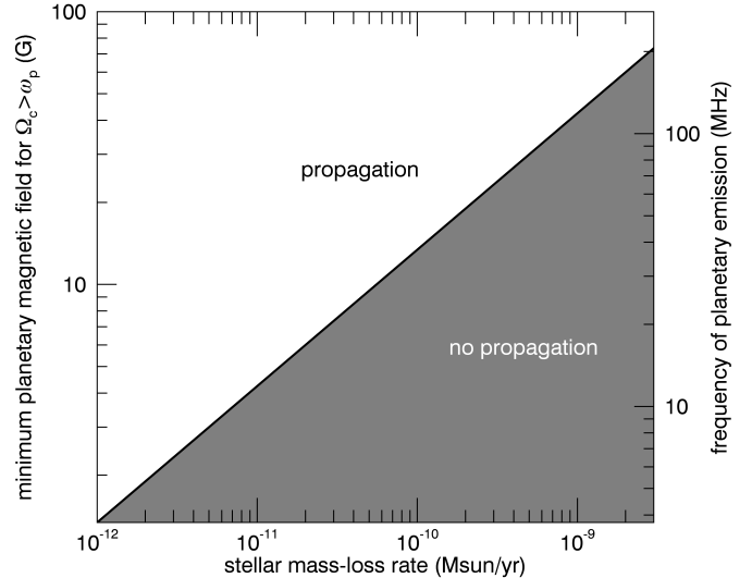
Fig. 5. Minimum planetary magnetic field intensity required for the propagation of planetary radio emission through the wind of the host star (Eq. (15)) as a function of stellar wind mass-loss rate. The right hand side axis shows the corresponding frequency of planetary emission (cyclotron).
