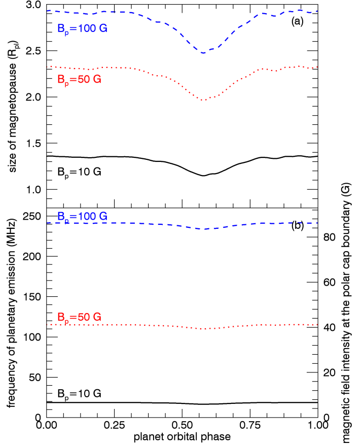
Fig. 2. a) Estimated sizes of the planetary magnetospheres along a planetary year assuming three different values of the polar planetary magnetic field: 10, 50, and 100 G. b) Predicted maximum frequency of the radio emission of V830 Tau b. This frequency is calculated at the border of the polar-cap boundary, which is located at different colatitudes depending on the size of the planet magnetosphere (cf., Eq. (A.1)). The magnetic field intensity at this position is shown in the right axis.
