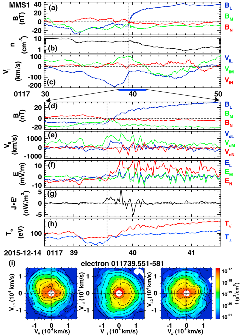
Figure 1. Overview of an EDR encounter by MMS. Data are from MMS1. (a) B in LMN with the transformation matrix to GSE given by (L, M, N) = ([0.27, -0.54, 0.79], [-0.41, -0.82, -0.41], [0.87, -0.21, -0.44]) ; (b) density n ; (c) the ion velocity V_{iLMN} ; (d–h) zoom-in view of B_{LMN} , V_{eLMN} , E_{LMN} (8192 samples/s averaged to the cadence of the electron data, 30 ms per sample), J \cdot E' and T_{e\parallel, \perp} . (i) An electron distribution in three orthogonal velocity planes establishes that MMS1 encounters the sheath part of the EDR: a magnetic field-aligned counterstreaming sheath component combined with the EDR-accelerated electrons forming a triangular structure in v_{\parallel} - v_{\perp 1} . The nongyrotropic electrons are unmagnetized (see text for explanations) and contribute to a crescent-like shape in the v_{\perp} plane due to finite gyroradius effects.
