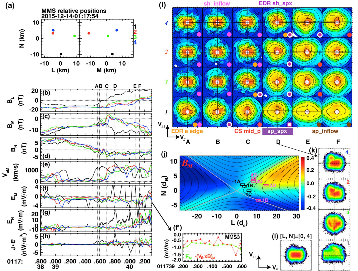
Figure 3. The EDR encounter by the four MMS spacecraft and comparison with PIC simulation results. (a) Relative positions of the spacecraft. (b) B_L and (c) B_M at MMS1 remain negative even in the sheath part of the +L exhaust, indicating a guide-field dominated region. MMS2–MMS4 observe a brief positive B_M excursion, showing traversals of the edge of the Hall B-dominated region. (d) The B_N reversals of all four spacecraft imply a transition from -L to +L of the X line. (e) The electron out-of-plane flow V_{em} . (f) The out-of-plane electric field E_M , consistent with the expected reconnection electric field. (f') Agreement of the MMS3 E_M and -(V_e \times B)_M , supporting the accuracy of EM measurements in the sheath inflow. (g) The electric field normal to the current layer E_N (averaged to the cadence of the B data, 128 sample/s) reverses sign slightly before the B_L reversal for each spacecraft (h) The energy conversion due to the nonideal E ( J \cdot E' ) enhances with V_{em} . (i) MMS v_{||} - v_{\perp 1} DF array (using the same colorbar and velocity range as those in Figure 1i) arranged according to the N positions of the spacecraft in rows and time in columns (A–F from left to right, corresponding to the vertical dotted lines marked in Figures 3b–3h) to provide a visual for the EDR encounter. The distinct electron regions are color coded and annotated. (j) PIC simulation predictions for B_M . (k) The PIC DFs for the four spacecraft locations at frame D (the spacecraft locations are marked by magenta boxes in Figure 3j). For reference, the locations of MMS1 for frames A–C are also noted (black) in the B_M panel to facilitate the comparison with the DFs in Figure 2. (l) A PIC DF showing that only sheath inflow electrons are present at N > -4 d_e from B_L = 0 .
