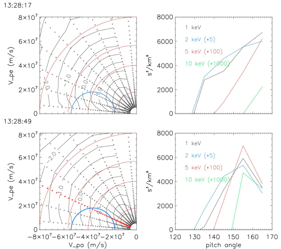
Figure 2. (left column) Distribution of the upgoing electrons at 13:28:17 and 13:28:49. The isocontours are shown using a logarithmic scale in units of s^3/km^6 . The red circular arcs correspond to energies of 1, 5, 10, and 20 keV and the radial lines to pitch angles of 175^\circ , 165^\circ , 155^\circ , .... An example of a resonant circle is displayed in blue. (right column) Corresponding \partial f/\partial v_\perp gradients (units of s^3/km^6 ) at 1, 2, 5, and 10 keV, measured in the loss cone.
