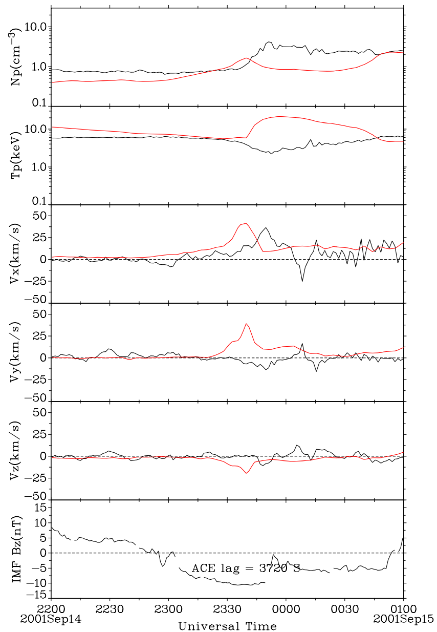
Figure 9. Simulation (red lines) versus LANL97A observations (black lines) from 22:00:00 UT on 14 September to 01:00:00 UT on 15 September. Shown are the same parameters as in Figure 7.
