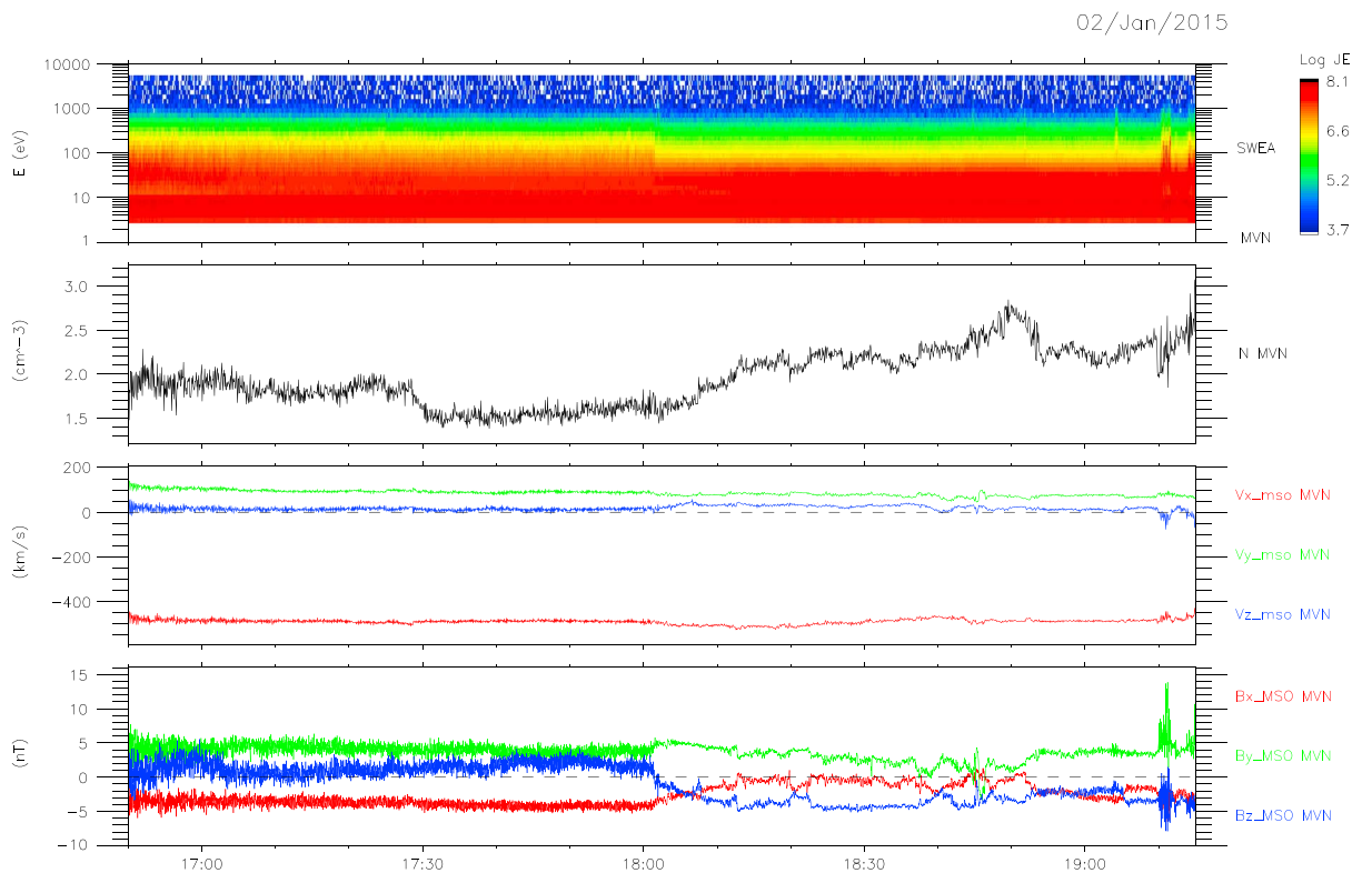
Figure 2. (first panel) The MAVEN-SWEA energy spectrogram for 2 January 2015, 1650–1915 UT. The following successive panels display respectively (second panel) the ion density, (third panel) the MSO components of the solar wind velocity, and (fourth panel) the magnetic field.
