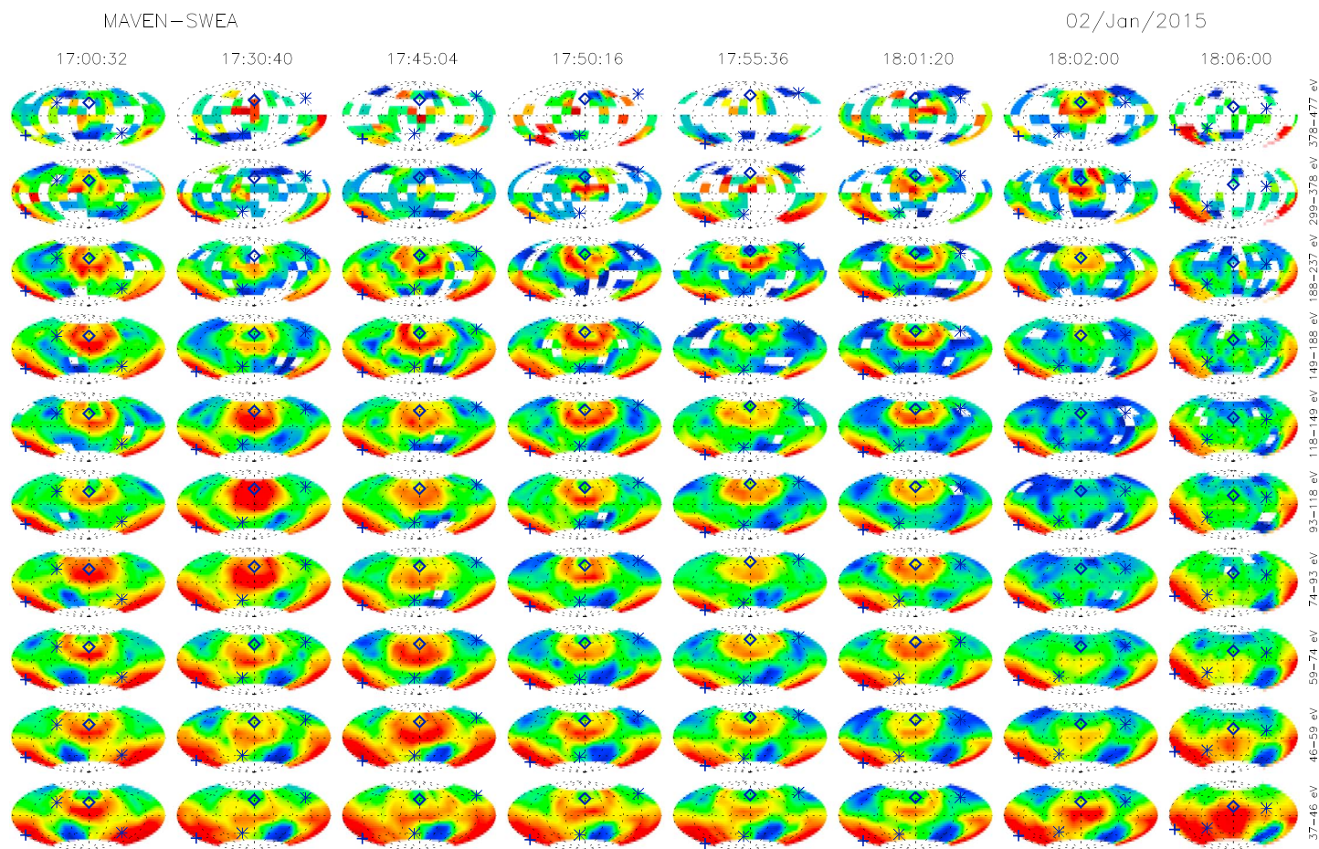
Figure 4. Snapshots of electron angular distribution for 10 selected energy ranges. The Hammer-Aitoff equal area projection is used. The cross (diamond) symbol represents the direction of \mathbf{B} ( -\mathbf{B} ) direction. The color scale corresponds to distribution function values and is normalized for each Hammer-Aitoff slice.
