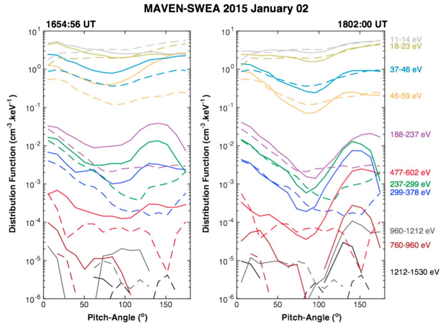
Figure 5. Two snapshots of the electron distribution measured by MAVEN-SWEA instrument. The solar wind distribution is represented by the dashed lines, and the energy ranges are indicated on the right panel. An instant for which the magnetic field direction is connected at a (left) quasi-parallel and (right) quasi-perpendicular geometry.
