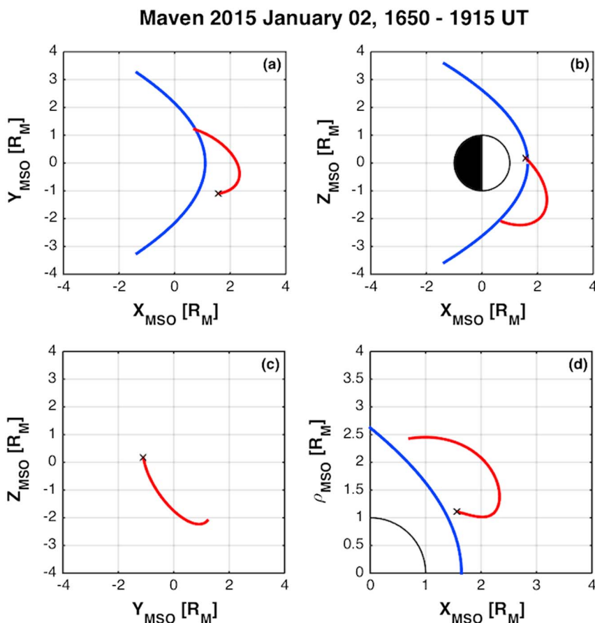
Figure 1. Cross sections of Mars model bow and MAVEN orbiter's path during the time of interest. Mars-centered Solar Orbital (MSO) system of coordinates is used.
