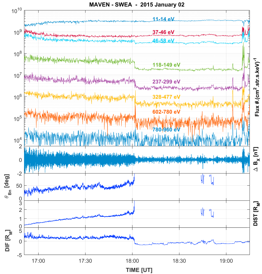
Figure 3. (first panel) The electron flux for eight selected energy ranges, (second panel) the B_x fluctuation level with respect to a running average, (third panel) the angle \theta_{Bn} , (fourth panel) the distance of MAVEN to the shock DIST, and (fifth panel) the foreshock depth DIF.
