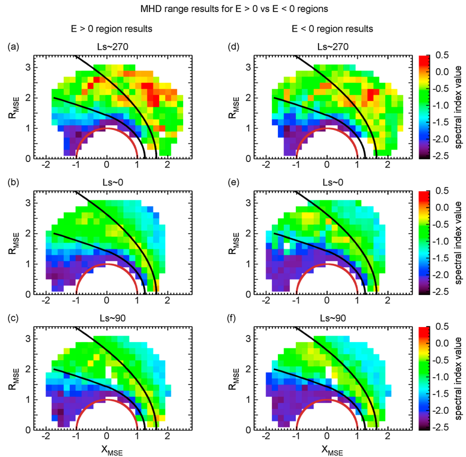
Figure 11. MHD range spectral indices in the magnetospheric hemispheres facing the positive and negative upstream electric field directions plotted in X_{MSE} versus R_{MSE} maps. (a–c) Orbit maps for the E > 0 region spectral indices. (d–f) Orbit maps for the E < 0 region spectral indices. The spectral indices show asymmetry in the upstream region for Ls \sim 270 .
