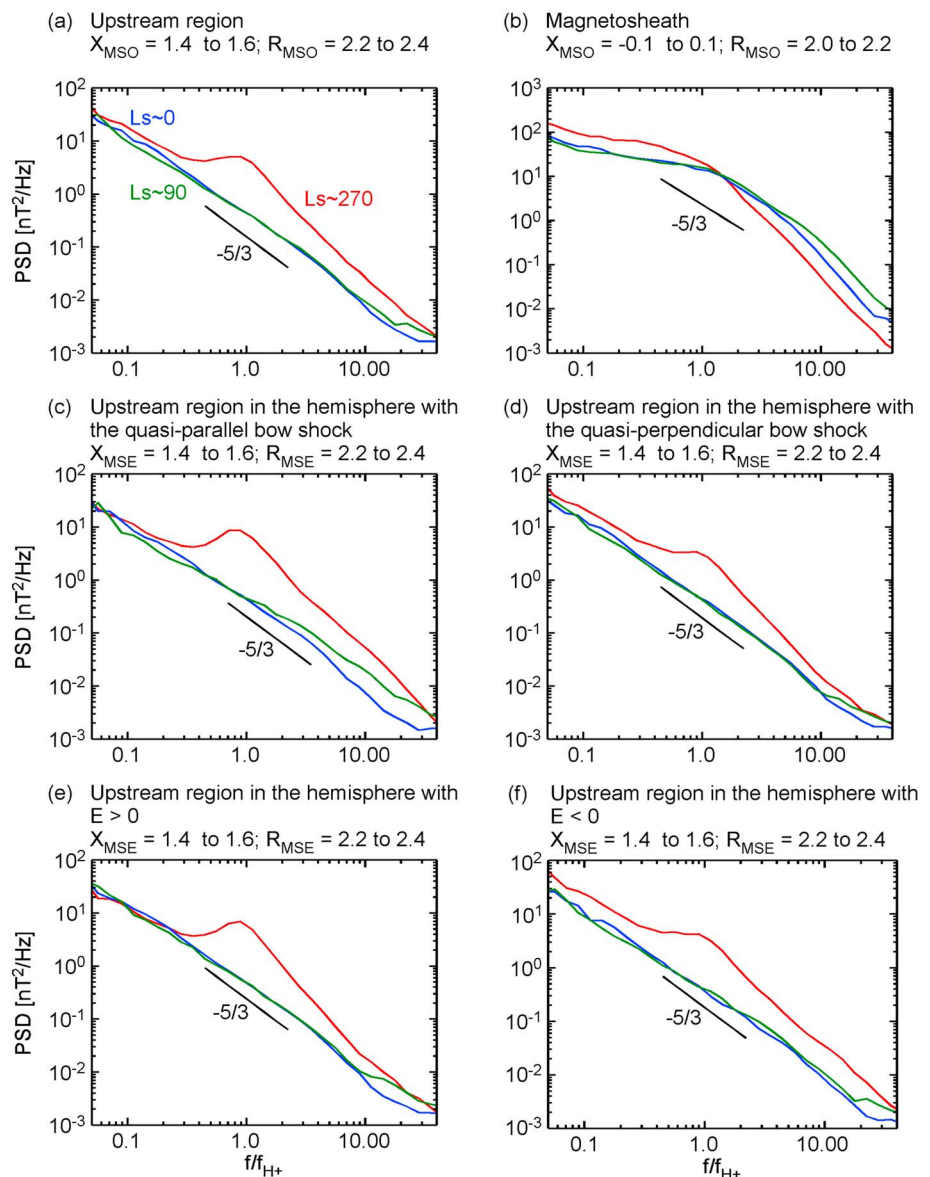
Figure 6. Power spectra for three seasons. (a and b) Power spectra in the upstream region and the magnetosheath. (c and d) Power spectra for the quasi-parallel and quasi-perpendicular regions. (e and f) Power spectra for the E > 0 and E < 0 regions. The black line depicts the slope corresponding to the Kolmogorov spectral index, and it is shown here for reference.
