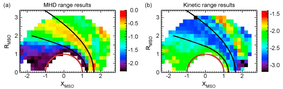
Figure 5. (a) MHD range spectral indices shown in a X_{\text{MSO}} versus R_{\text{MSO}} = \sqrt{(Y_{\text{MSO}}^2 + Z_{\text{MSO}}^2)} map. (b) Kinetic range spectral indices shown in a X_{\text{MSO}} versus R_{\text{MSO}} map. The colors indicate the values of the spectral indices. The MHD range spectral index values decrease when going deeper into the magnetosphere. The kinetic range spectral indices show the opposite trend. The banded structure in the upstream region is a consequence of the fact that the spacecraft only covered apoapsis far out in the subsolar region in the L_s \sim 270 time range.
