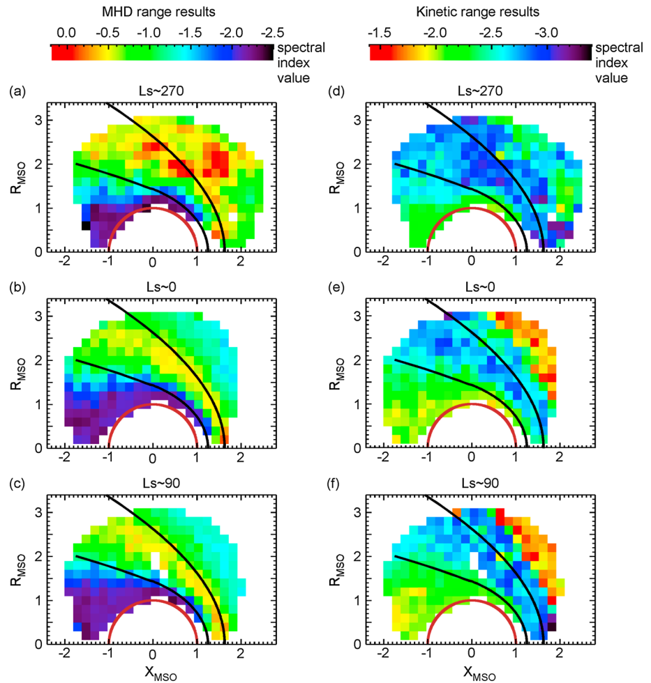
Figure 8. Seasonal variability of the spectral indices. (a–c) MSO orbit maps for the MHD range spectral indices for seasons L_s \sim 270 , L_s \sim 0 , and L_s \sim 90 . (d–f) MSO orbit maps for the kinetic range spectral indices for the same three seasons. The MHD range spectral indices show seasonal variability in the upstream region and in the magnetosheath, while the kinetic range spectral indices show seasonal variability in the upstream region and in the nightside magnetic pileup region.
