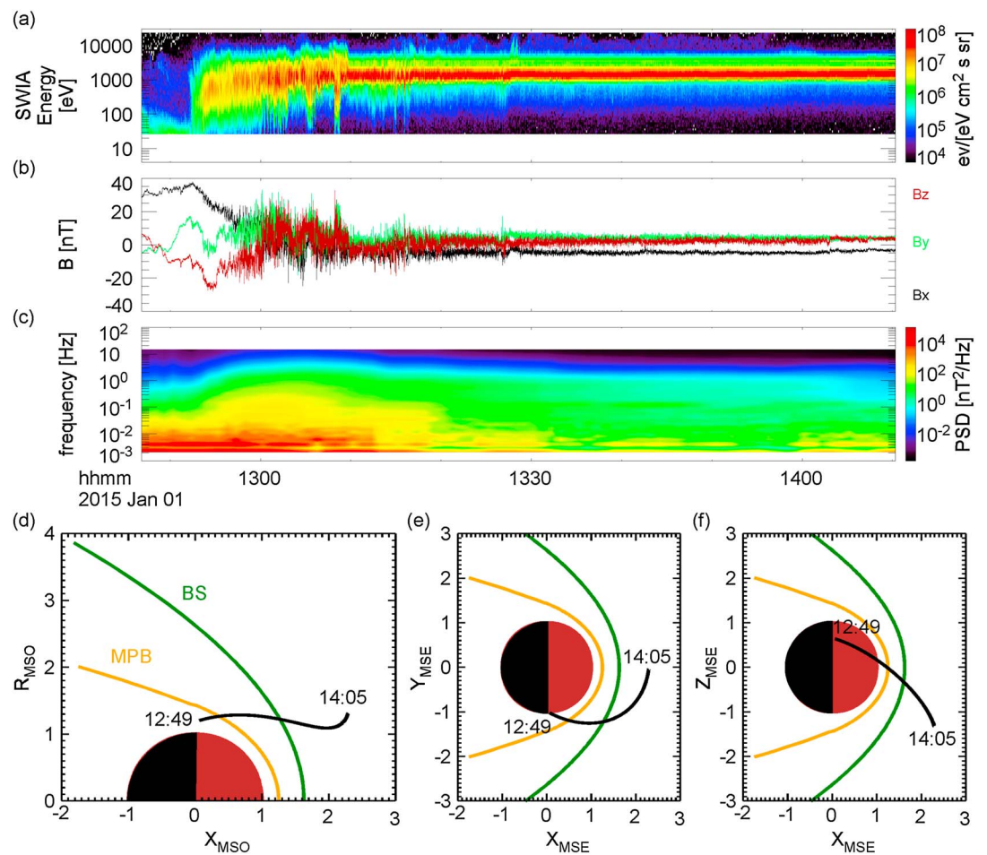
Figure 2. MAVEN observations and PSDs computed for magnetic field fluctuations for a portion of the MAVEN orbit. (a) The MAVEN Solar Wind Ion Analyzer measurements of the ion energy spectrum is shown here to merely give context for the observation. During this observation, the MAVEN spacecraft traversed from the magnetic pileup region which is typically populated by ions with energies < 100 eV, through the magnetosheath, which is populated by ions with energies centered at ~1 keV, and finally into the upstream region with ions that have energies centered also at 1 keV, but with a narrower temperature than in the magnetosheath. (b) Magnetic field time series. The magnetic field shows oscillations centered on various nonzero values because the spacecraft traversed through various regions of the Mars plasma environment during this time interval. As discussed in section 2, the solar wind magnetic field is subjected to compression and draping downstream of Mars' bow shock which lead to the variation of the local magnetic field. (c) Power spectral density for the magnetic field fluctuations computed using the wavelet transform. (d) The MAVEN orbit shown in a X_{MSE} versus R_{MSE} = \sqrt{Y_{MSE}^2 + Z_{MSE}^2} map. (e) The MAVEN orbit in a X_{MSE} versus Y_{MSE} map. (f) The MAVEN orbit in a X_{MSE} versus Z_{MSE} map.
