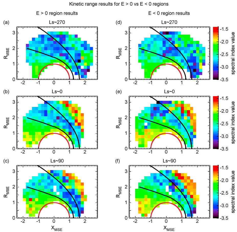
Figure 12. Kinetic range spectral indices in the magnetospheric hemispheres in the positive and negative electric field directions plotted in X_{MSE} versus R_{MSE} maps. (a–c) Orbit maps for the E > 0 region spectral indices. (d–f) Orbit maps for the E < 0 region spectral indices. The spectral indices do not show a discernible asymmetry in any of the seasons.
