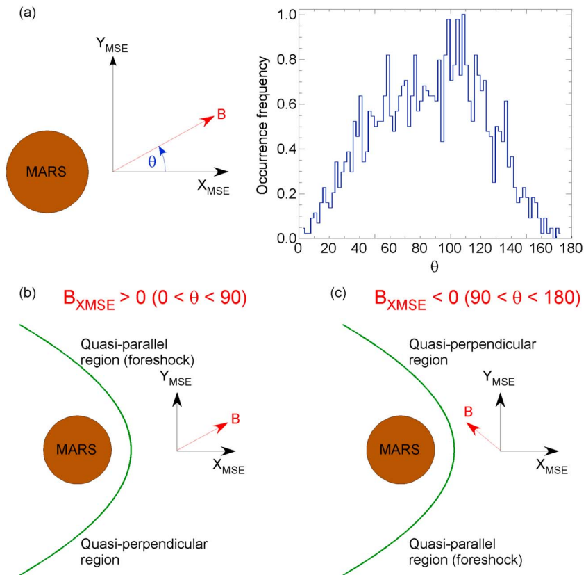
Figure 7. (a) Histogram of the upstream magnetic field orientation \theta . The X_{MSE} direction is aligned opposite to the solar wind flow direction, and the Y_{MSE} direction is aligned with the upstream magnetic field component perpendicular to the solar wind flow. Thus, the sign of B_{XMSE} or the X - MSE component of the magnetic field is indicative of the foreshock locations. (b) When B_{XMSE} > 0 or when 0^\circ < \theta < 90^\circ the quasi-parallel shock or the foreshock region is located at Y_{MSE} > 0 , whereas the quasi-perpendicular shock region is located at Y_{MSE} < 0 . (c) When B_{XMSE} < 0 or when 90^\circ < \theta < 180^\circ the quasi-parallel shock region is located at Y_{MSE} < 0 , whereas the quasi-perpendicular shock region is located at Y_{MSE} > 0 .
