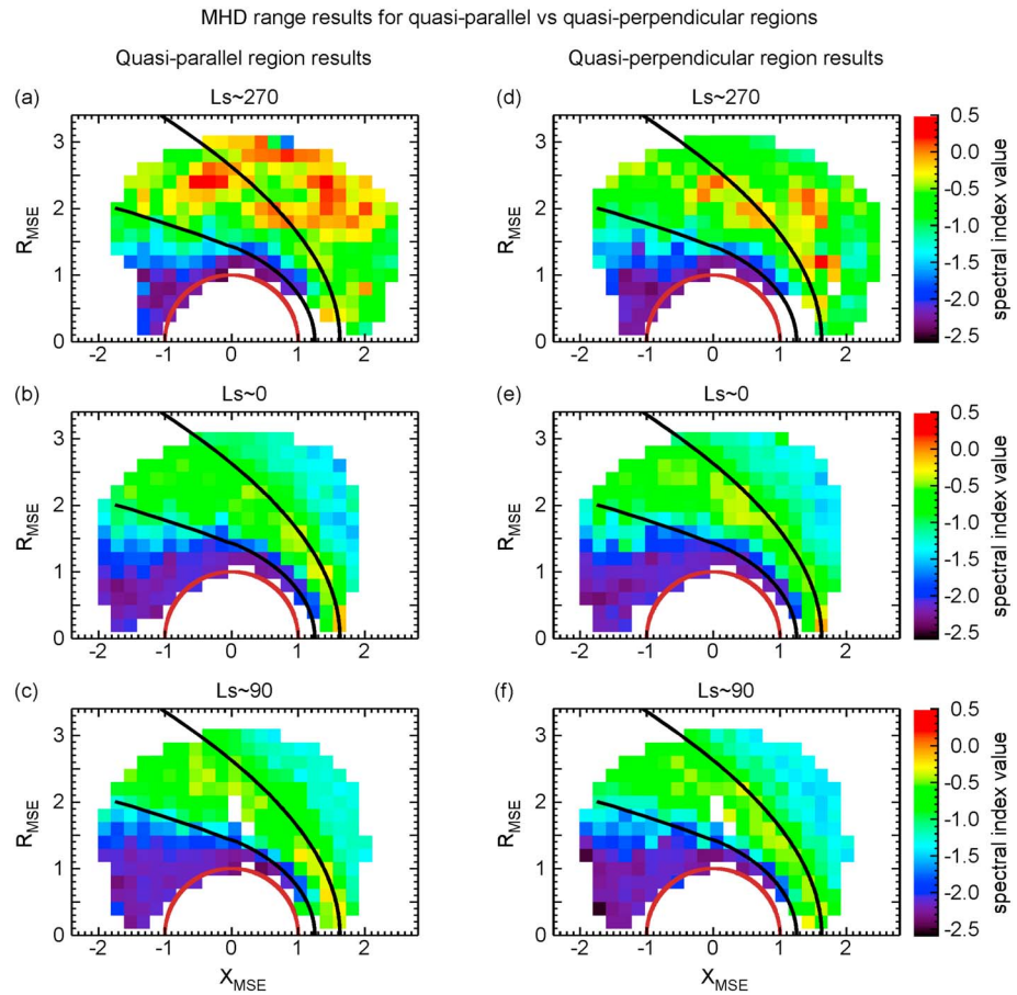
Figure 9. MHD range spectral indices in the magnetospheric hemispheres containing the quasi-parallel and the quasi-perpendicular shock regions. (a–c) Quasi-parallel region spectral indices plotted in X_{MSE} versus R_{MSE} = \sqrt{(Y_{MSE}^2 + Z_{MSE}^2)} maps for the three seasons. (d–f) Quasi-perpendicular region spectral indices plotted in X_{MSE} versus R_{MSE} maps. A prominent asymmetry for the spectral index values can be seen in the upstream region and in the magnetosheath for Ls \sim 270 .
