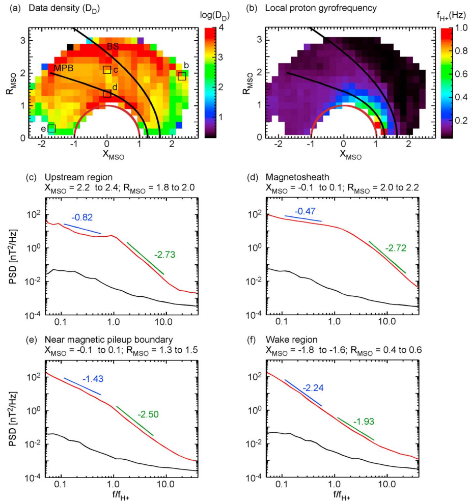
Figure 3. (a) MAVEN orbit coverage map showing data density D_D . (b) Median local proton gyrofrequency f_{H+} . (c–f) Median PSDs (shown in red) in four different regions of the Mars plasma environment indicated in Figure 3a by black squares. The black curves in Figures 3c–3f indicate the MAG noise level estimated by determining the minimum PSD for the magnetic field fluctuations measured by MAVEN when it was in the solar wind upstream of the bow shock. The spectral indices in the low- and high-frequency ranges (shown by a blue and a green line, respectively) have different values in different regions of the Mars plasma environment.
