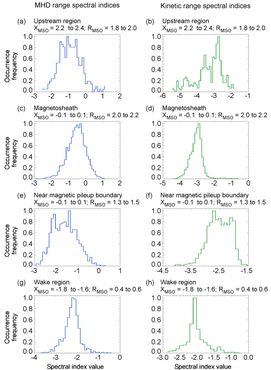
Figure 4. Histograms of spectral indices in the four different locations in the Mars plasma environment indicated in Figure 3a. (a and b) MHD and kinetic range spectral index histograms in the upstream region. (c and d) MHD and kinetic range spectral index histograms in the magnetosheath. (e and f) MHD and kinetic range spectral index histograms near the MPB. (g and h) MHD and kinetic range spectral index histograms in the wake.
