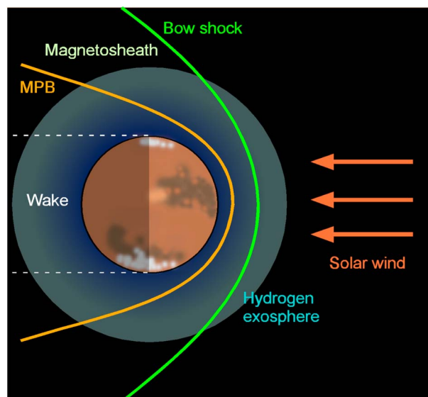
Figure 1. The Mars plasma environment. The bow shock separates the upstream solar wind from the magnetosheath. The magnetic pileup boundary separates the magnetosheath from the magnetic pileup region. The hydrogen exosphere, which extends beyond the bow shock of Mars, is also a crucial component in the Mars plasma environment.
