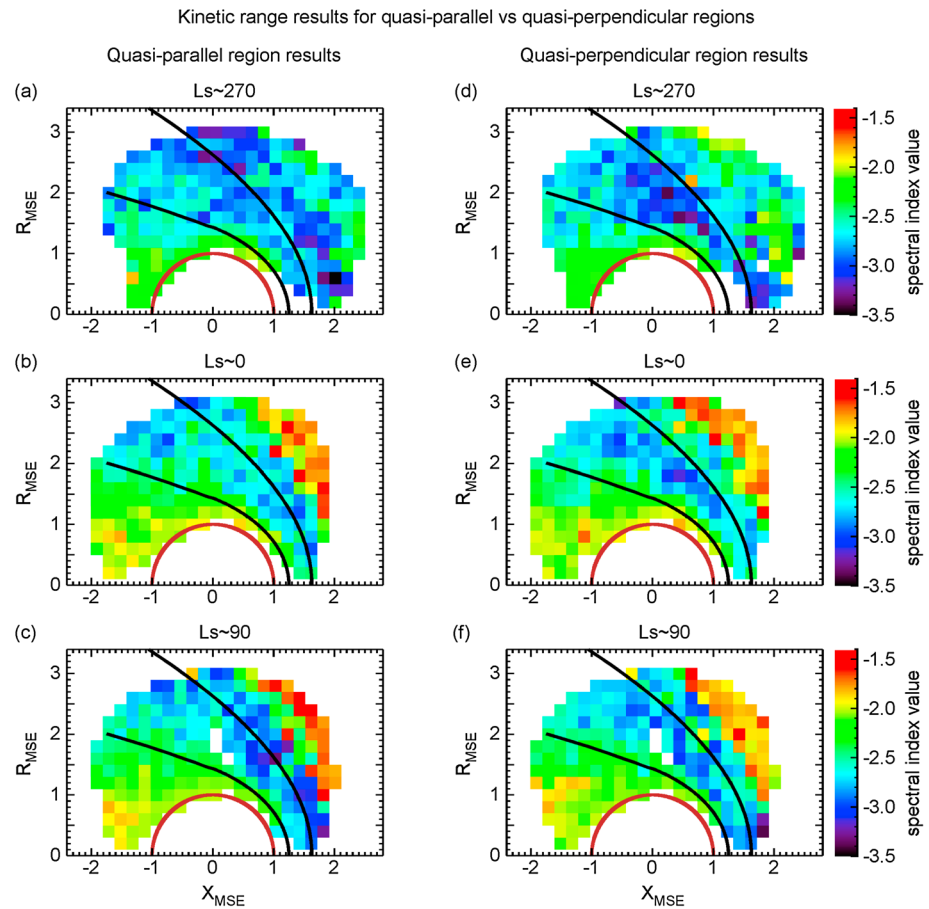
Figure 10. Kinetic range spectral indices in the magnetospheric hemispheres containing the quasi-parallel and quasi-perpendicular shock regions. (a–c) Quasi-parallel region spectral indices plotted in X_{MSE} versus R_{MSE} maps for the three seasons. (d–f) Quasi-perpendicular region spectral indices plotted in X_{MSE} versus R_{MSE} maps. An asymmetry is present for the spectral index values between the quasi-parallel and quasi-perpendicular regions for Ls \sim 270 .
