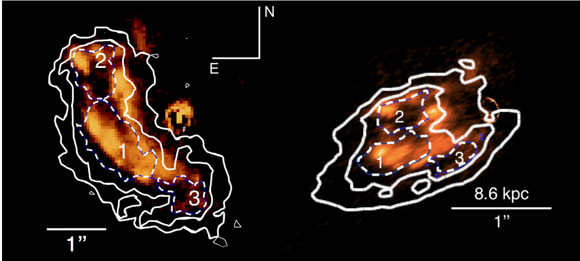
Fig. 1. HST/F814W images of A68-HLS115 in the image ( left panel ) and source plane after reconstruction ( right panel ). White dashed contours represent the H\alpha clumps and the white solid contours the H\alpha surface brightness measured in the image ( left panel ) and source plane ( right panel ) surface brightness maps corresponding to 0.64 and 1.28 \times 10^{-16} \text{ erg s}^{-1} \text{ cm}^{-2} \text{ arcsec}^{-2} . The surface brightness is conserved between the image and source plane. The cluster galaxy which is acting as a lens has been removed from the two images.
