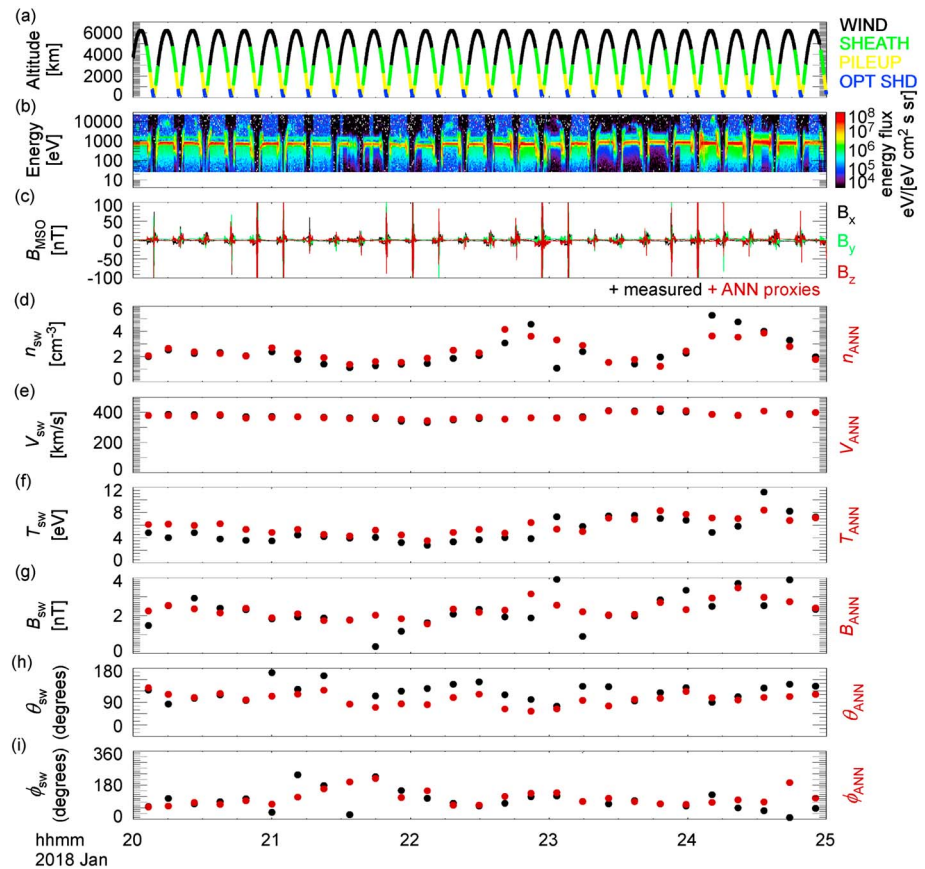
Figure 3. (a) Mars Atmosphere and Volatile EvolutioN spacecraft altitude with a color coding to indicate different regions in the Mars plasma environment. (b) A times stack of ion energy spectra from Solar Wind Ion Analyzer instrument which were used to determine the solar wind and sheath ion moments. (c) Time series of the three components of the magnetic field in Mars Solar Orbital coordinate system measured by the MAG instrument. (d–i) Measured versus ANN proxies for solar wind ion moments and IMF magnitude and orientations. The measured solar wind values are depicted in black, whereas the ANN proxies are depicted in red. Here n_{ANN} , V_{ANN} , T_{ANN} , B_{ANN} , \theta_{ANN} , and \phi_{ANN} denote ANN proxies for solar wind ion density, ion speed, ion temperature, IMF magnitude, IMF cone angle, and IMF clock angle, respectively. Each data point represents the orbit averages of the measured solar wind values and the ANN proxy values. ANN = artificial neural network; IMF = interplanetary magnetic field.
