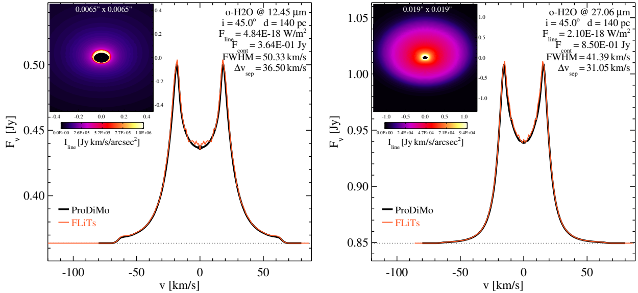
Fig. 1. Computation of high-resolution single line profiles with PRODiMo (black lines) and FLiTs (red lines) based on a medium-resolution 90×70 disc model. Left panel: o-H 2 O rotational line 13 6,5 → 12 4,9 at 12.453 μm with an excitation energy of 4213 K, which is emitted partly from the inner rim of the disc, and partly from the disc surface up to a radius of about 0.4 au in this model. Right panel: o-H 2 O rotational line 8 5,4 → 8 2,7 at 27.059 μm is depicted, which has an excitation energy of 1806 K and is mainly emitted from the disc surface up to a radius of about 1 au. The time consumption is about 92 CPU-sec with PRODiMo (251 velocity-channels, 356 × 144 rays) and 1.2 CPU-sec with FLiTs with enhanced accuracy settings (173 channels, 22375 rays), i.e. enhanced over FLiTs standards.
