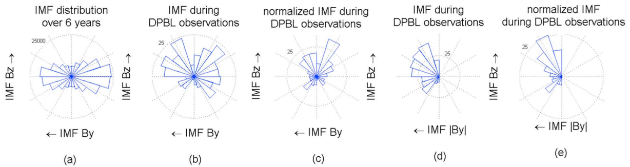
Figure 10. Interplanetary magnetic field (IMF) clock angle angular distributions for (a) all 6 years of observations, (b) during double population boundary layer (DPBL) events, and (c) the normalized distribution for DPBL events (i.e., [b] normalized to [a]). Panels (d) and (e) display the same distributions as (b) and (c) but only for the norm of the IMF B_y . Scales are given in each angular distribution with a number next to a circle of given radius.
