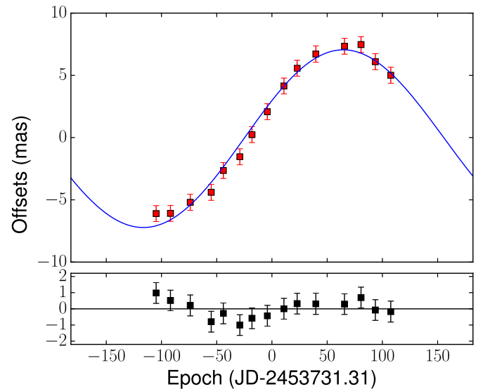
Fig. 6. Parallax fit to the mean positions of the shock front. Top: parallax sinusoid from the best fit to these data (blue line). The red squares are the mean positions of the shock front. In both cases, we have subtracted the proper motion and the RA position at JD 2453731.31 (the mean epoch from our observations) from the best fit. Bottom: residuals in right ascension.
