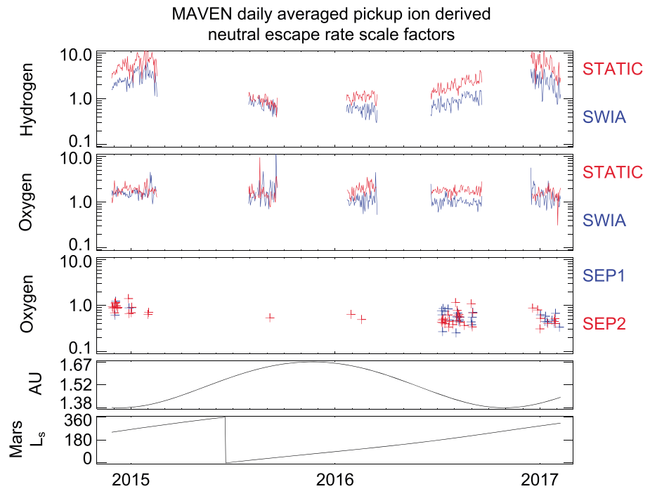
Figure 2. Daily averaged Solar Energetic Particle (SEP), Solar Wind Ion Analyzer (SWIA), and SupraThermal and Thermal Ion Composition (STATIC) derived neutral H and O escape rate scale factors along with Mars heliocentric distance and solar longitude. The scale factors are calculated by taking the ratio between the measured and modeled flux of pickup ions, indicating by how much the assumed input neutral density profiles and therefore the neutral escape rates need to be adjusted to match the data. MAVEN = Mars Atmosphere and Volatile Evolution. AU = Astronomical Unit.
