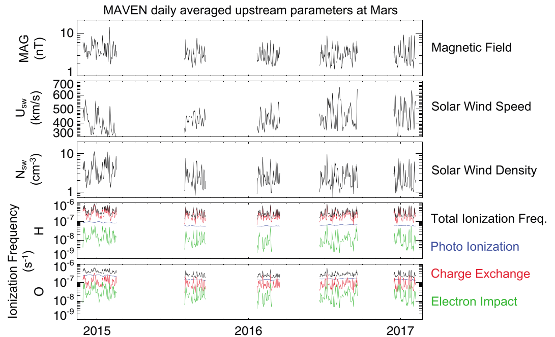
Figure 1. Daily averaged Mars Atmosphere and Volatile Evolution (MAVEN) measured upstream magnetic field magnitude, solar wind speed, and solar wind density at Mars, along with calculated hydrogen and oxygen ionization frequencies. Charge exchange by solar wind protons and photoionization are the dominant ionization mechanisms for H and O, respectively. Solar wind electron impact is a minor ionization process for both species. The periods with no upstream data are for when no part of MAVEN's orbit was sampling the solar wind.
