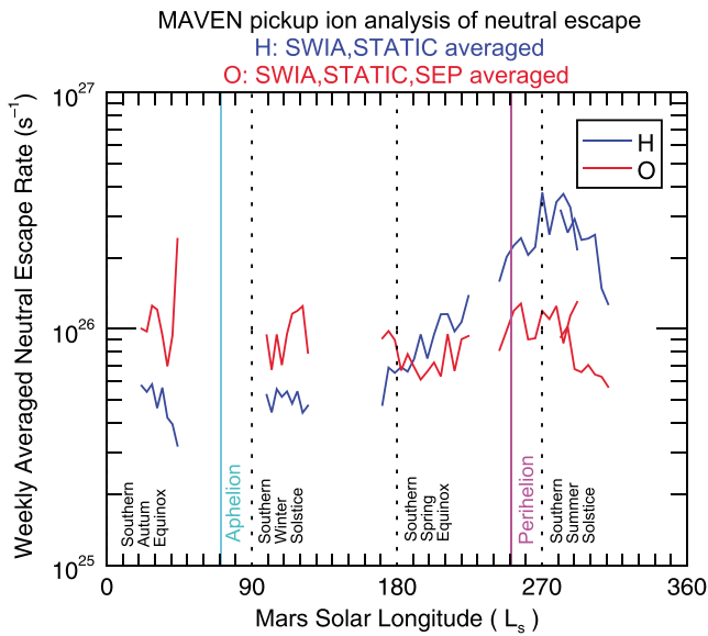
Figure 3. Seasonal variation of neutral H and O escape rates as derived from Mars Atmosphere and Volatile EvolutionN (MAVEN) pickup H^+ and O^+ observations. The escape rates are weekly averaged over Solar Wind Ion Analyzer (SWIA) and SupraThermal and Thermal Ion Composition (STATIC) for H and over SWIA, STATIC, SEP1, and SEP2 for O. The location of aphelion and perihelion along with Mars seasons are also included. A factor of 10 variation in H escape rate is observed, whereas O escape rate remains steadier. SEP = Solar Energetic Particle.
