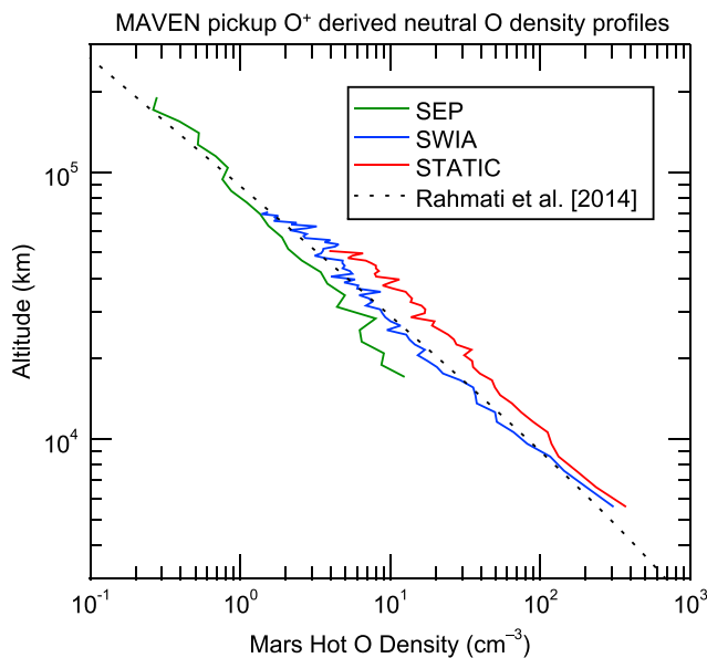
Figure 4. Hot oxygen density profiles derived from Solar Energetic Particle (SEP), Solar Wind Ion Analyzer (SWIA), and SupraThermal and Thermal Ion Composition (STATIC) pickup O^+ measurements by back-tracing the pickup ions to their ionization point in the exosphere. The hot O exospheric density profile of Rahmati et al. (2014) is included for comparison. The factor of 3 disagreement between the densities is most likely due to the lack of reliable calibration between the three instruments for pickup ion detection. MAVEN = Mars Atmosphere and Volatile EvolutionN.
