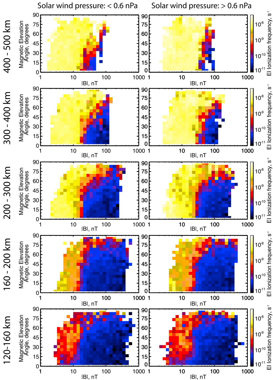
Figure 11. Mean electron impact ionization frequency is binned as a function of in situ measured magnetic field strength and elevation angle, separately by altitude range (rows: 120–160, 160–200, 200–300, 300–400, and 400–500 km) and solar wind pressure (columns: <math>< 0.6 \text{ nPa}</math> and <math>> 0.6 \text{ nPa}</math>), for SZA > 115° and with the same color scale as shown in Figure 6. Note that 0° elevation angle corresponds to local horizontal and 90° elevation angle to local vertical. SZA = solar zenith angle.
