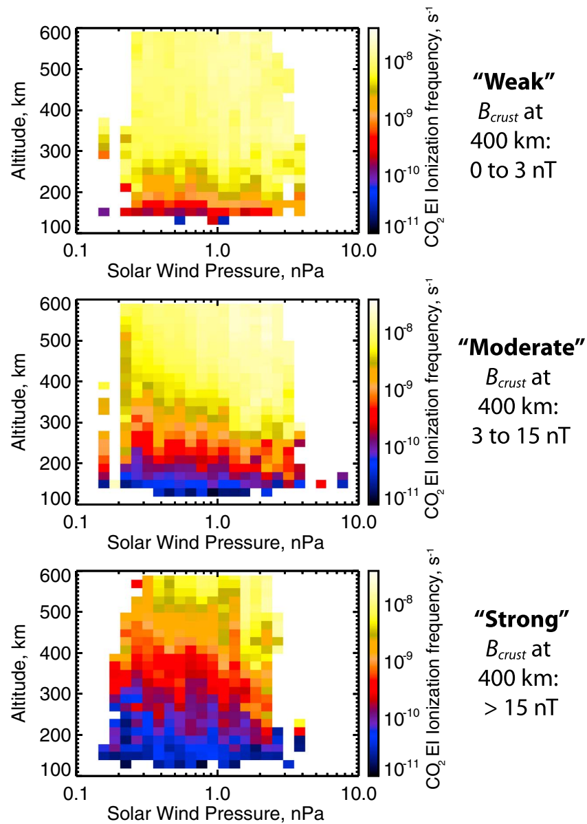
Figure 7. \text{CO}_2 electron impact ionization frequency is plotted as a function of altitude and solar wind pressure, for \text{SZA} > 115^\circ , for the same three ranges of regional crustal magnetic field strength, and with the same color scale, as shown in Figure 6. \text{SZA} = solar zenith angle.
