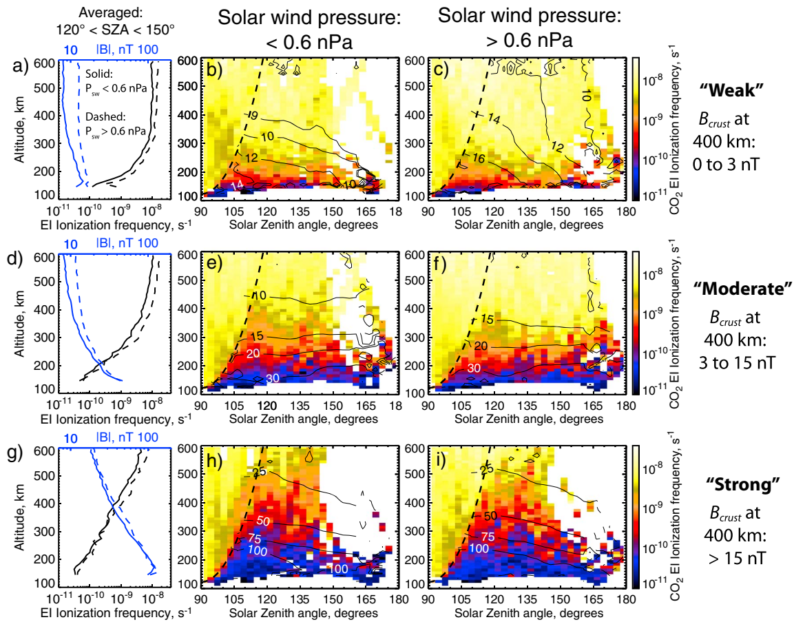
Figure 6. CO 2 electron impact ionization frequency is binned as a function of solar zenith angle (SZA) and altitude. The six color panels show the same data as Figure 4 but in coarser bins (3° in SZA and 10 km in altitude) and divided up by the strength of the crustal magnetic field at 400 km above or below each measurement at the same geographic location (rows: 0–3, 3–15, and >15 nT per the model of Morschhauser et al., 2014) and solar wind pressure (columns: <0.6 and >0.6 nPa). Thin labeled contours are average magnetic field values measured in situ. The associated line plots in the left-hand column show EIIIF (black) and in situ magnetic field strength (blue) averaged over 120° < SZA < 150°, for solar wind pressures below (solid) and above (dashed) 0.6 nPa.
