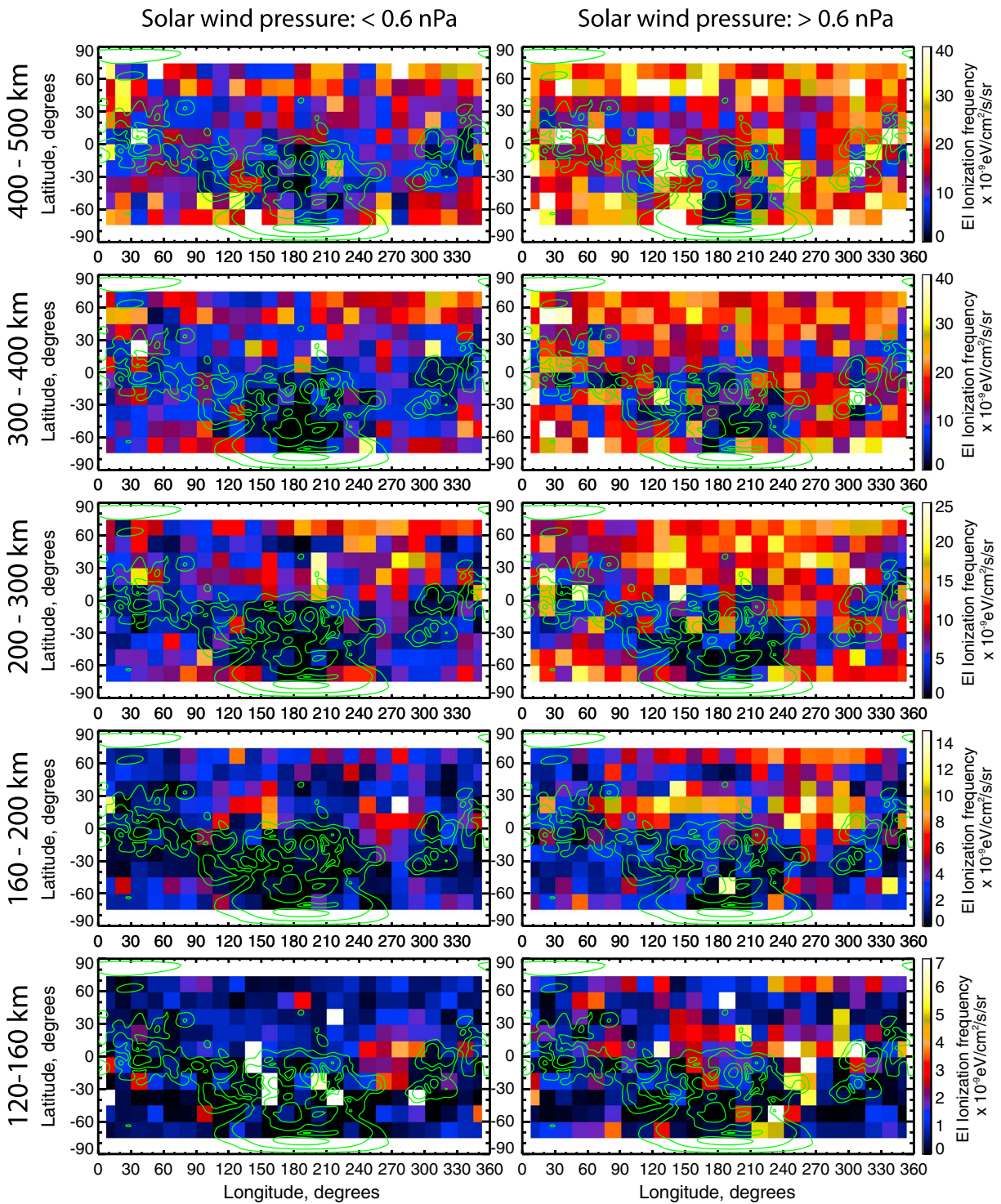
Figure 9. Mean electron impact ionization frequency is plotted in 15° bins of latitude and longitude for SZA >115°, separately by altitude range (rows: 120–160, 160–200, 200–300, 300–400, 400–500 km) and solar wind pressure (columns: <0.6 and >0.6 nPa). Overplotted in green is crustal magnetic field magnitude at 400 km per the model of Morschhauser et al. (2014), in contours of 10, 20, 50, and 100 nT. Note the color scale is not logarithmic and is different for each altitude range to bring out the geographic pattern of electron fluxes. SZA = solar zenith angle.
