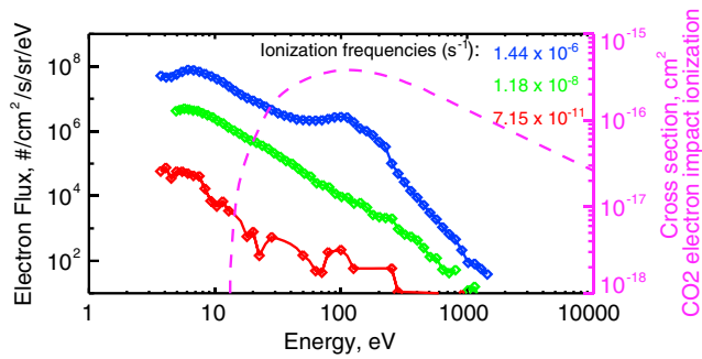
Figure 1. Example calculation of electron impact ionization frequency producing \text{CO}_2^+ ions. Blue, green, and red are three typical electron flux spectra seen on the Martian nightside. Electron impact ionization frequency is the integral over energy of the product of these spectra with the cross section (pink).
