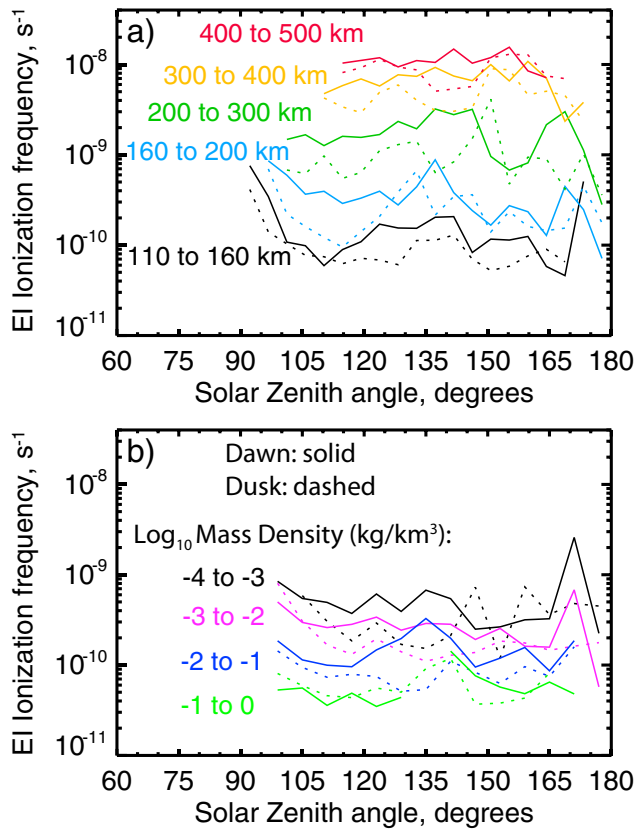
Figure 5. CO 2 electron impact ionization frequency as a function of solar zenith angle is plotted separately for dawn (solid lines) and dusk (dashed lines), for five different altitude ranges (colors, top panel) and four different mass density ranges (colors, bottom panel).
