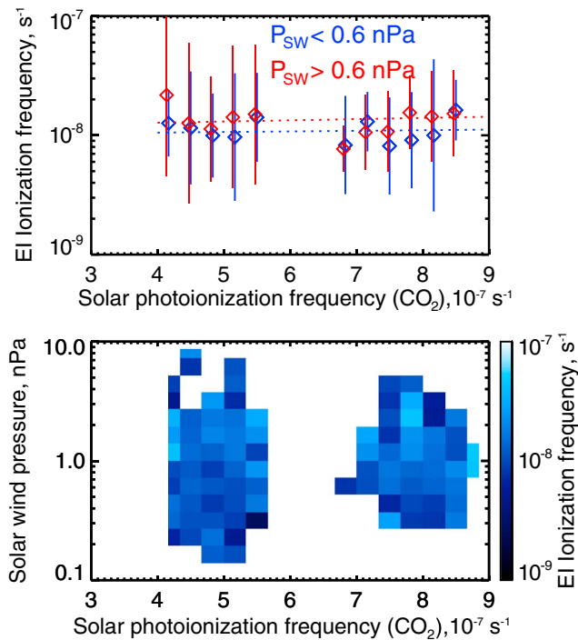
Figure 10. Dependence of “unperturbed” electron impact ionization frequency, that is, collected above 350-km altitude where crustal fields are weak ( B_{crust} at 400 km < 3 nT, as in Figures 6a–6c and Figure 7a) on solar wind pressure and CO_2 solar photoionization frequency. Panel (a) shows binned averages for high ( >0.6 nPa) and low ( <0.6 nPa) solar wind pressures with standard deviations, along with linear fits to the full dataset. Panel (b) shows a color plot of binned averages as a function of both solar photoionization frequency and solar wind pressure.
