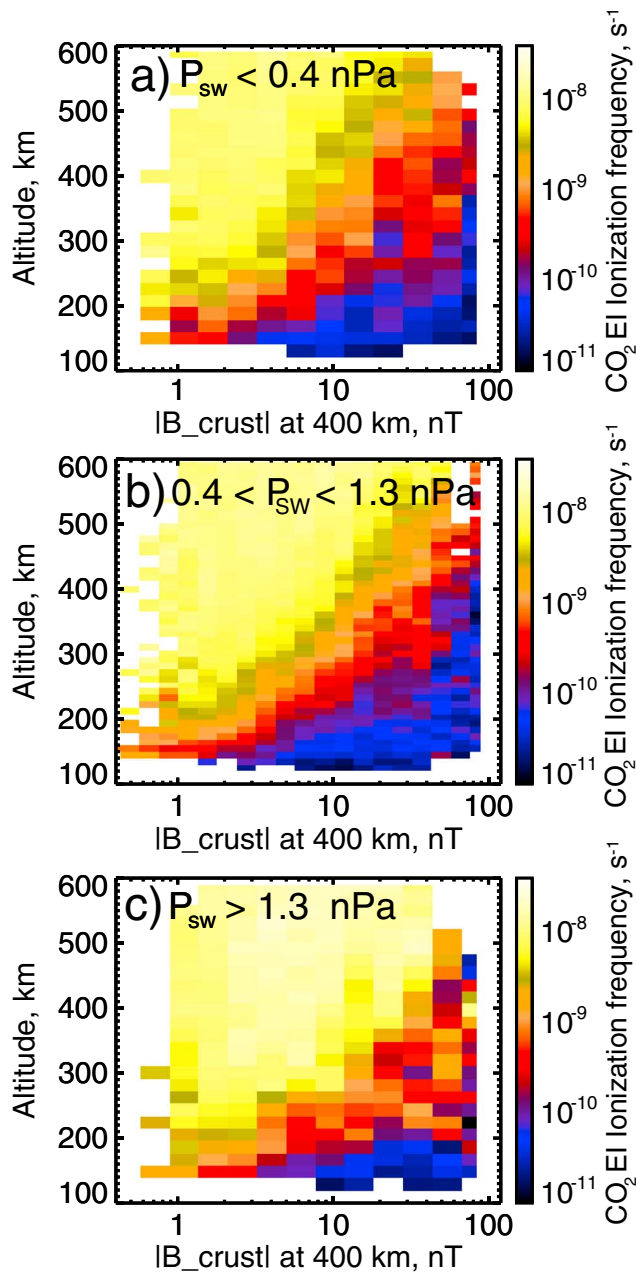
Figure 8. CO 2 electron impact ionization frequency is binned as a function of altitude and crustal magnetic field strength at 400 km (i.e., above or below each measurement at the same latitude/longitude) per the model of Morschhauser et al. (2014) for SZA > 115° for three separate ranges of solar wind pressure (<0.4, 0.4–1.3, and >1.3 nPa), and with the same color scale as shown in Figure 6. The resolution in each panel is determined by the number of available data points. SZA = solar zenith angle.
