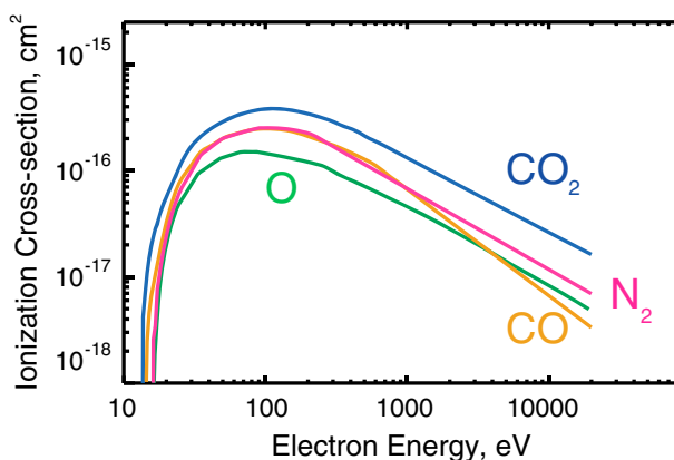
Figure 2. Electron impact ionization cross sections are plotted as a function of energy for the four major Martian thermospheric neutral species (Sung & Fox, 2000).
