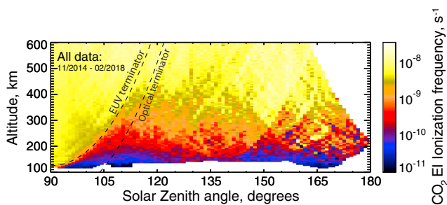
Figure 4. \text{CO}_2 electron impact ionization frequency on the Martian nightside, measured between 1 November 2014 and 1 February 2018, binned as a function of solar zenith angle ( 1^\circ bins) and altitude (5-km bins). The black dotted and dashed lines are the optical and extreme ultraviolet terminators (assuming a spherical planet with Mars’ mean radius of 3,389.9 and 3,389.9 + 122.5 km, respectively, Steckiewicz et al., 2017).
