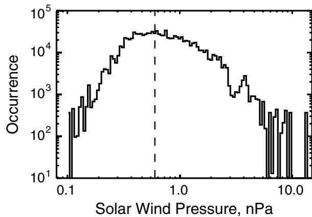
Figure 3. Histogram of all the solar wind pressure measurements made during this time, with the median (vertical dashed line) shown at 0.65 nPa.
