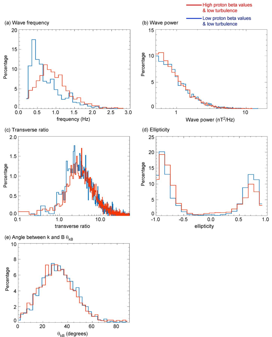
Figure 11. (a, e) Histograms of 1-Hz wave characteristics for low ( <0.6 ) and high ( >1.7 ) beta values under low turbulent conditions ( <1.2 nT 2 /Hz): frequency, power, transverse ratio, ellipticity, and the angle between the wave vector k and the magnetic field B , \theta_{kB} . The wave frequencies tend to be lower for the low proton beta values than for the high proton beta values.
