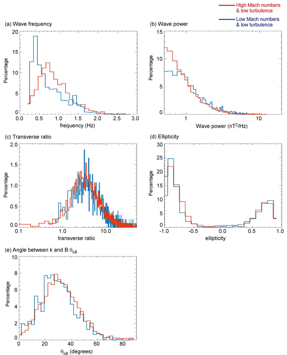
Figure 10. (a–e) Histograms of 1-Hz wave characteristics for low (<6.1) and high (>8.0) Mach numbers under low turbulent conditions (<1.2 nT 2 /Hz): frequency, power, transverse ratio, ellipticity, and the angle between the wave vector k and the magnetic field B , \theta_{kB} . The wave frequencies tend to be lower for the low Mach numbers than for the high Mach numbers.
