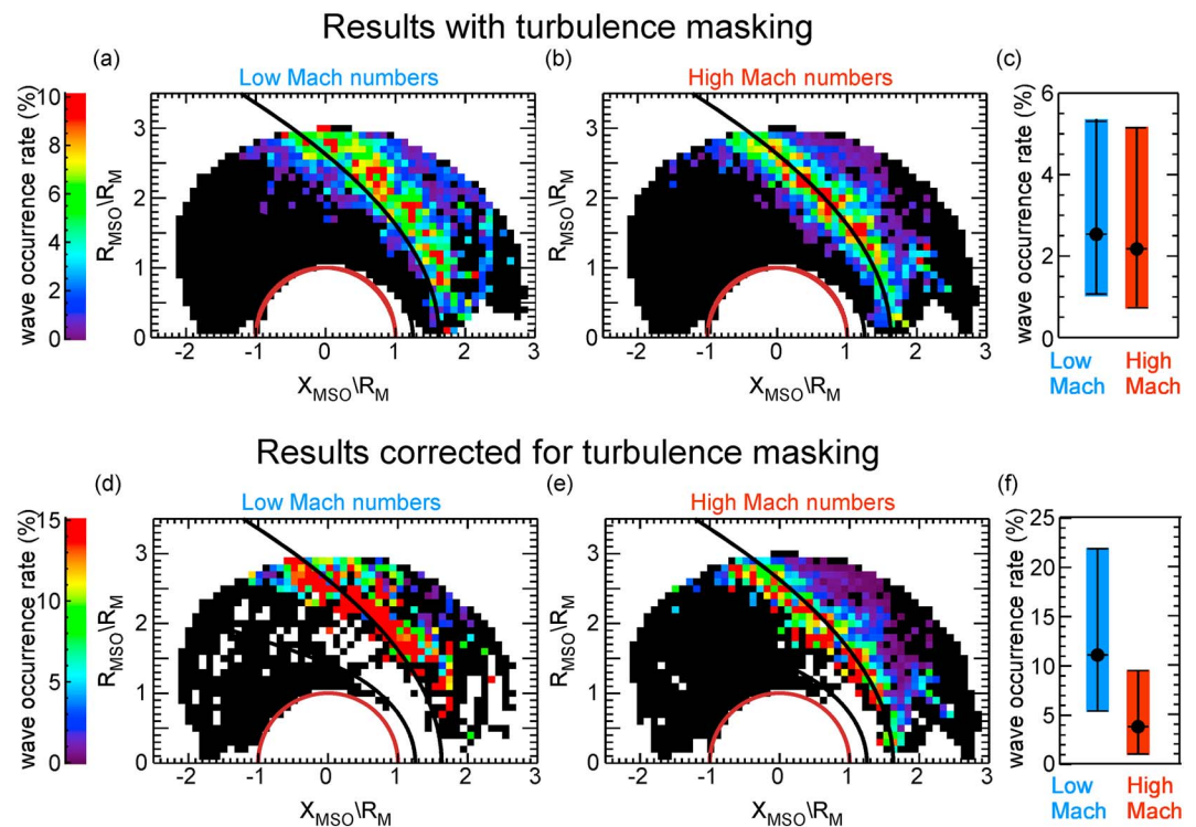
Figure 5. (a, b) Orbit maps for the 1-Hz wave occurrence rates for low ( <6.1 ) and high ( >8.0 ) magnetosonic Mach numbers. (c) Median wave occurrence rates and lower and upper quartiles for the low and high Mach numbers. (d, e) Orbit maps for the 1-Hz wave occurrence rates for low ( <6.1 ) and high ( >8.0 ) magnetosonic Mach numbers under the low turbulent conditions ( <1.2 \text{ nT}^2/\text{Hz} ). (f) Median wave occurrence rates and lower and upper quartiles for the low and high Mach numbers under the low turbulent conditions. Note that the results shown in (a)–(c) have not been corrected for turbulence masking effects, whereas results shown in (d)–(f) have been corrected for turbulence masking effects. The turbulence masking corrected results shown in (d)–(f) reveal that the wave occurrence rates are higher for the low Mach numbers than for the high Mach numbers. MSO = Mars Solar Orbital.
