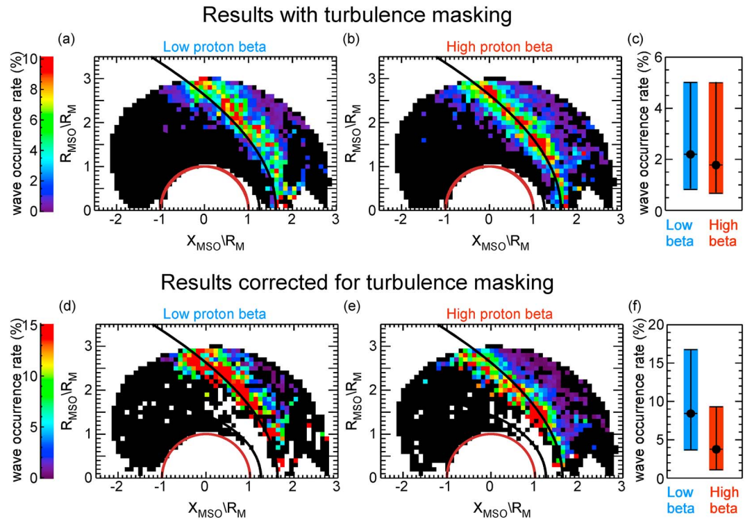
Figure 6. (a, b) Orbit maps for the 1-Hz wave occurrence rates for low ( <0.6 ) and high ( >1.7 ) proton beta values. (c) Median wave occurrence rates and lower and upper quartiles for the low and high proton beta values. (d, e) Orbit maps for the 1-Hz wave occurrence rates for low ( <0.6 ) and high ( >1.7 ) proton beta values under the low turbulent conditions ( <1.2 nT 2 /Hz). (f) Median wave occurrence rates and lower and upper quartiles for the low and high proton beta values under the low turbulent conditions. Note that the results shown in (a)–(c) have not been corrected for turbulence masking effects, whereas results shown in (d)–(f) have been corrected for turbulence masking effects. The turbulence masking corrected results shown in (d)–(f) reveal that the wave occurrence rates are higher for the low proton beta values than for the high proton beta values. MSO = Mars Solar Orbital.
