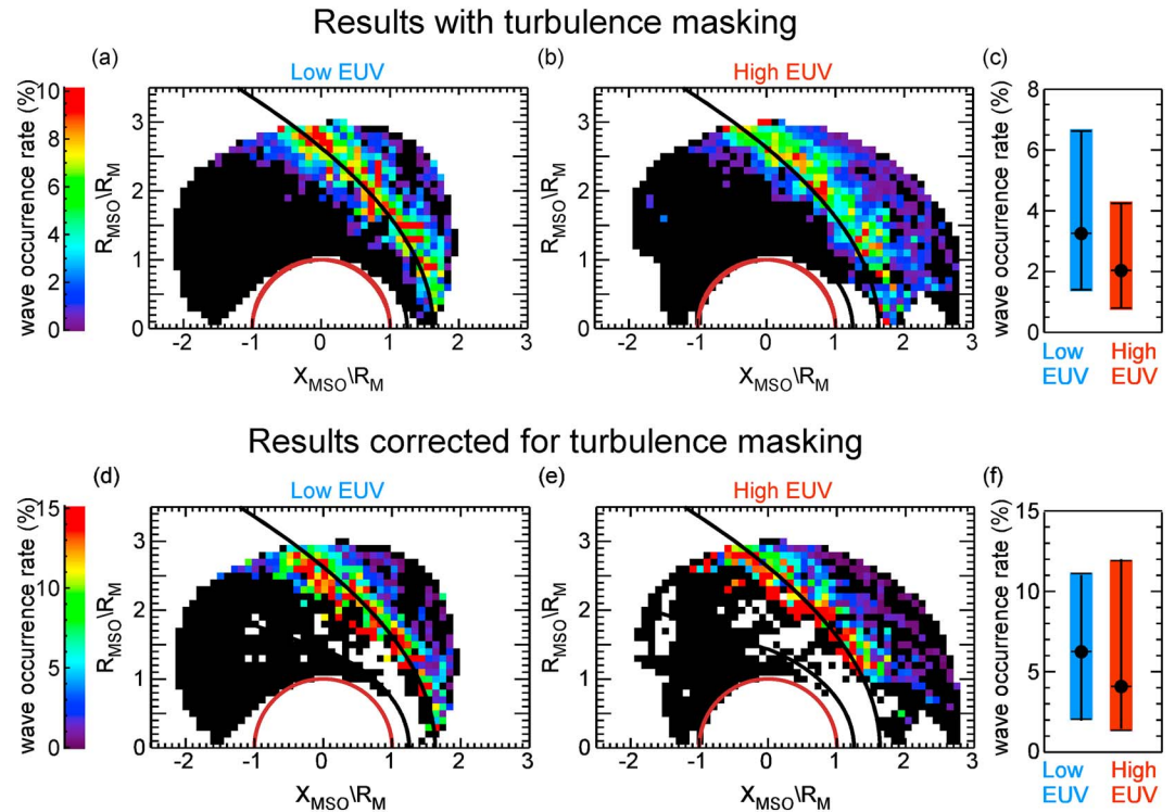
Figure 4. (a, b) Orbit maps for the 1-Hz wave occurrence rates for low ( <0.0027 \text{ W/m}^2 ) and high ( >0.0032 \text{ W/m}^2 ) extreme ultraviolet (EUV) flux levels. (c) Median wave occurrence rates and lower and upper quartiles for the low and high EUV flux levels. (d, e) Orbit maps for the 1-Hz wave occurrence rates for low ( <0.0027 \text{ W/m}^2 ) and high ( >0.0032 \text{ W/m}^2 ) EUV flux levels under low turbulent conditions ( <1.2 \text{ nT}^2/\text{Hz} ). (f) Median wave occurrence rates and lower and upper quartiles for the low and high EUV flux levels under the low turbulent conditions. Note that the results shown in (a)–(c) have not been corrected for turbulence masking effects, whereas results shown in (d)–(f) have been corrected for turbulence masking effects. The turbulence masking corrected results shown in (d)–(f) reveal that the wave occurrence rates do not vary significantly with the EUV flux levels. MSO = Mars Solar Orbital.
