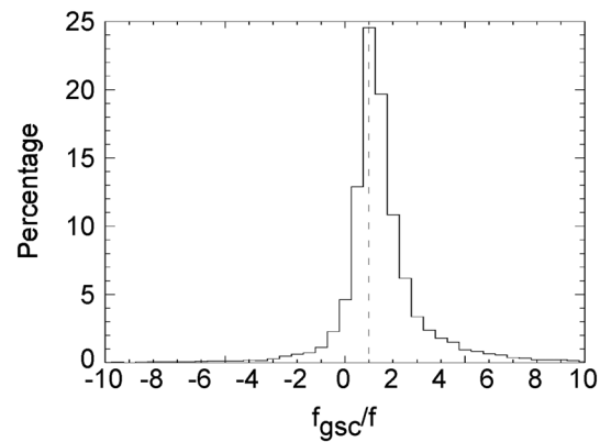
Figure 12. Histograms for the ratio of the group-standing frequency in the spacecraft frame f_{\text{gsc}} (= \omega_{\text{gsc}}/2\pi) to the wave frequency in the spacecraft frame f for 1-Hz waves at Mars under low turbulent conditions ( <1.2 \text{ nT}^2/\text{Hz} ). A high percentage of the waves have a ratio near 1 indicating that a large fraction of the 1-Hz waves at Mars satisfy the group-standing condition.
