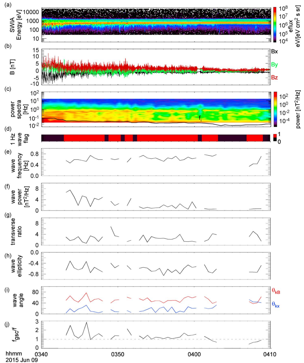
Figure 1. (a) Solar Wind Ion Analyzer energy spectrum shown to provide context for the wave observation. (b) Magnetic field time series. (c) Magnetic field power spectrum. (d) One-hertz wave flag which is the output of the automated search procedure for 1-Hz waves. Here time intervals corresponding to 1 or the red colored time intervals correspond to times where 1-Hz waves have been identified by the automated routine. (e–i) One-hertz wave parameters: frequency, power, transverse ratio, ellipticity, and wave angle. (j) The ratio of the group-standing frequency in the spacecraft frame f_{gsc}(= \omega_{gsc}/2\pi) to the wave frequency in the spacecraft frame f .
