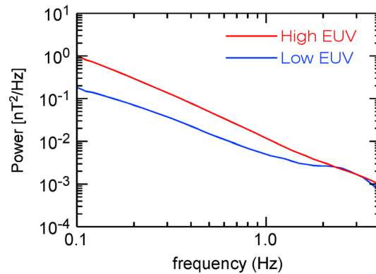
Figure 8. Median turbulence spectra for low ( <0.0027 \text{ W/m}^2 ) and high ( >0.0032 \text{ W/m}^2 ) extreme ultraviolet flux levels. The turbulent levels are high during the times of high extreme ultraviolet flux, enabling masking of the 1-Hz waves.
