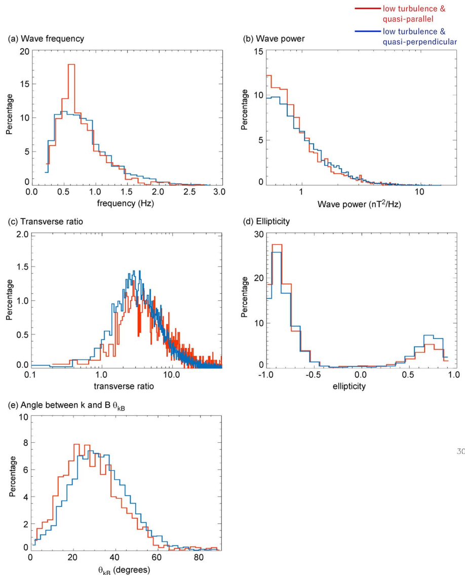
Figure 14. (a–e) Histograms of 1-Hz wave parameters for quasi-parallel and quasi-perpendicular regions under low turbulent conditions ( <1.2 \text{ nT}^2/\text{Hz} ): frequency, power, transverse ratio, ellipticity, and \theta_{kB} . The wave frequency distribution tends to be slightly broader in the quasi-perpendicular region than in the quasi-parallel region.
