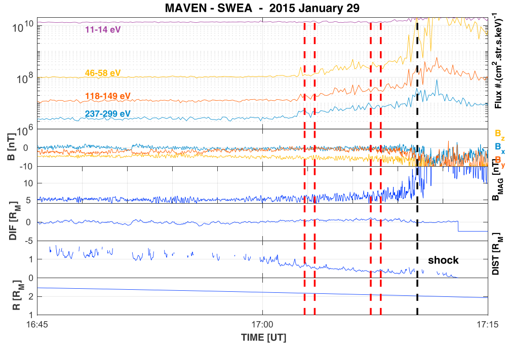
Figure 3. Same format as Figure 1 for 29 January 2015/1645–1715 UT time interval.
