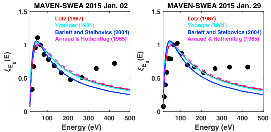
Figure 4. Black circles indicate \xi_{E_0}(E) ratio versus E with E_0 = 52.1 eV. The continuous lines show the ratio of HI-electron impact cross sections \frac{\sigma(E)}{\sigma(E_0)} from various sources.
