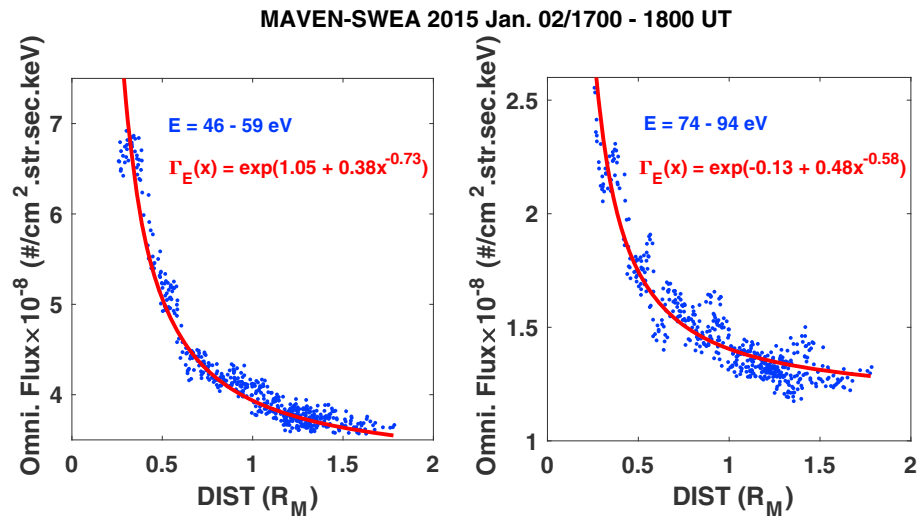
Figure 2. Scatter plot of electron flux versus DIST for two energy ranges. The continuous red curve represents the best fit with a function y = \exp(a + bx^{-\beta}) .
