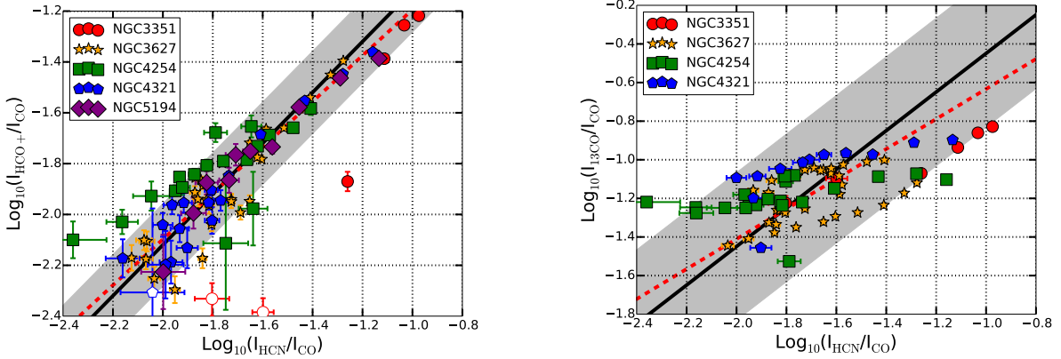
Figure 9. Line ratios for our radial profiles. ( Left ): I_{\text{HCO}^+}/I_{\text{CO}} as a function of I_{\text{HCN}}/I_{\text{CO}} . The black line shows the median \text{HCO}^+/\text{CO} ratio and its \pm 1\sigma range in our data. The gray shaded region illustrates the \pm 1\sigma range found by Privon et al. (2015) for luminous infrared galaxies. The two line ratios track one another, reinforcing that our results are not specific to HCN. There is some indication of a slightly sublinear slope to the I_{\text{HCO}^+}/I_{\text{CO}} vs I_{\text{HCN}}/I_{\text{CO}} relation, which would be expected for a lognormal distribution give the lower critical density of \text{HCO}^+ . ( Right ): ^{13}\text{CO}/\text{CO} as a function of I_{\text{HCN}}/I_{\text{CO}} . The black line shows the median ^{13}\text{CO}/\text{HCN} in our sample. The sublinear slope can be expected if the effective density for ^{13}\text{CO} emission lies below the median density by mass while HCN traces comparatively dense gas.
