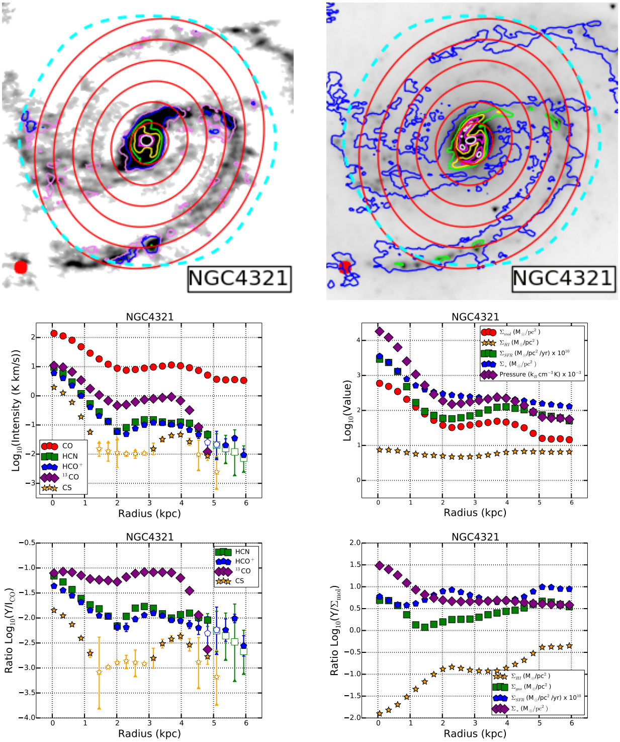
Figure 4. As Figure 1 but for NGC 4321.
