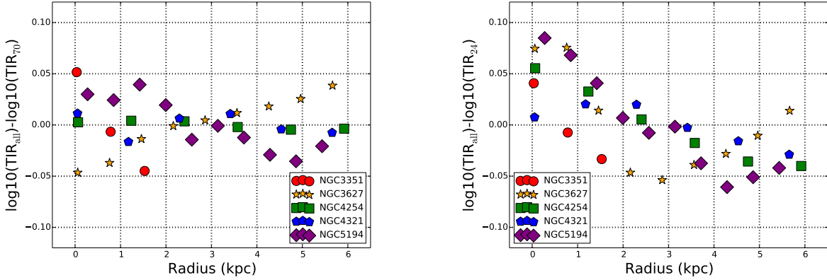
Figure 12. Residuals between \Sigma_{\text{TIR}} ( TIR ) calculated using all IR data and \Sigma_{\text{TIR}} predicted using only 70 \mu m ( TIR_{70} , left) or 24 \mu m ( TIR_{24} , right) following Equation A1 and Table 9. We show the logarithmic residual between the predicted and best-estimate TIR for each ring at 30'' resolution. The 70 \mu m-based prediction recovers the best-estimate TIR with \sim 0.05 dex ( \sim 12\% ) scatter and only modest residuals.
