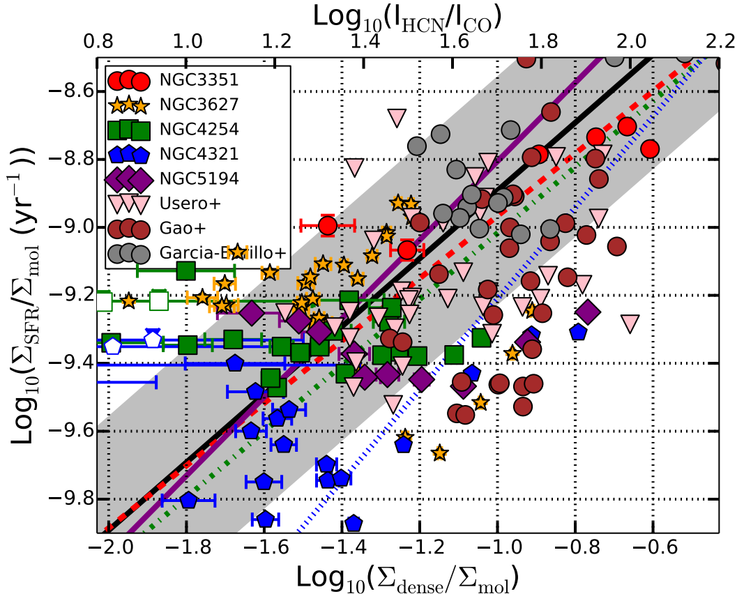
Figure 7. \Sigma_{SFR}/\Sigma_{mol} , or the normalized rate at which molecular gas forms stars, as a function of \Sigma_{dense}/\Sigma_{mol} , or the dense gas fraction as traced by I_{HCN}/I_{CO} . Higher dense gas fractions do correspond to more efficient star formation in the total molecular gas, but with large scatter, which we show below to be physical in nature. Lines show the median, best fit, and scatter for our survey along with the measurements of Gao & Solomon (2004), García-Burillo et al. (2012), and Usero et al. (2015). Statistically, the HCN/CO ratio is a relatively poor predictor of \Sigma_{SFR}/\Sigma_{mol} when all data are considered together, though it performs better in some individual galaxies or subsamples.
