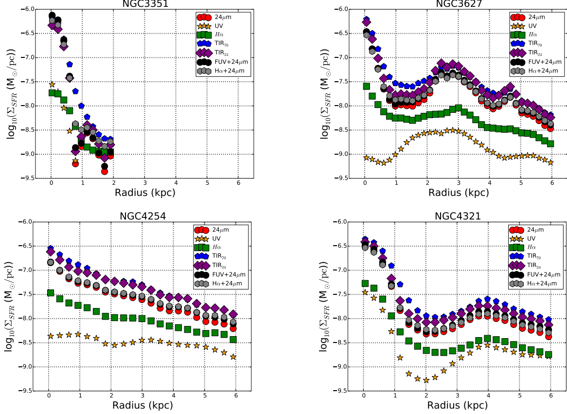
Figure 13. A comparison of the SFR as determined using only 24\mu\text{m} emission, only FUV emission, only \text{H}\alpha emission, only TIR emission, a combination of FUV and 24\mu\text{m} emission, and a combination of \text{H}\alpha and 24\mu\text{m} emission. We find that IR emission dominates significantly over FUV or \text{H}\alpha emission, indicating a high level of extinction.
