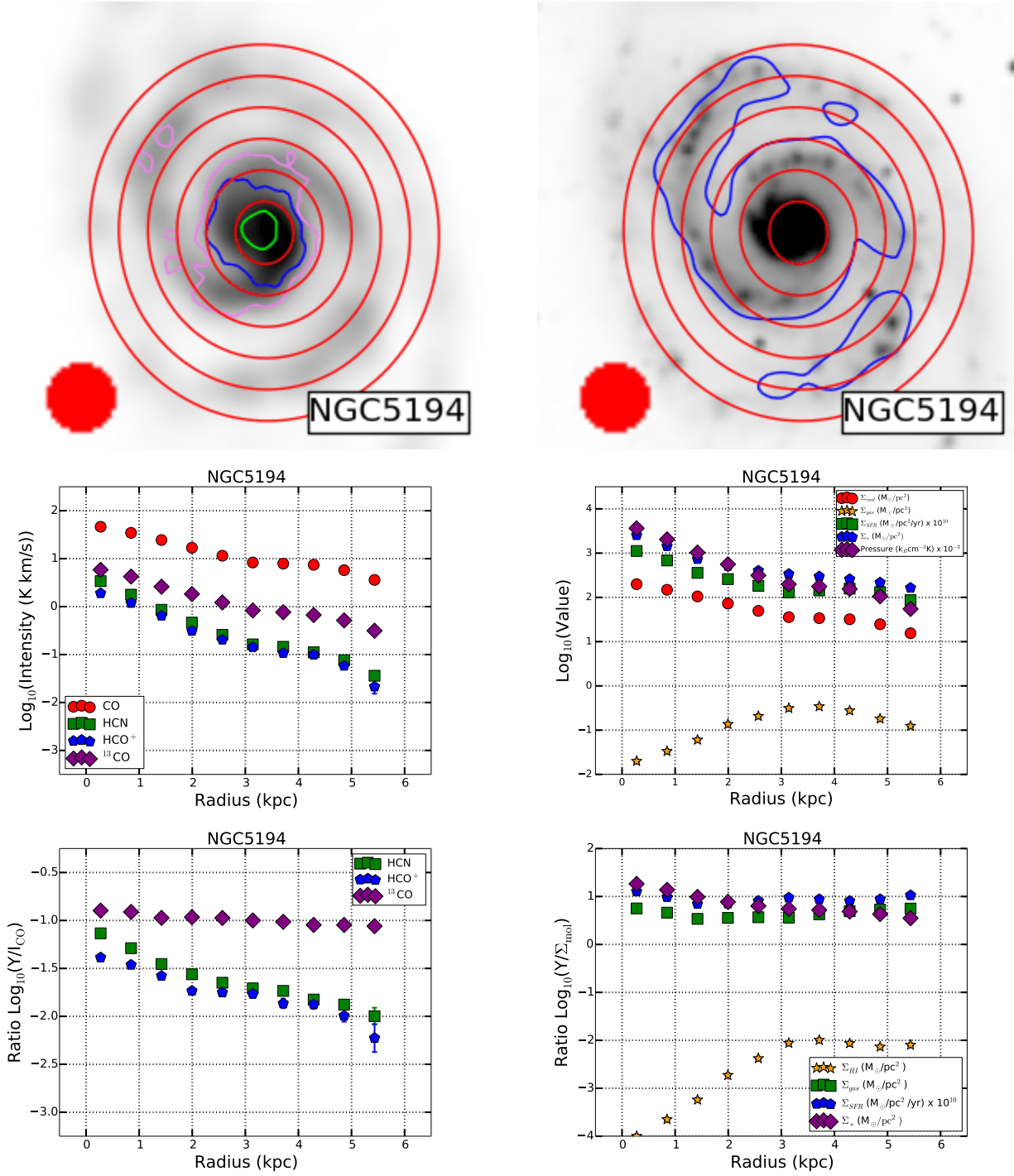
Figure 5. As Figure 1 but for NGC 5194, with data from the IRAM large program EMPIRE (Bigiel et al. 2016). Note that EMPIRE does not cover CS (2-1). Please note that the y-axis range for the two right hand panels are different for NGC 5194 than for the other 4 galaxies.
