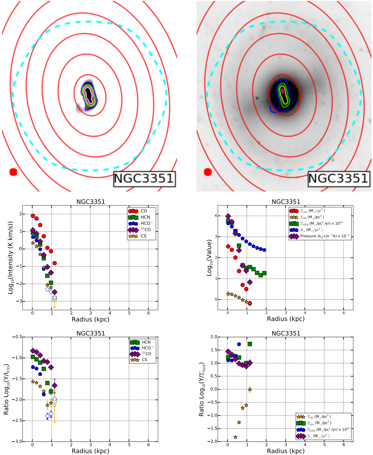
Figure 1. Our ALMA observations in context for NGC 3351. ( Top left: ) HCN contours (color) over CO integrated intensity (grayscale). HCN contours: show 0.5 (violet), 1 (blue), 3.5 (green), 6.5 (yellow), 9.5 (magenta), and 12.5 (white) K km s -1 . Red rings show fixed galactocentric radius in the plane of the galaxy, spaced by 1 kpc. The filled red circle in the lower left shows the common \theta = 8'' (FWHM) beam used in our analysis. The dashed cyan contour shows the ALMA field of view for HCN emission. ( Top right: ) 3.6μm map, tracing stellar structure, with CO integrated intensity contours at 10, 60, 110, 160, and 210 K km s -1 . ( Center left: ) Azimuthally averaged integrated intensity profiles for CO, HCN, CS, HCO + , and 13 CO (see §2.10), restricting the average to regions with statistically significant CO emission. Filled points have SNR ≥ 2. Error bars show uncertainty in the mean. Empty points indicate upper limits. ( Center right: ) Intensity profiles for tracers of galaxy and ISM structure: CO (tracing molecular gas), Hα and 24μm emission (tracing star formation), and contaminant-corrected 3.6μm emission (tracing stellar mass). ( Bottom left: ) Ratio of other lines to CO intensity as a function of radius. ( Bottom right: ) Ratios among tracers of galaxy and ISM structure, along with estimated dynamical equilibrium pressure. The radial profiles are available online as described in Appendix C.
