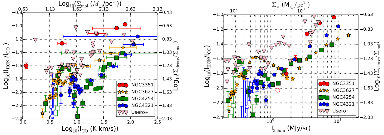
Figure 8. HCN/CO, tracing the dense gas fraction, as a function observable cognates of (left) molecular gas and (right) stellar surface density. The left panel shows HCN/CO as a function of mean molecular gas surface density, estimated from I_{\text{CO}} using a fixed conversion factor. The right panel shows HCN/CO as a function of stellar surface density, estimated from contaminant-corrected 3.6\mu\text{m} maps. In both cases, a higher overall surface density corresponds to a larger apparent dense gas fraction. The correlation with stellar surface density is particularly striking (as in Usero et al. 2015 ).
