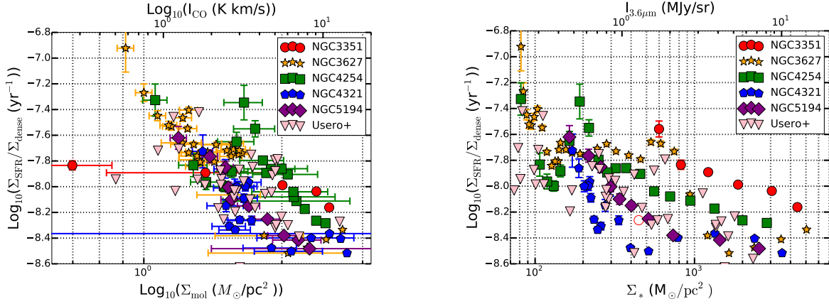
Figure 10. \Sigma_{SFR}/\Sigma_{dense} , or the star formation efficiency of dense gas, as a function of tracers of the molecular gas (left) and stellar (right) surface density. \Sigma_{SFR}/\Sigma_{dense} anti-correlates with \Sigma_{mol} , traced by I_{CO} , and with \Sigma_{*} , as traced by contaminant-corrected 3.6\mu m intensity. Thus dense gas appears less efficient at star formation at high surface densities. The primary axes adopt our fiducial translations to physical quantities and report the molecular gas or stellar surface density ( x ) and the star formation efficiency of dense gas ( SFR/M_{dense} ). The alternate axes present the observational data.
