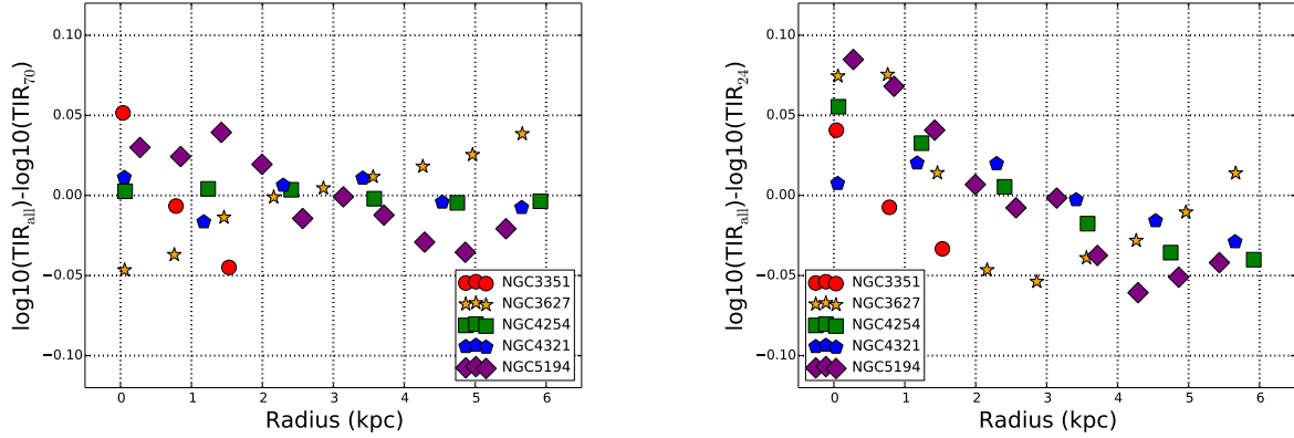
Figure 12. Residuals between \Sigma_{\text{TIR}} (TIR) calculated using all IR data and \Sigma_{\text{TIR}} predicted using only 70 \mu m ( TIR_{70} , left) or 24 \mu m ( TIR_{24} , right) following Equation A1 and Table 9. We show the logarithmic residual between the predicted and best-estimate TIR for each ring at 30'' resolution. The 70 \mu m-based prediction recovers the best-estimate TIR with \sim 0.05 dex ( \sim 12\% ) scatter and only modest residuals.
