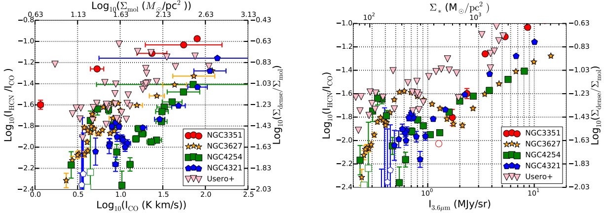
Figure 8. HCN/CO, tracing the dense gas fraction, as a function observable cognates of ( left ) molecular gas and ( right ) stellar surface density. The left panel shows HCN/CO as a function of mean molecular gas surface density, estimated from I_{\text{CO}} using a fixed conversion factor. The right panel shows HCN/CO as a function of stellar surface density, estimated from contaminant-corrected 3.6\mu\text{m} maps. In both cases, a higher overall surface density corresponds to a larger apparent dense gas fraction. The correlation with stellar surface density is particularly striking (as in Usero et al. 2015 ).
