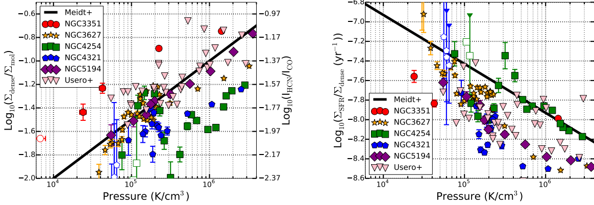
Figure 11. (Left:) I_{\text{HCN}}/I_{\text{CO}} , tracing dense gas fraction, and (right) \Sigma_{\text{SFR}}/\Sigma_{\text{dense}} , or the star formation efficiency of dense gas, both as a function of dynamical equilibrium pressure calculated following Equation 7. Regions where high P_{\text{DE}} is needed to sustain the weight of the gas have high dense gas fractions but apparently low dense gas star formation efficiencies. This is consistent with the idea that the mean cloud density reflects the large scale environment and that the role of any particular density in star formation (here the density needed to emit HCN) depends on the environment. Gas of a particular density appears to be less efficient in regions of high mean density. The black lines are model predictions from Meidt (2016).
