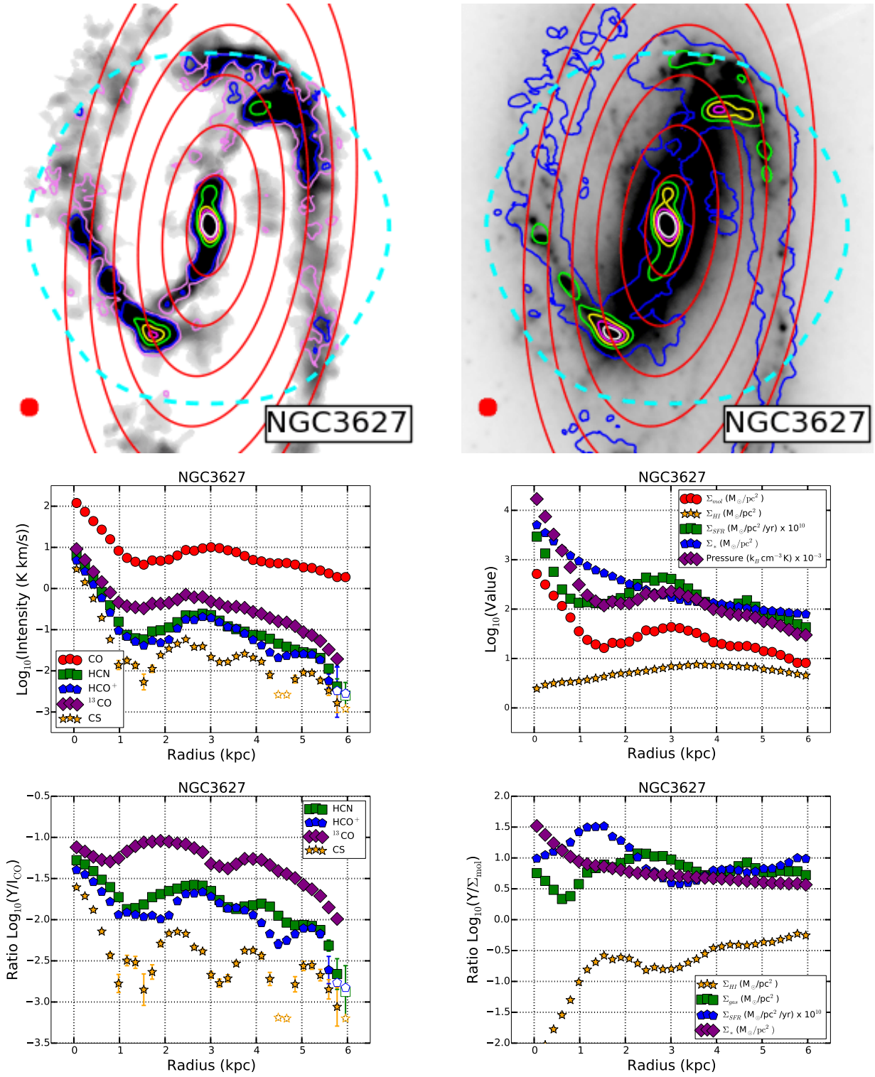
Figure 2. As Figure 1 but for NGC 3627.
