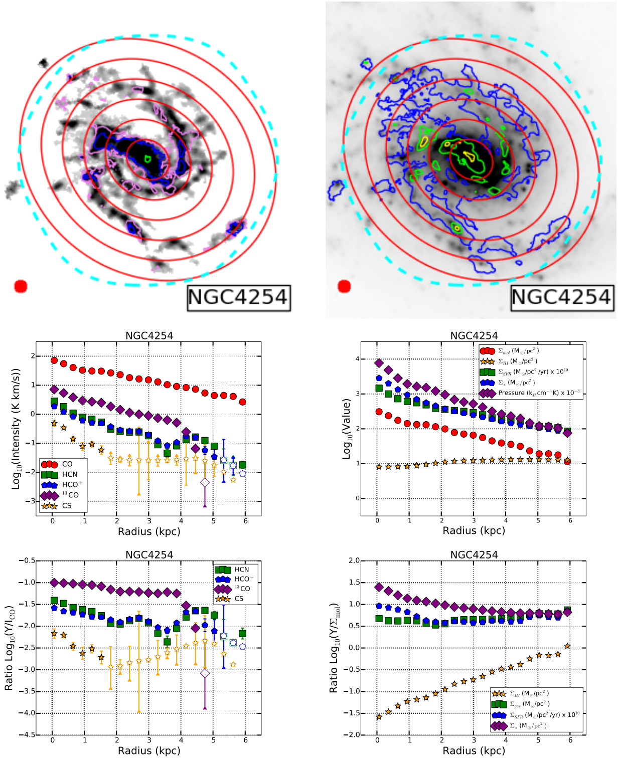
Figure 3. As Figure 1 but for NGC 4254.
