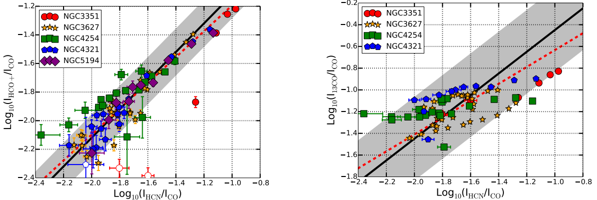
Figure 9. Line ratios for our radial profiles. ( Left ): I_{\text{HCO}^+}/I_{\text{CO}} as a function of I_{\text{HCN}}/I_{\text{CO}} . The black line shows the median \text{HCO}^+/\text{HCN} ratio and its \pm 1\sigma range in our data. The gray shaded region illustrates the \pm 1\sigma range found by Privon et al. (2015) for luminous infrared galaxies. The two line ratios track one another, reinforcing that our results are not specific to HCN. There is some indication of a slightly sublinear slope to the I_{\text{HCO}^+}/I_{\text{CO}} vs I_{\text{HCN}}/I_{\text{CO}} relation, which would be expected for a lognormal distribution give the lower critical density of \text{HCO}^+ . ( Right ): ^{13}\text{CO}/\text{CO} as a function of I_{\text{HCN}}/I_{\text{CO}} . The black line shows the median ^{13}\text{CO}/\text{HCN} in our sample. The sublinear slope can be expected if the effective density for ^{13}\text{CO} emission lies below the median density by mass while HCN traces comparatively dense gas.
