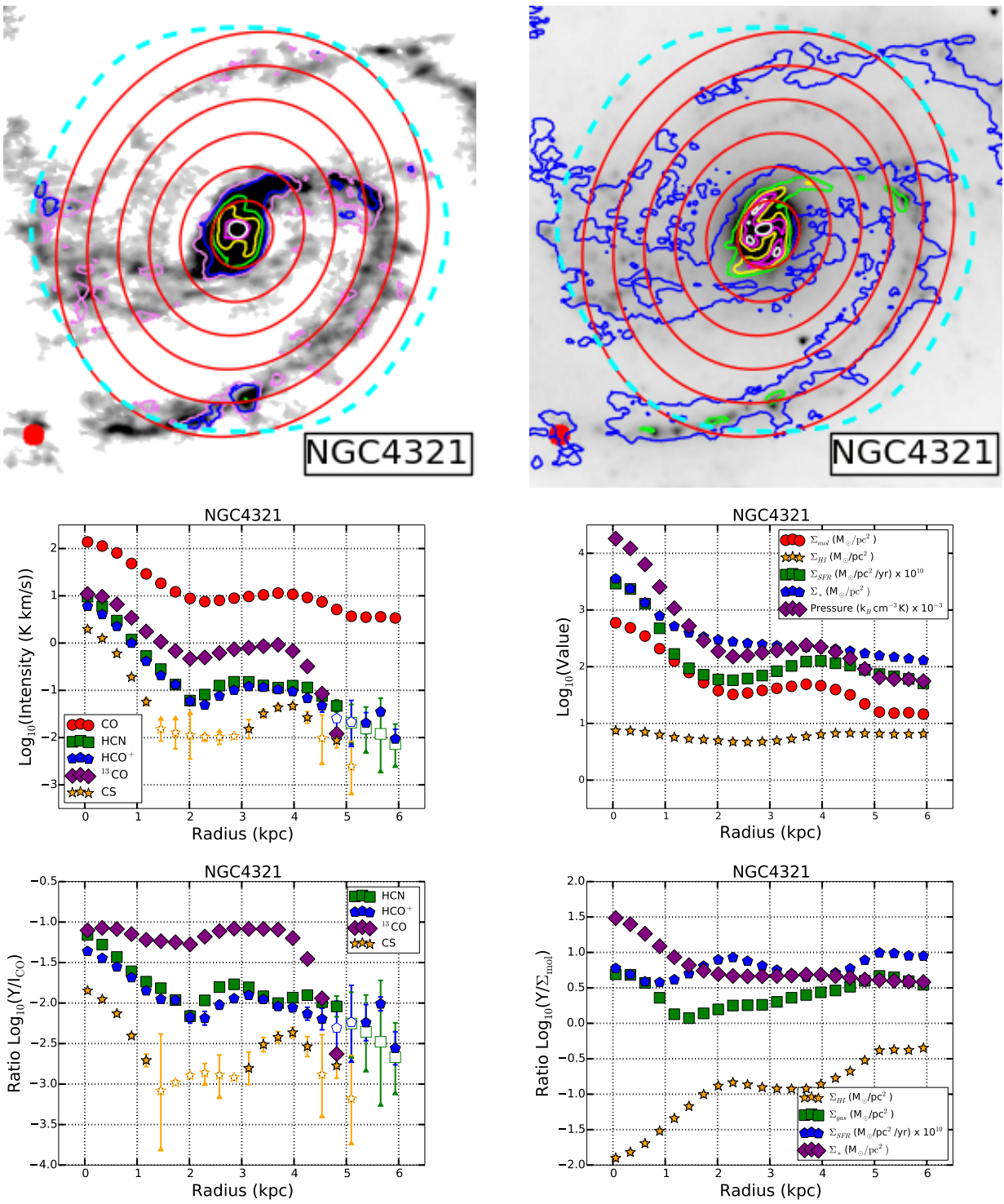
Figure 4. As Figure 1 but for NGC 4321.
