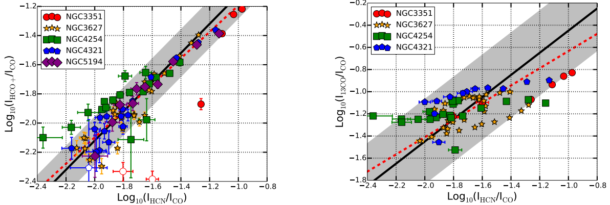
Figure 9. Line ratios for our radial profiles. (Left:) I_{\text{HCO}^+}/I_{\text{CO}} as a function of I_{\text{HCN}}/I_{\text{CO}} . The black line shows the median \text{HCO}^+/\text{HCN} ratio and its \pm 1\sigma range in our data. The gray shaded region illustrates the \pm 1\sigma range found by Privon et al. (2015) for luminous infrared galaxies. The two line ratios track one another, reinforcing that our results are not specific to HCN. There is some indication of a slightly sublinear slope to the I_{\text{HCO}^+}/I_{\text{CO}} vs I_{\text{HCN}}/I_{\text{CO}} relation, which would be expected for a lognormal distribution give the lower critical density of \text{HCO}^+ . (Right:) ^{13}\text{CO}/\text{CO} as a function of I_{\text{HCN}}/I_{\text{CO}} . The black line shows the median ^{13}\text{CO}/\text{HCN} in our sample. The sublinear slope can be expected if the effective density for ^{13}\text{CO} emission lies below the median density by mass while HCN traces comparatively dense gas.
