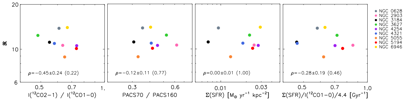
Figure 3. Correlation between the ^{12}\text{CO}(1-0) -to- ^{13}\text{CO}(1-0) intensity ratio, \mathfrak{R} , and several quantities: the ^{12}\text{CO}(2-1)/^{12}\text{CO}(1-0) ratio probing the gas physical conditions, the PACS70/PACS160 flux density ratio probing the dust temperature, \Sigma_{\text{SFR}} , and the \Sigma_{\text{SFR}}/\text{CO}(1-0) ratio which is a proxy for the SFE. Quantities are averaged over entire galaxies and do not show significant correlations. Uncertainties on the galaxy averages are plotted but smaller than the symbol sizes. We also indicate the Spearman’s rank correlation coefficients, their uncertainty, and their significance (in parenthesis).
