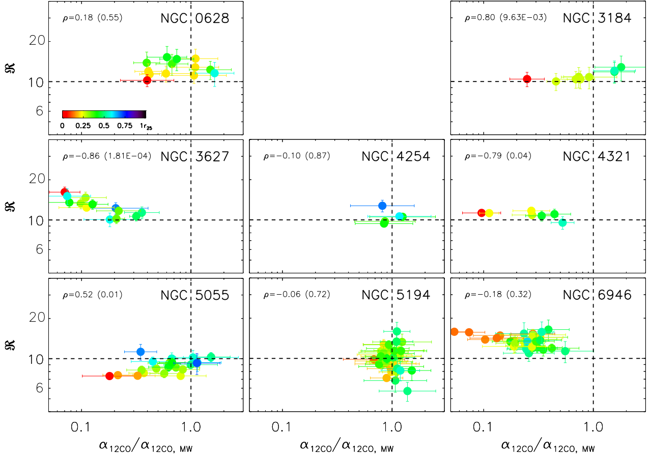
Figure 6. Correlation within galaxies of \mathfrak{R} and the conversion factor \alpha_{\text{CO}} , which is calibrated on dust emission. The trends are quite different from galaxy to galaxy. The colour code corresponds to distance to the galaxy centre and it is the same for all panels. The dashed lines are shown to guide the eye. We also indicate the Spearman's rank correlation coefficients and their significance in parenthesis.
