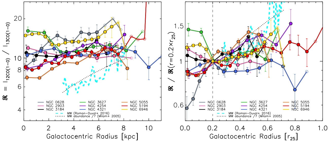
Figure 2. Left-hand panel: profiles of the ^{12}\text{CO}(1-0) -to- ^{13}\text{CO}(1-0) intensity ratio, \mathfrak{R} , as a function of galactocentric radius for each EMPIRE galaxy. Profile points for which the average ^{13}\text{CO}(1-0) or ^{12}\text{CO}(1-0) intensity within the ring is below 5\sigma are shown with open circles. We overlay for reference the Milky Way measurements of the \mathfrak{R} profile (dashed cyan curve) from Roman-Duval et al. (2016) and of the ^{12}\text{C}/^{13}\text{C} abundance gradient (black dotted line, divided by a factor of 7 for display) from Milam et al. (2005). Right-hand panel: same as the left-hand panel with radii normalized to r_{25} (x-axis) and the profiles normalized to their value at a radius of r = 0.2 r_{25} . We assume r_{25} = 11.5 kpc for the Milky Way (de Vaucouleurs & Pence 1978).
