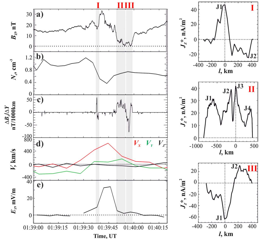
Figure 2. In the left column, a zoom of the pink shaded interval shown in Figure 1. From top to bottom are shown the (a) B_Z field and (b) electron density, N_e , from C3; the (c) \Delta B_X/\Delta Y_{C3-C4} ; (d) three components of proton bulk velocity; and (e) the dawn-dusk electric field, E_Y , from C4. Three intervals (I–III) of strong \Delta B_X/\Delta Y_{C3-C4} variations are shaded in gray. In the right part of the figure the spatial profiles of the electric current density J_Z^* estimated for intervals I–III are shown.
