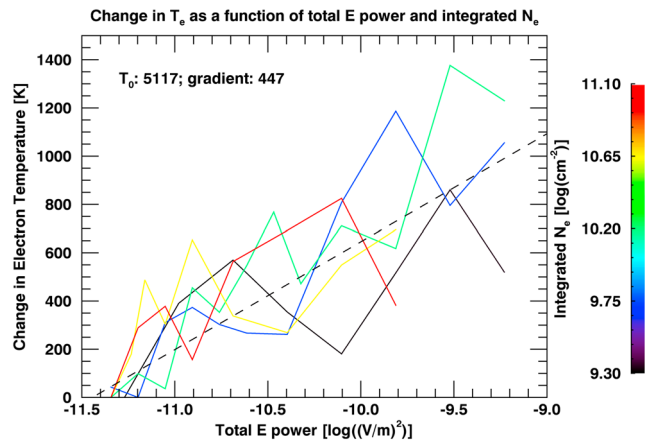
Figure 3. Horizontal cuts through Figure 2a, showing T_e as a function of total electric field wave power, for specific integrated electron densities. T_e have been shifted such that the vertical axis shows the change in T_e , from the coldest value measured for each line. The dashed black line is a fit to all data points. Note that Figure 4a can be used to obtain an approximate conversion between integrated electron density and altitude.
