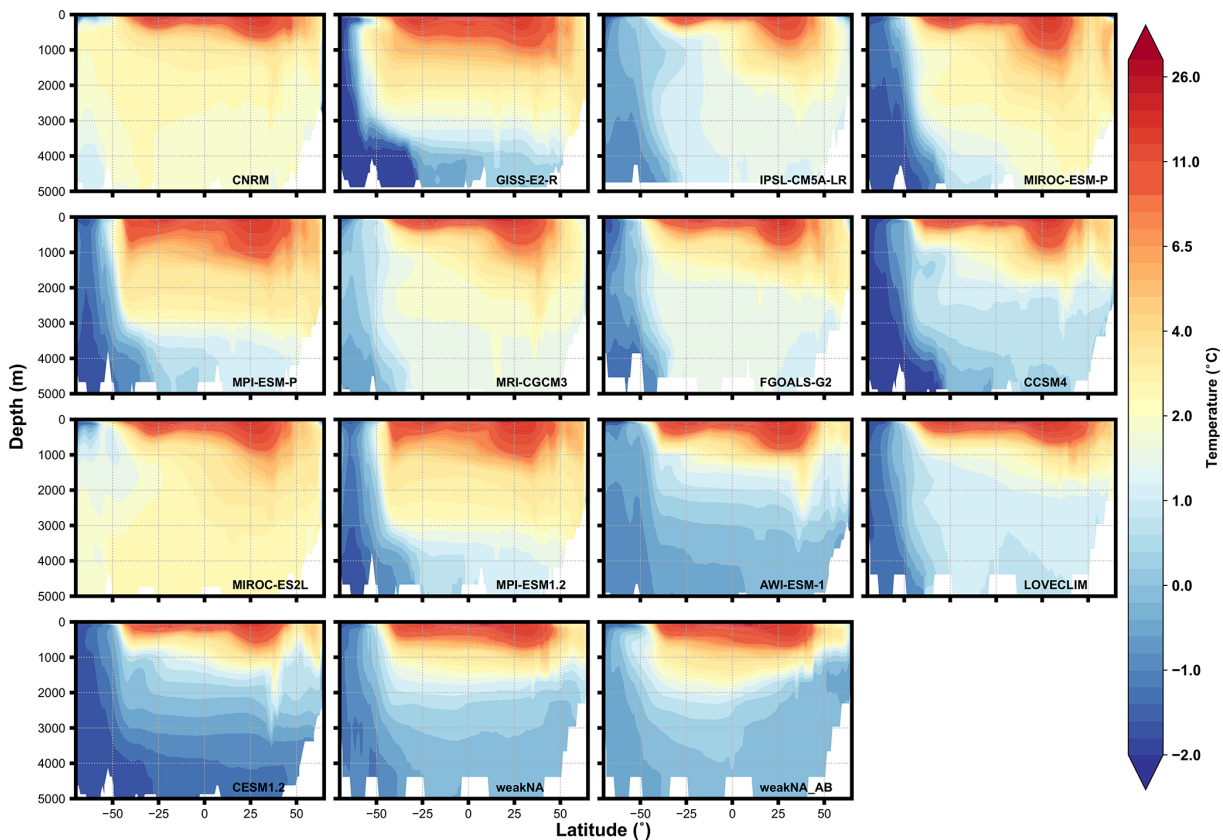
Figure 6. Zonally averaged oceanic potential temperatures (°C) in the Atlantic basin for PMIP3, PMIP4 and LOVECLIM simulations.
