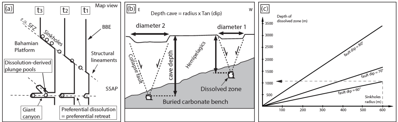
Figure 7: (a) Conceptual sketch showing how the BBE erosional retreat likely exploits the structural lineaments related to the TOC transition in to reach its present-day geomorphological configuration. (b) Conceptual sketch showing the relationships between the depth of the dissolved rock volume (cave) and the radius of outer and inner sinkholes (c) Quantitative estimation of the cave depth in the case of sinkhole 1 (radius = 600 m).
