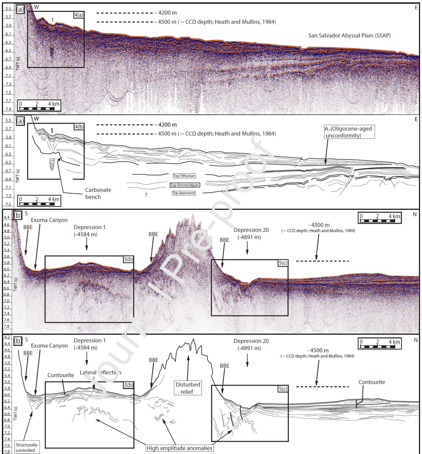
Figure 3: 2D seismic lines Two-Way Travel Time (TWT) of the study area and associated interpretations: (a) N080 trending line respectively showing from the west (left) to the east (right) the BBE, the depression #1 and the San Salvador Abyssal Plain. The top basement, the top Kimmeridgian, the top Tithonian, the A u unconformity and the post Miocene deposits have been interpreted. (b) N170 trending line respectively showing from the south (left) to the north (right), the Exuma Canyon, the depression #1, the BBE, the depression #2 and the layered northern contouritic deposits.
