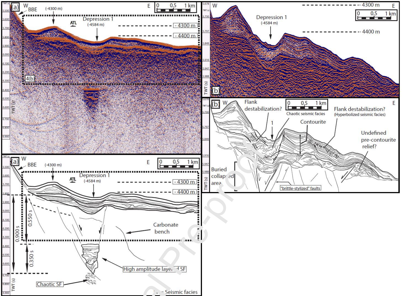
Figure 4: (a) Details of Figure 3(c) showing the depression #1 with its underlying seismic anomaly. (b) Details of the contouritic drift architecture overlying the depression #1 and exhibiting several stages of collapse by brittle faulting. The vertical exaggeration in (b) is around 2.5.
