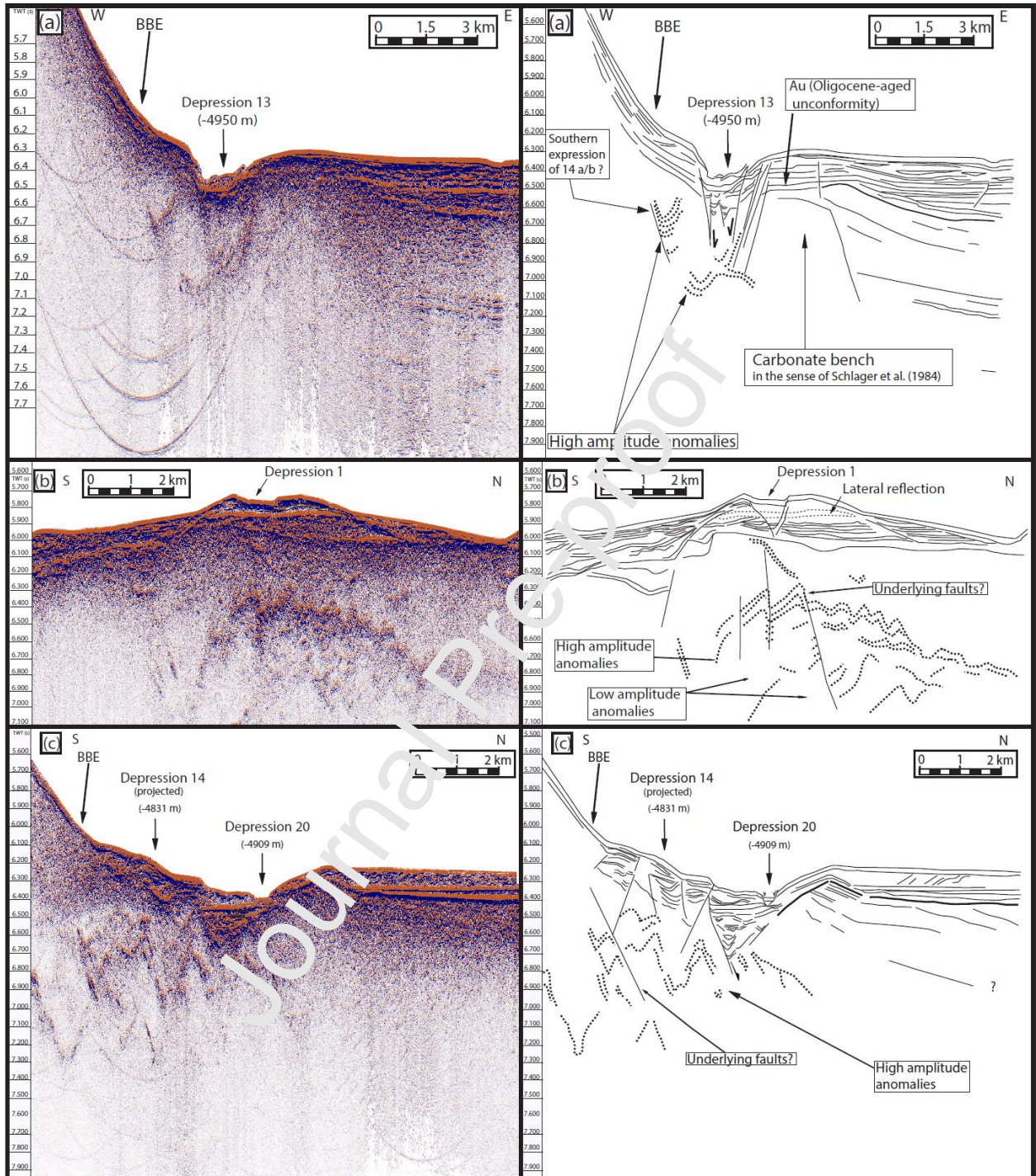
Figure 5: (a) N080-trending 2D seismic line and its interpretation crossing the depression #13 in the BBE curvature area. (b) Details of the Figure 3(b), 2D seismic line and its interpretation showing the depression #1 with its related underlying seismic anomaly. (c) Details of the Figure 3(b), 2D seismic line and its interpretation showing the depression #20 near the BBE curvature area. The interpretation shows the normal faults probably related to the depression formation. The aforementioned seismic lines are also reported in Figures 1 and 2.
